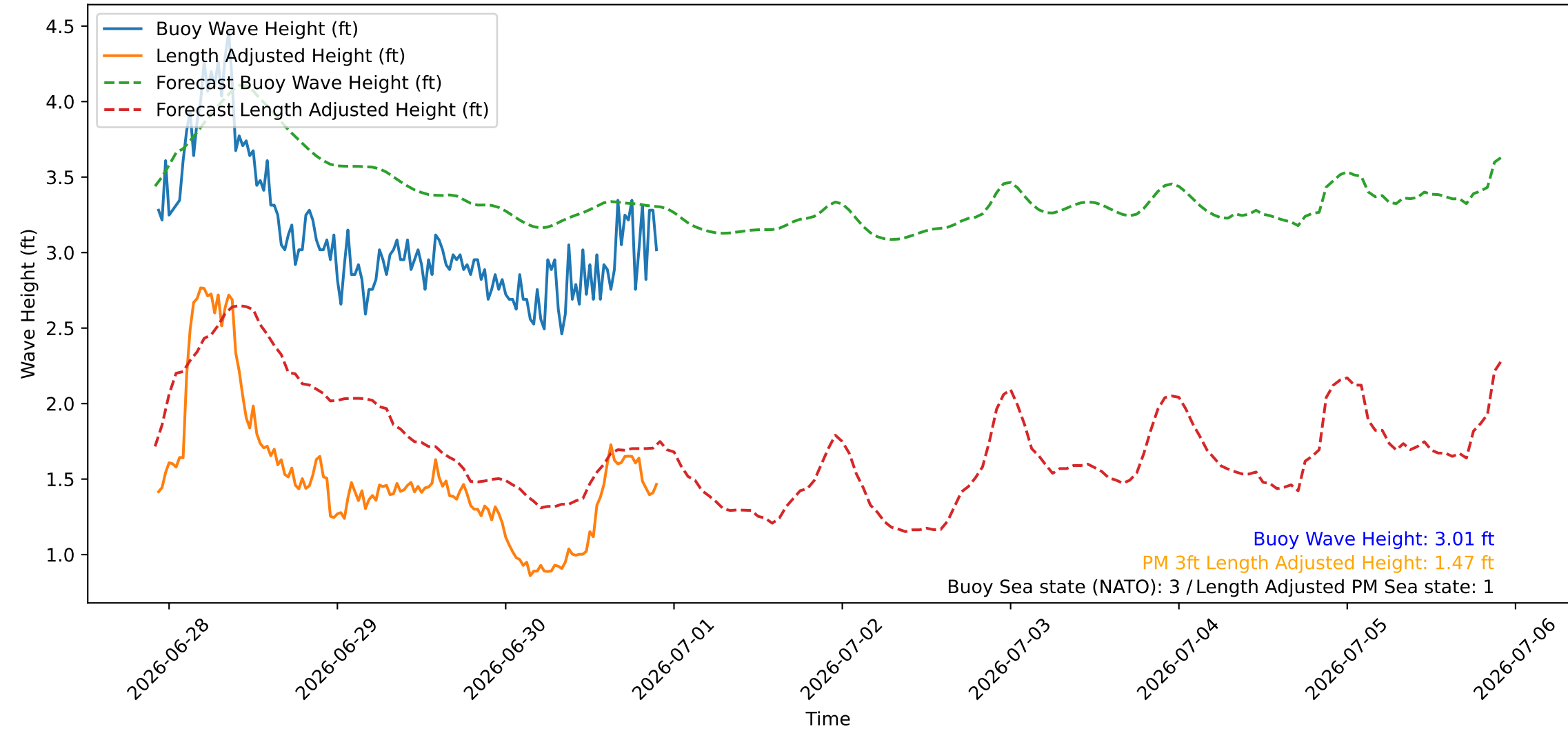
Wave Heights over Time for Red Beach at 2026-06-30 22:20:48
