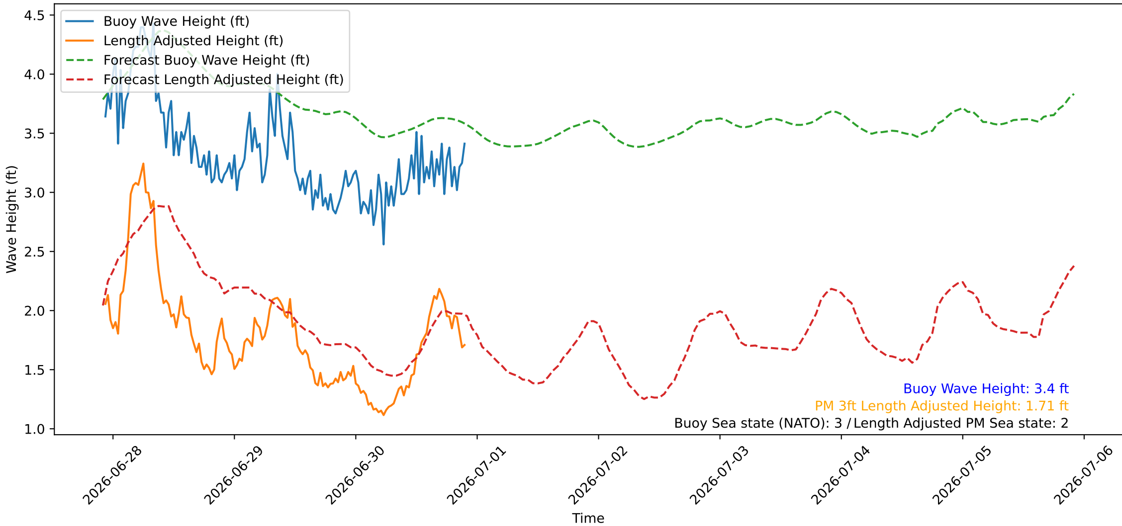
Wave Heights over Time for Oceanside Harbor at 2026-06-30 22:20:27
