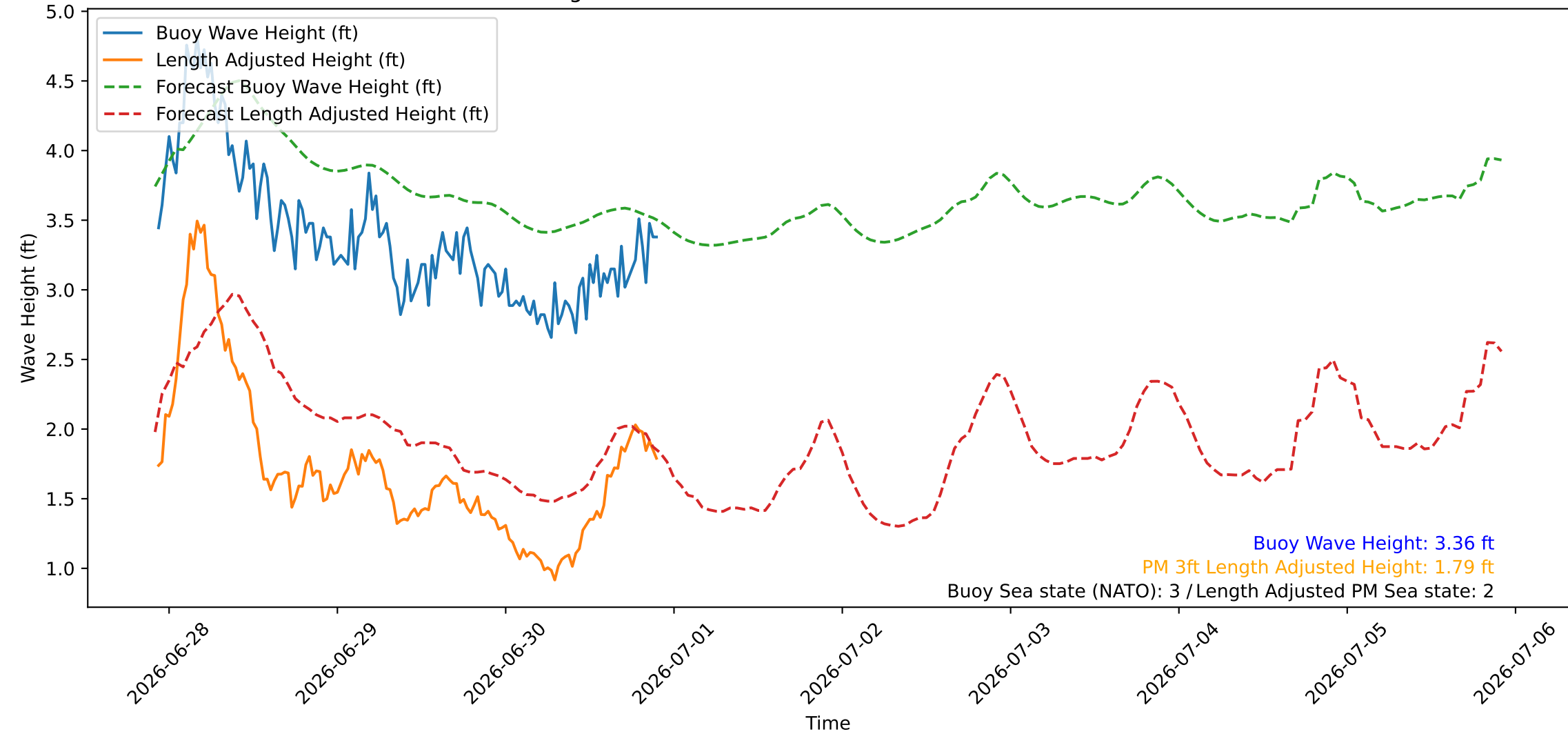
Wave Heights over Time for Green Beach at 2026-06-30 22:21:11
