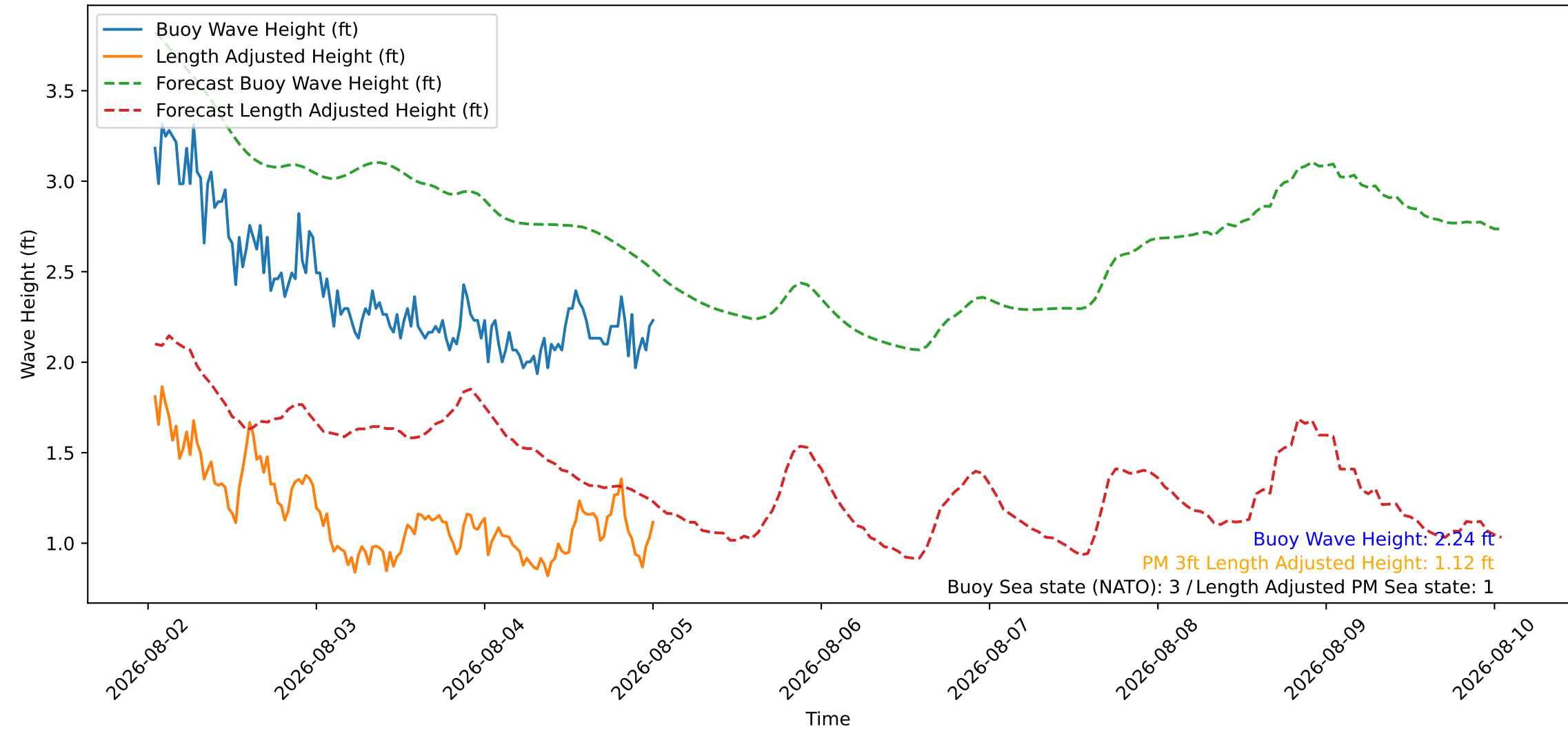
Wave Heights over Time for Green Beach at 2026-08-05 00:51:09
