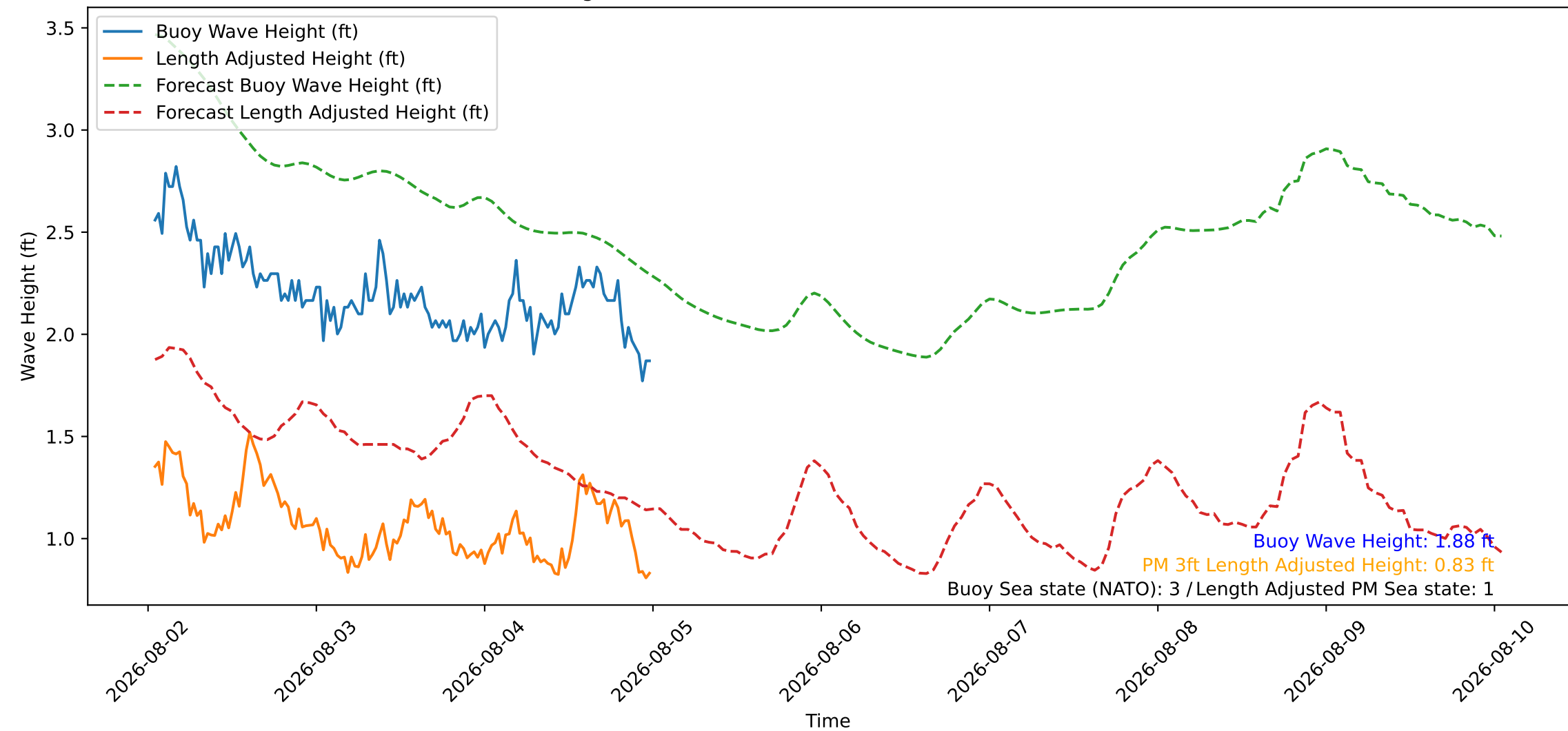
Wave Heights over Time for Red Beach at 2026-08-05 00:50:47
