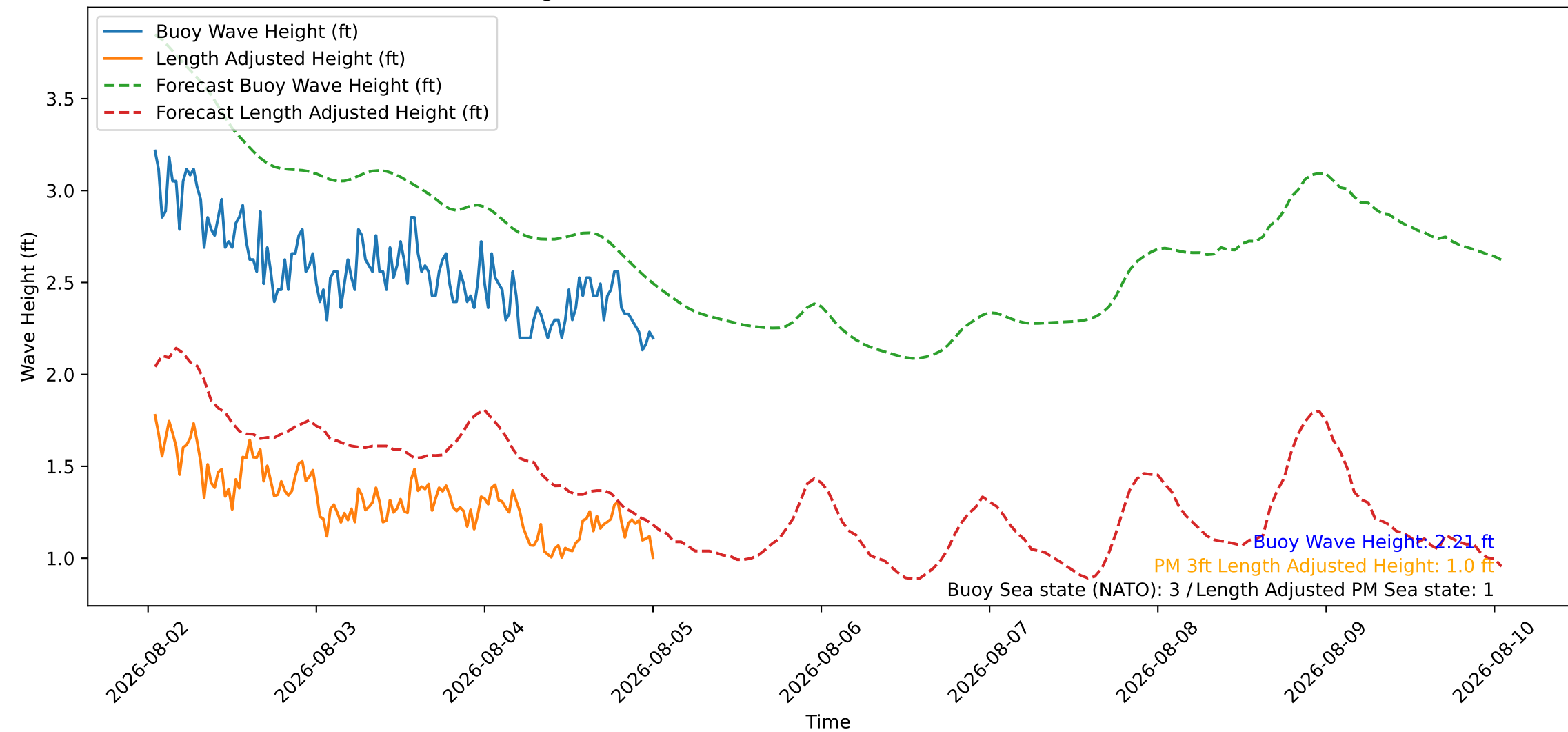
Wave Heights over Time for Oceanside Harbor at 2026-08-05 00:50:26
