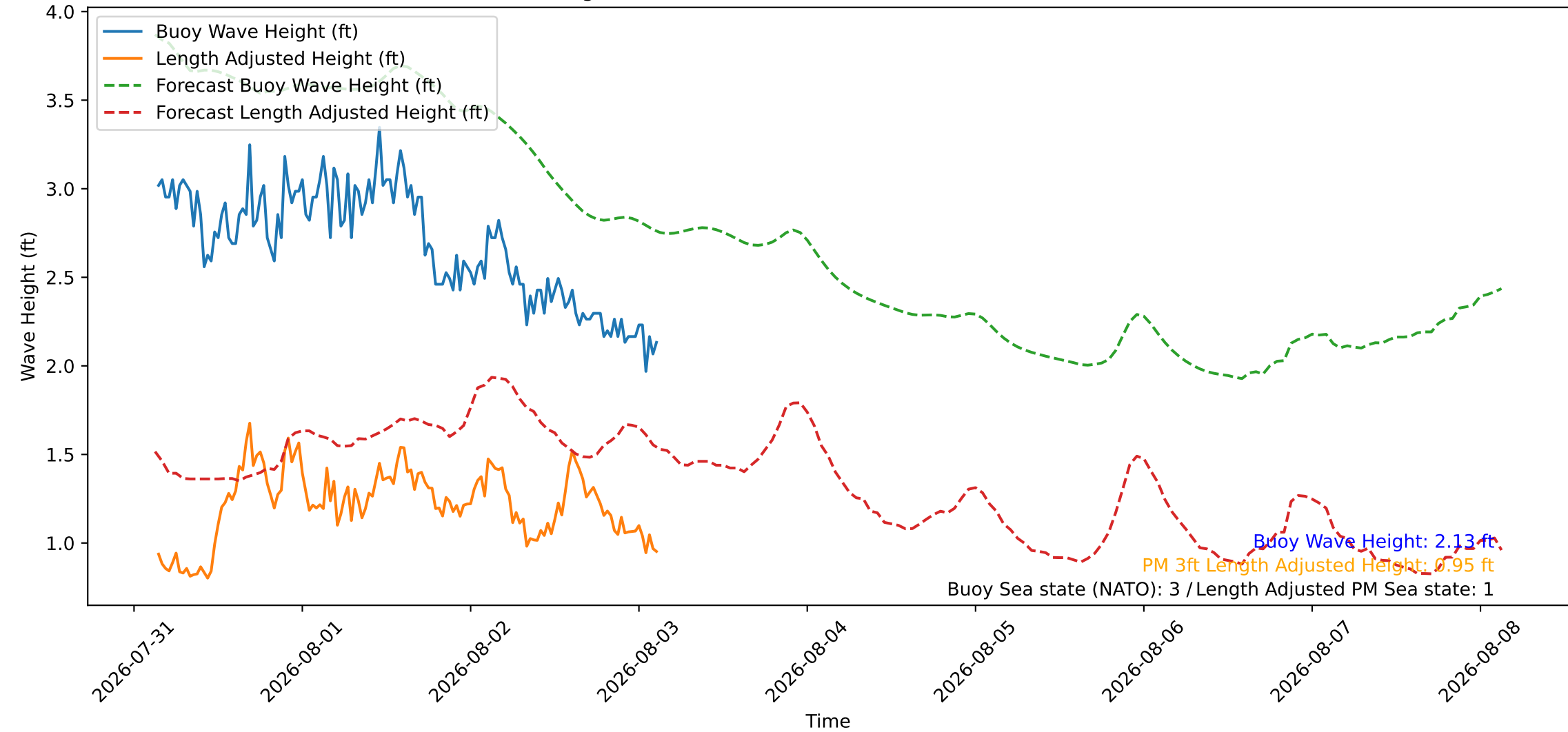
Wave Heights over Time for Red Beach at 2026-08-03 03:20:46
