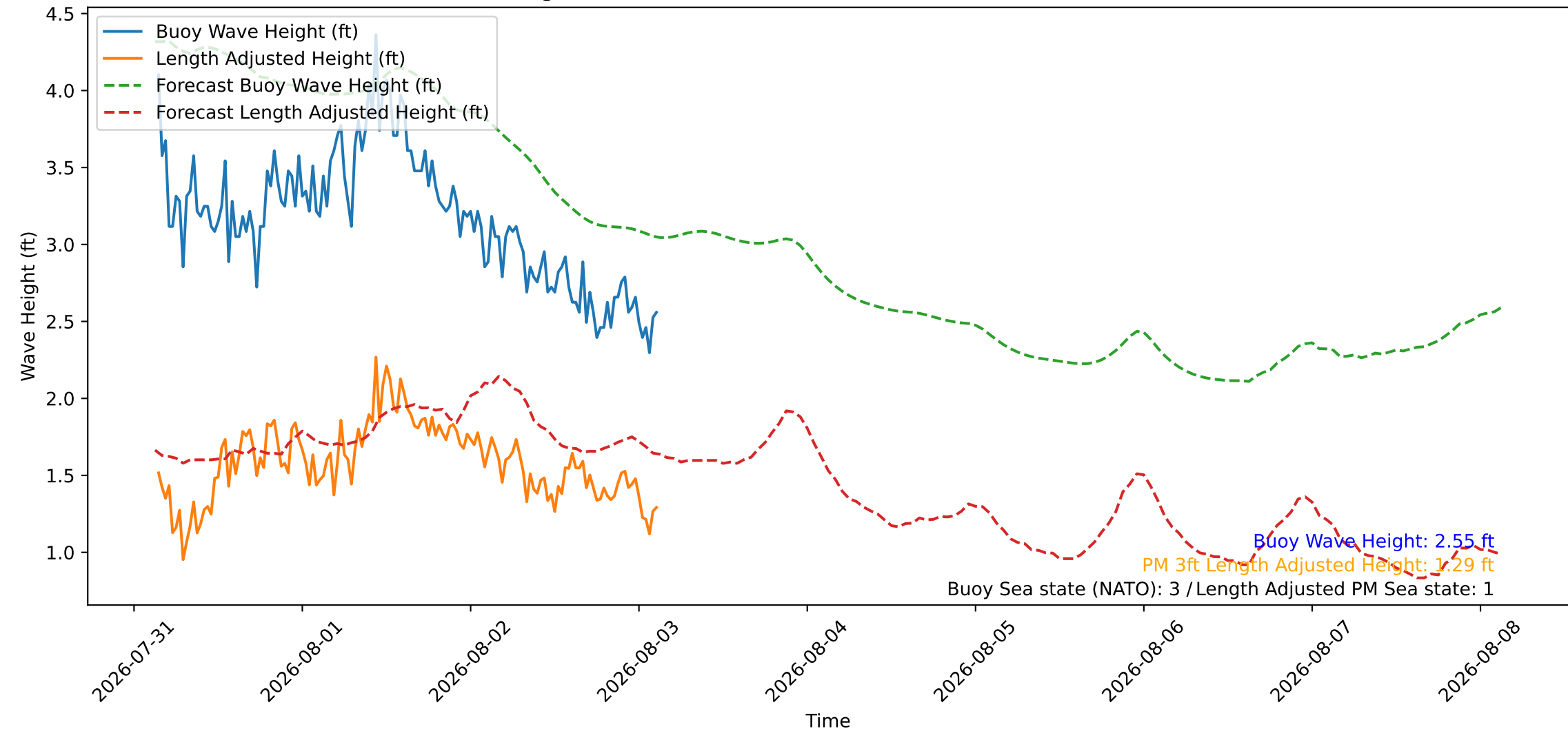
Wave Heights over Time for Oceanside Harbor at 2026-08-03 03:20:25
