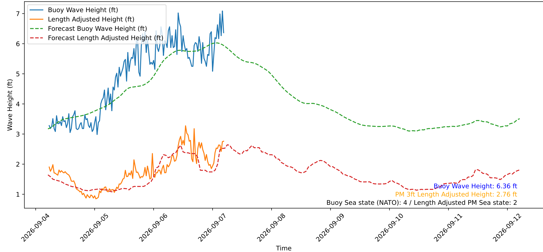
Wave Heights over Time for Oceanside Harbor at 2026-09-07 05:20:30
