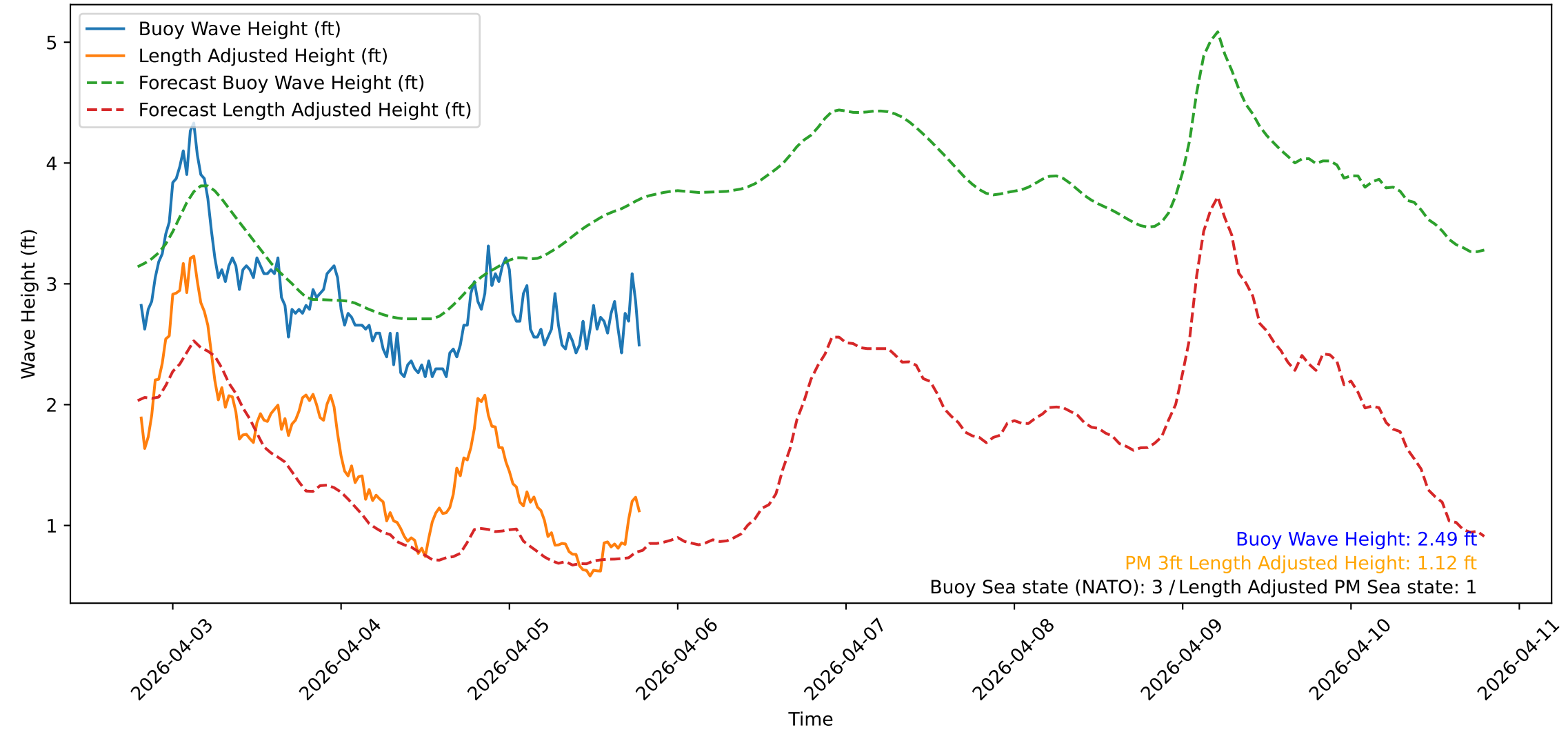
Wave Heights over Time for Green Beach at 2026-04-05 19:21:18
