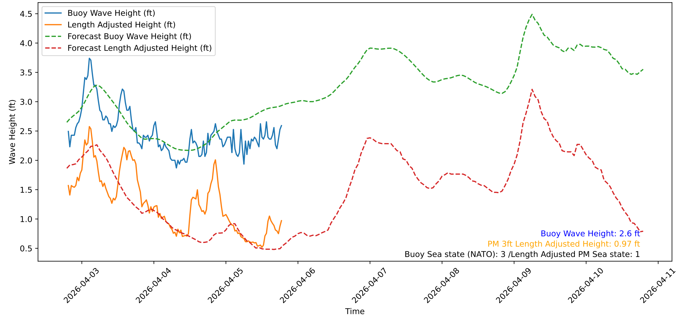
Wave Heights over Time for Red Beach at 2026-04-05 19:20:52
