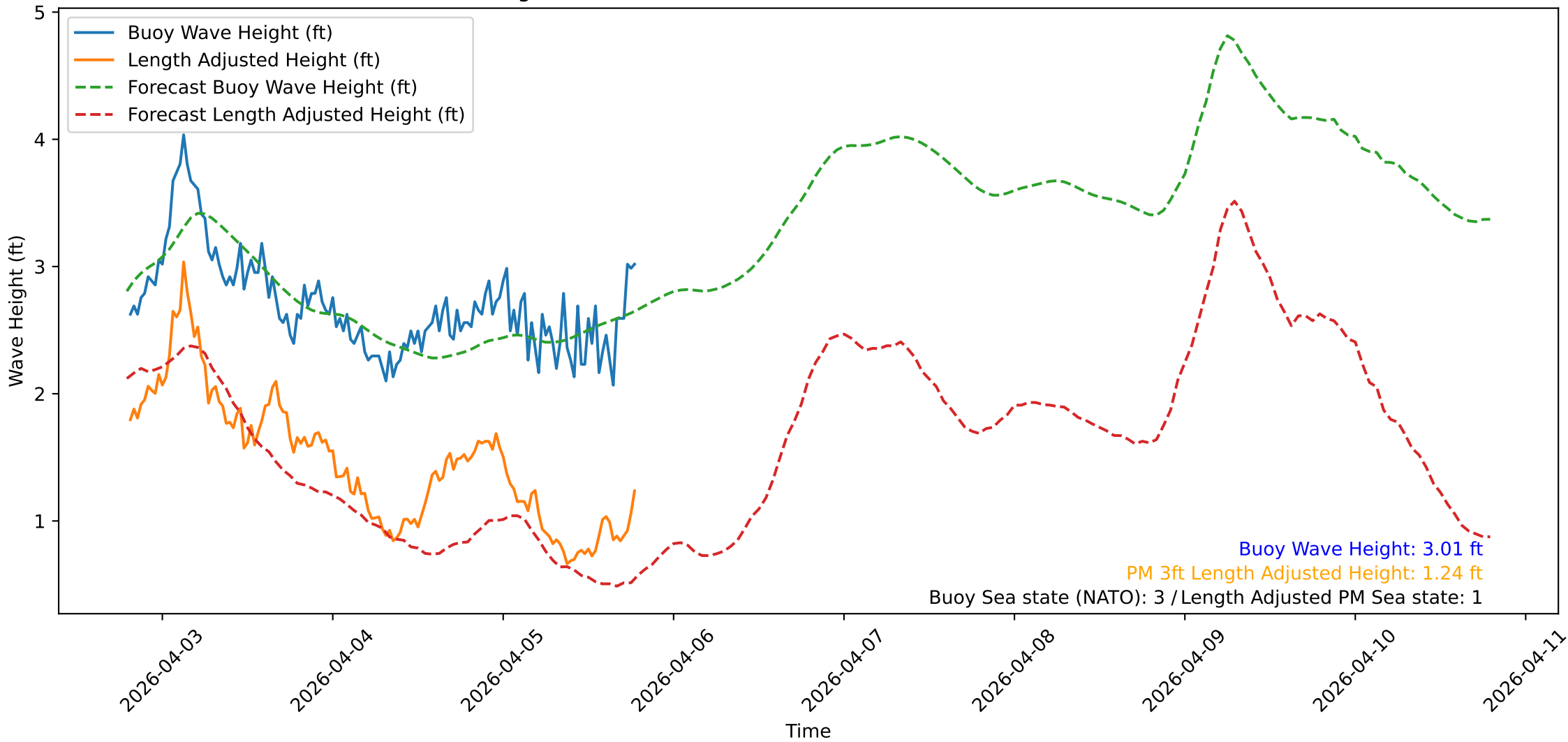
Wave Heights over Time for Oceanside Harbor at 2026-04-05 19:20:33
