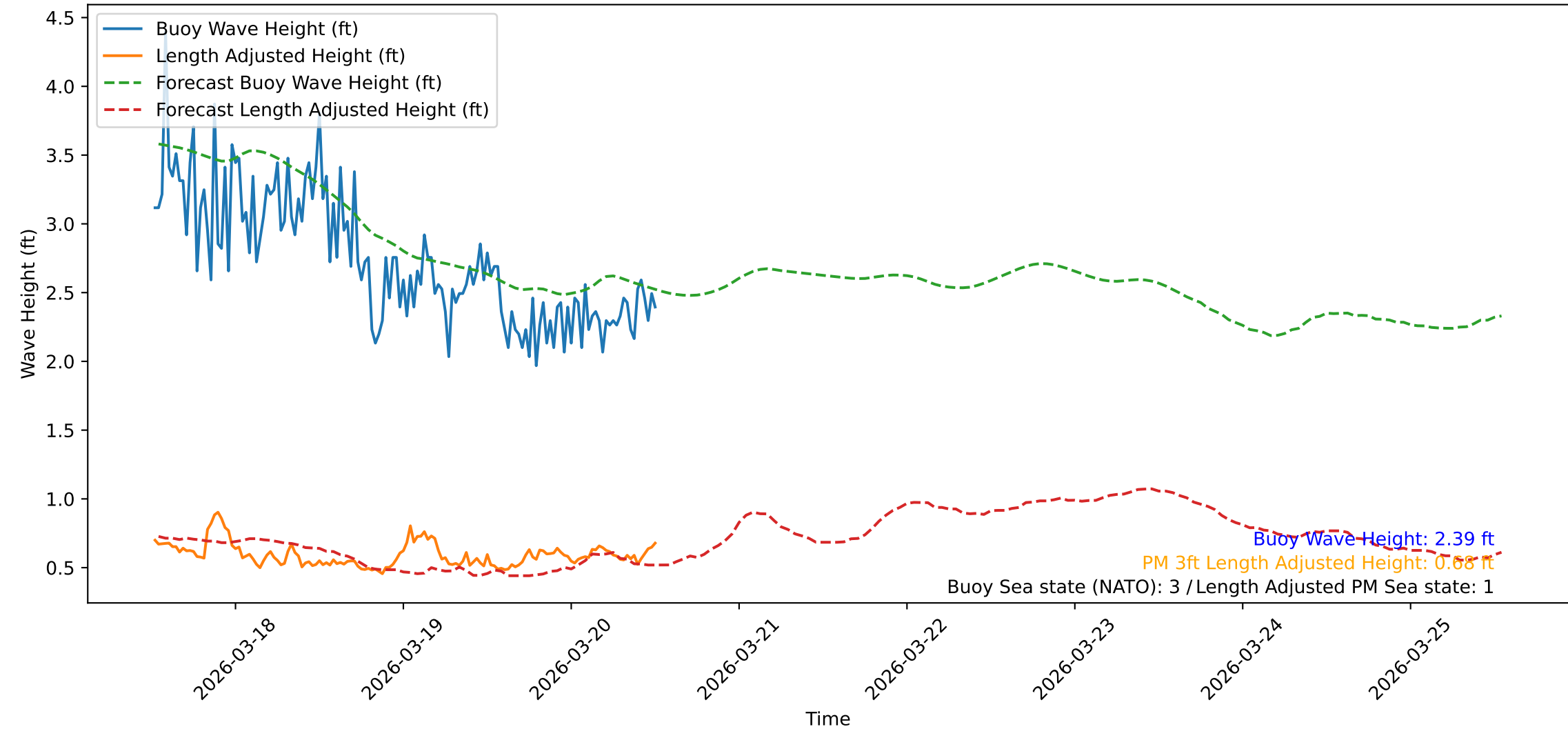
Wave Heights over Time for Oceanside Harbor at 2026-03-20 12:40:32
