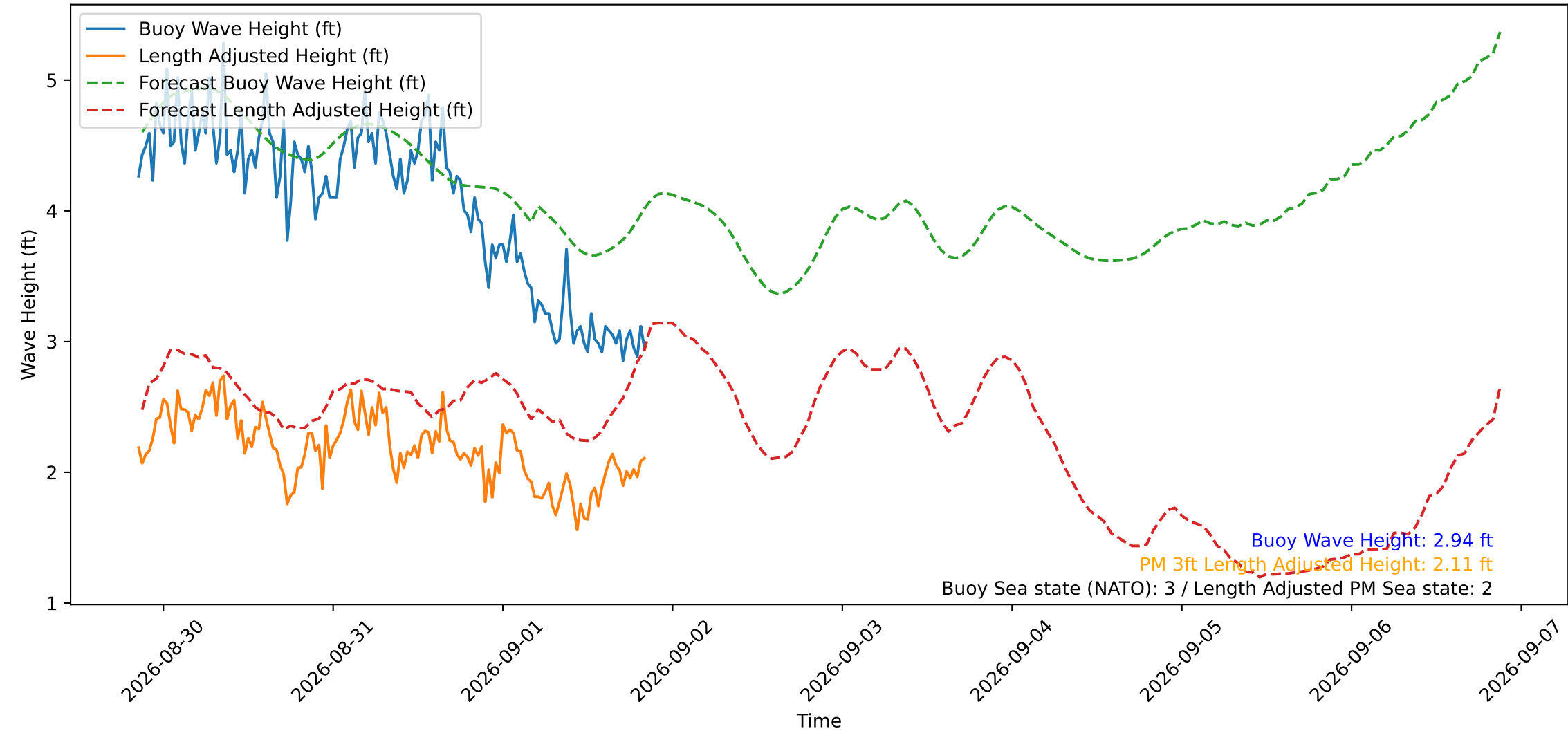
Wave Heights over Time for Oceanside Harbor at 2026-09-01 20:40:29
