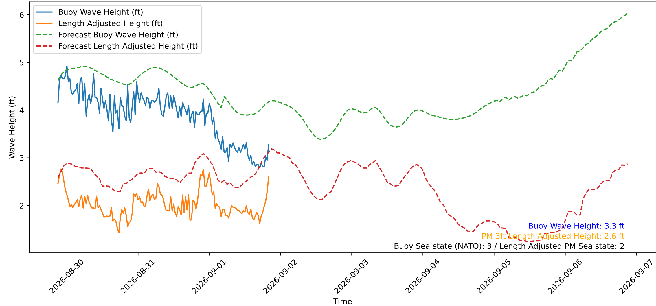
Wave Heights over Time for Green Beach at 2026-09-01 20:41:12
