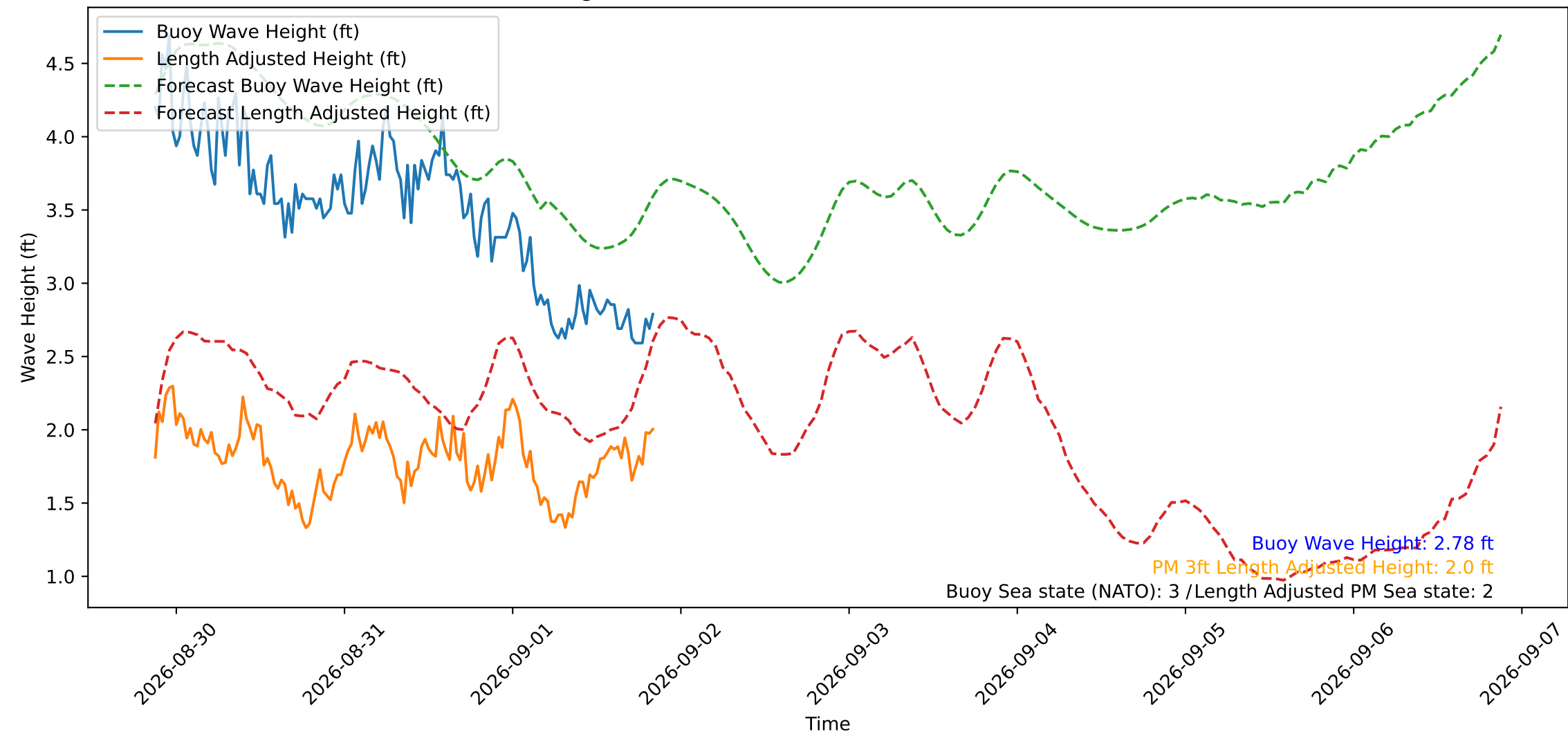
Wave Heights over Time for Red Beach at 2026-09-01 20:40:49
