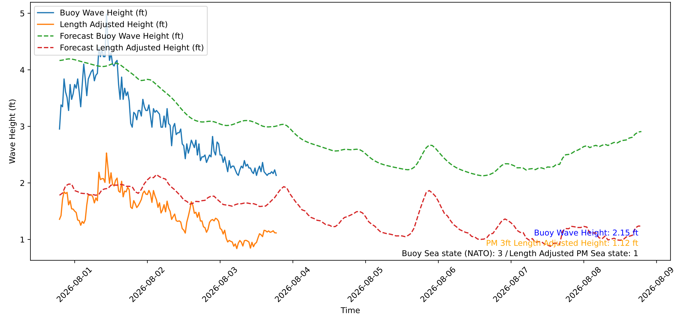
Wave Heights over Time for Green Beach at 2026-08-03 19:11:08
