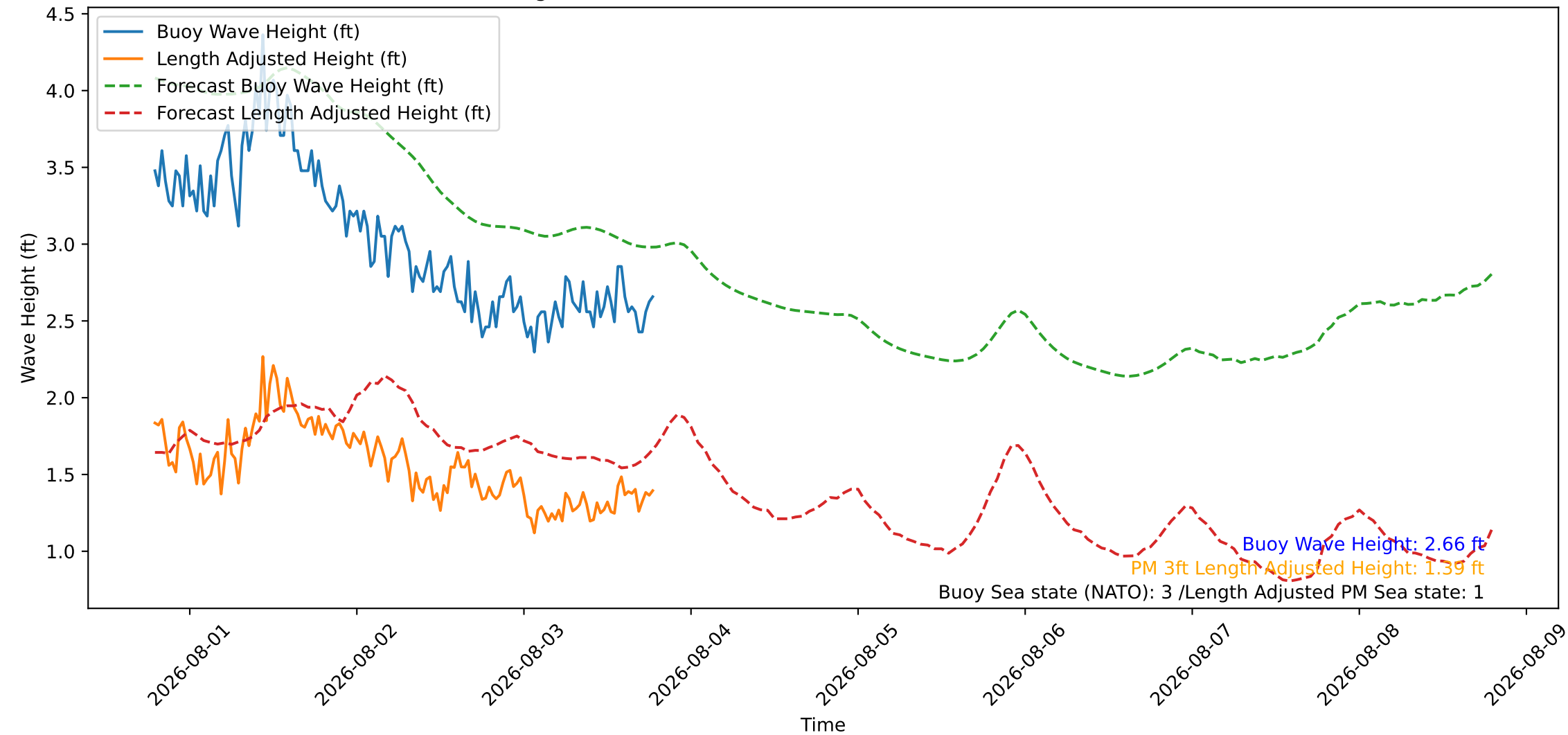
Wave Heights over Time for Oceanside Harbor at 2026-08-03 19:10:26
