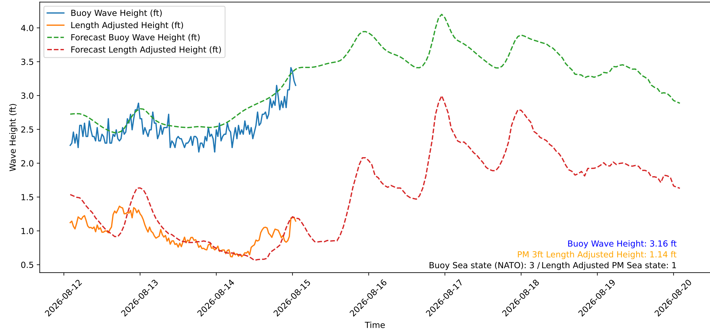
Wave Heights over Time for Red Beach at 2026-08-15 01:40:46
