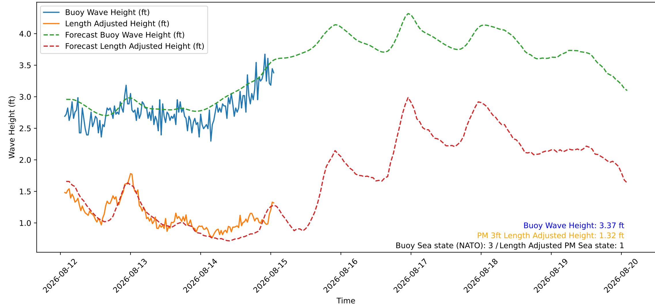
Wave Heights over Time for Oceanside Harbor at 2026-08-15 01:40:26
