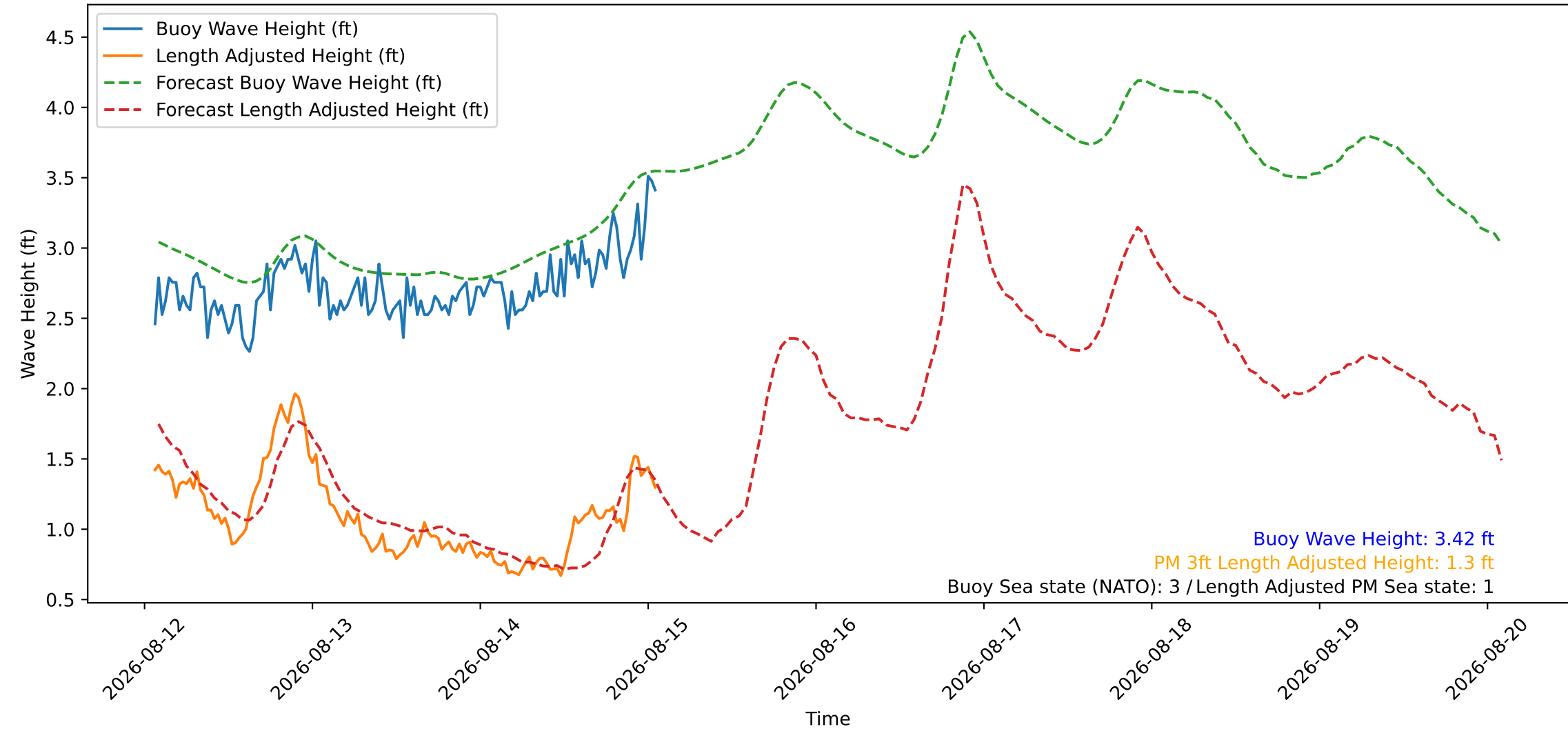
Wave Heights over Time for Green Beach at 2026-08-15 01:41:09
