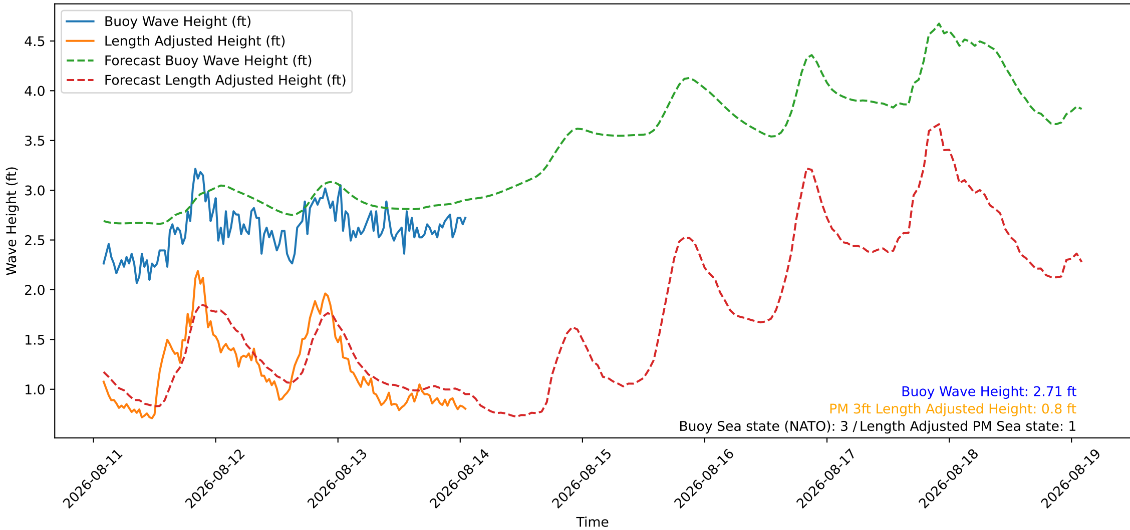
Wave Heights over Time for Green Beach at 2026-08-14 02:01:09
