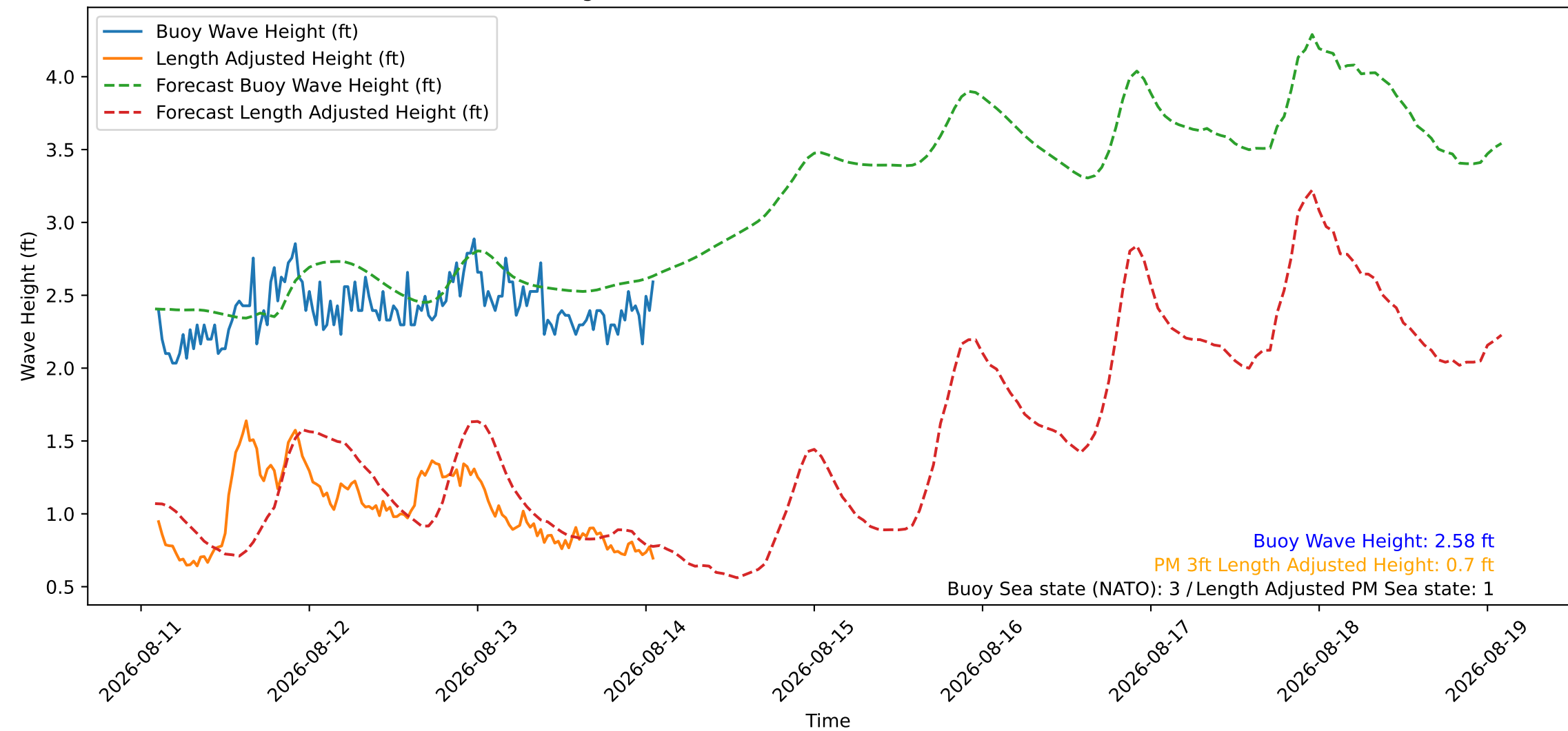
Wave Heights over Time for Red Beach at 2026-08-14 02:00:46
