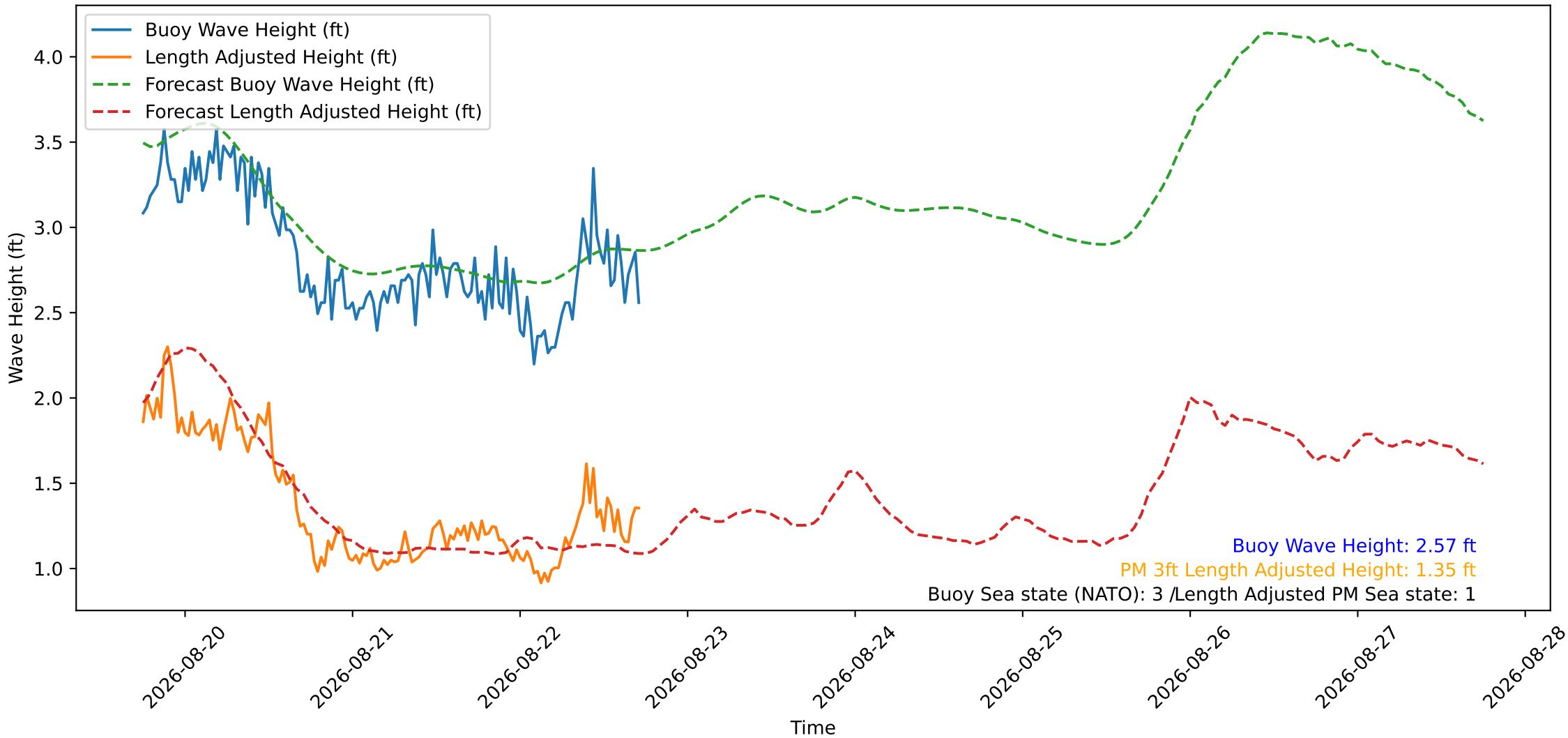
Wave Heights over Time for Oceanside Harbor at 2026-08-22 17:50:30
