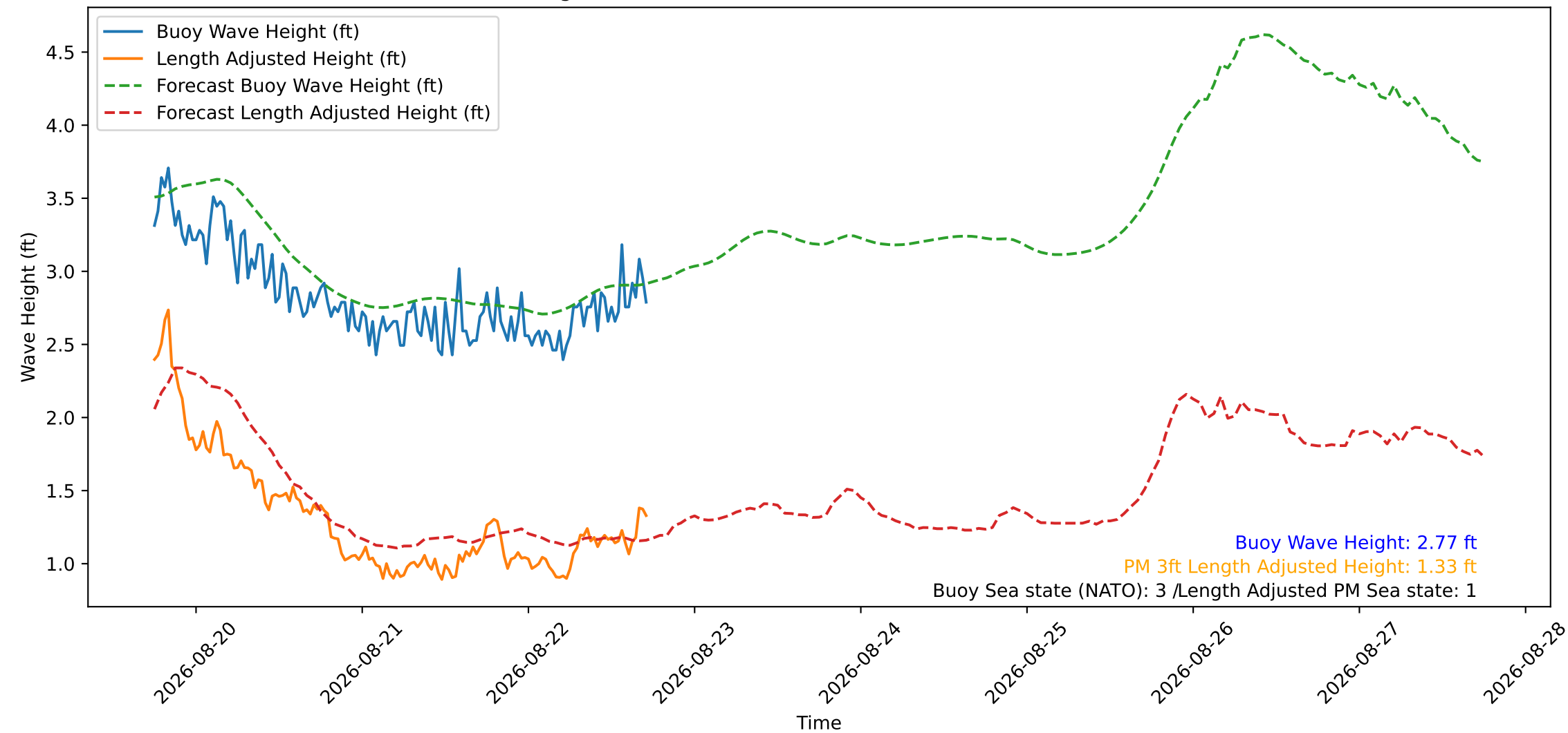
Wave Heights over Time for Green Beach at 2026-08-22 17:51:15
