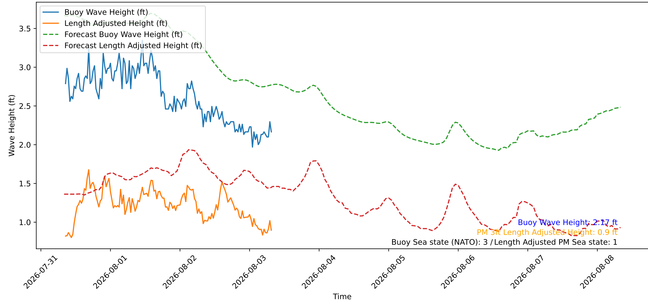
Wave Heights over Time for Red Beach at 2026-08-03 08:20:47
