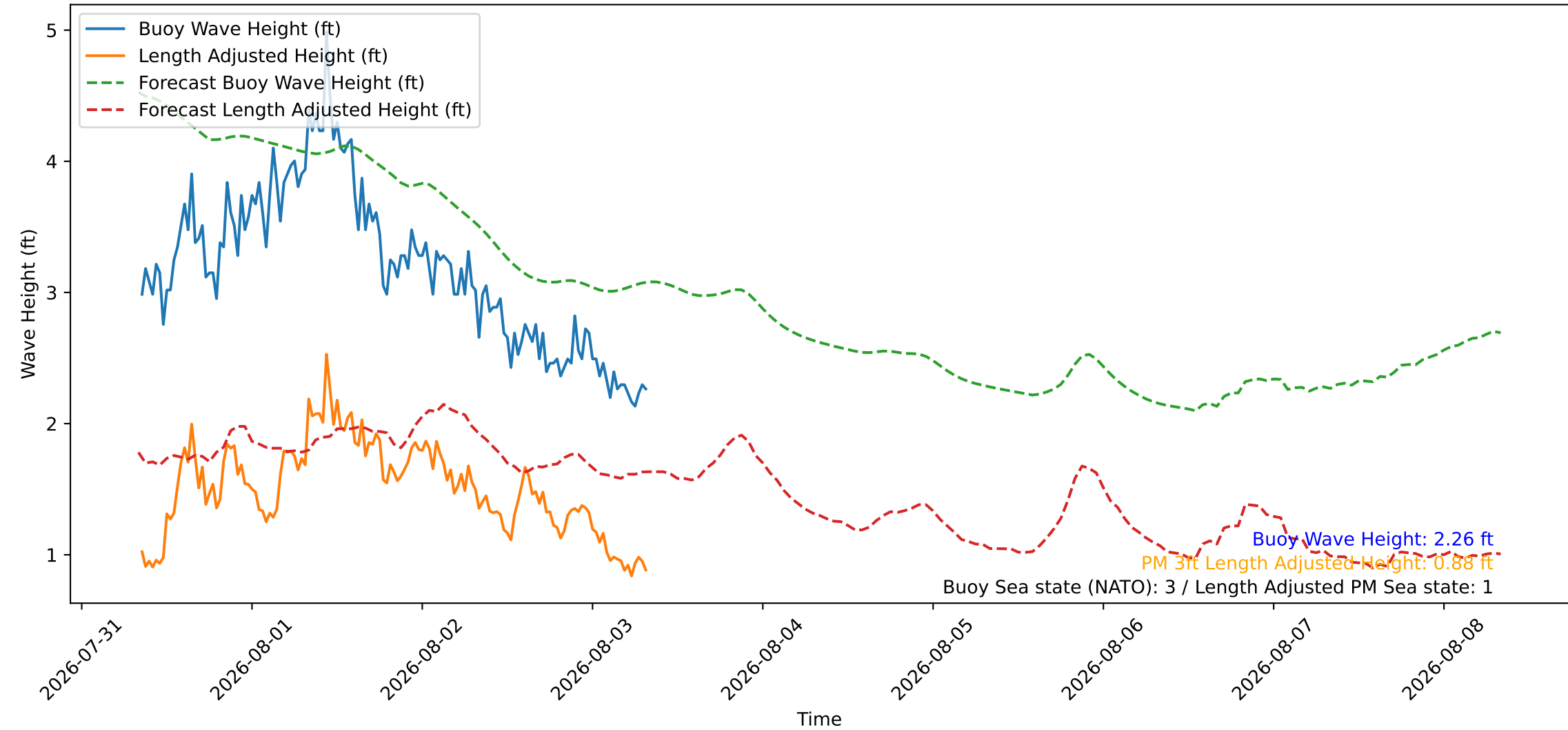
Wave Heights over Time for Green Beach at 2026-08-03 08:21:09
