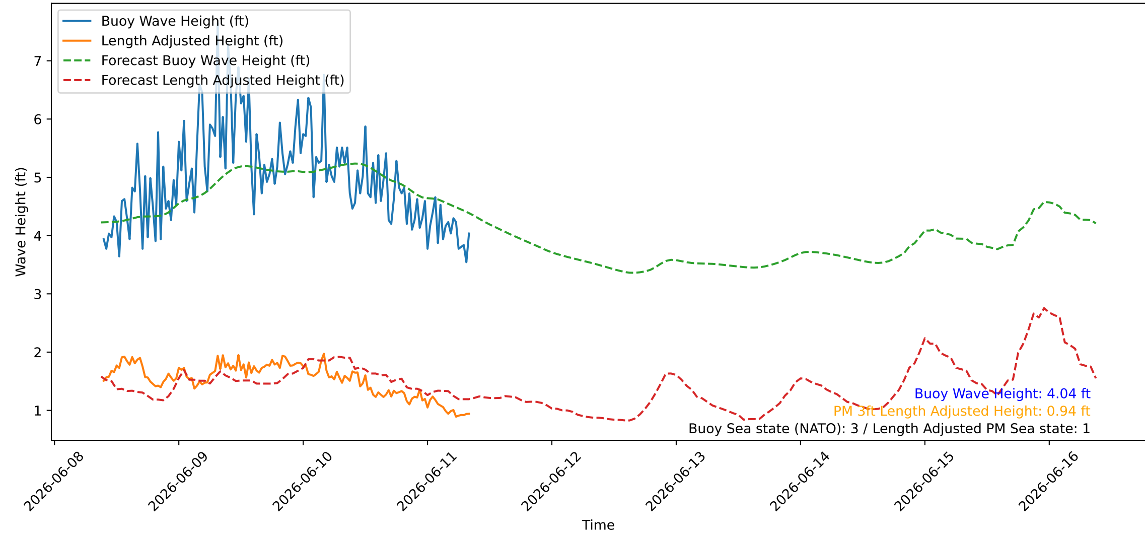
Wave Heights over Time for Red Beach at 2026-06-11 09:20:47
