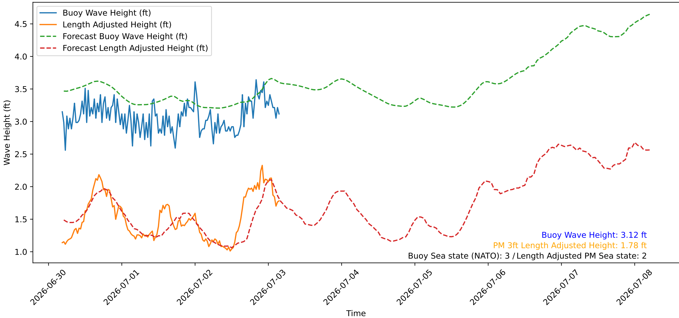
Wave Heights over Time for Oceanside Harbor at 2026-07-03 04:30:26
