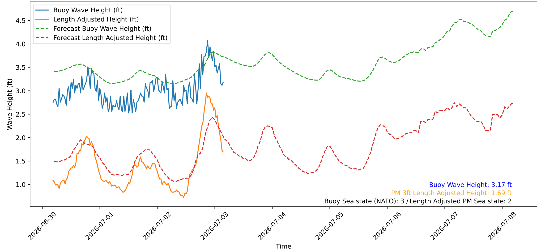
Wave Heights over Time for Green Beach at 2026-07-03 04:31:08
