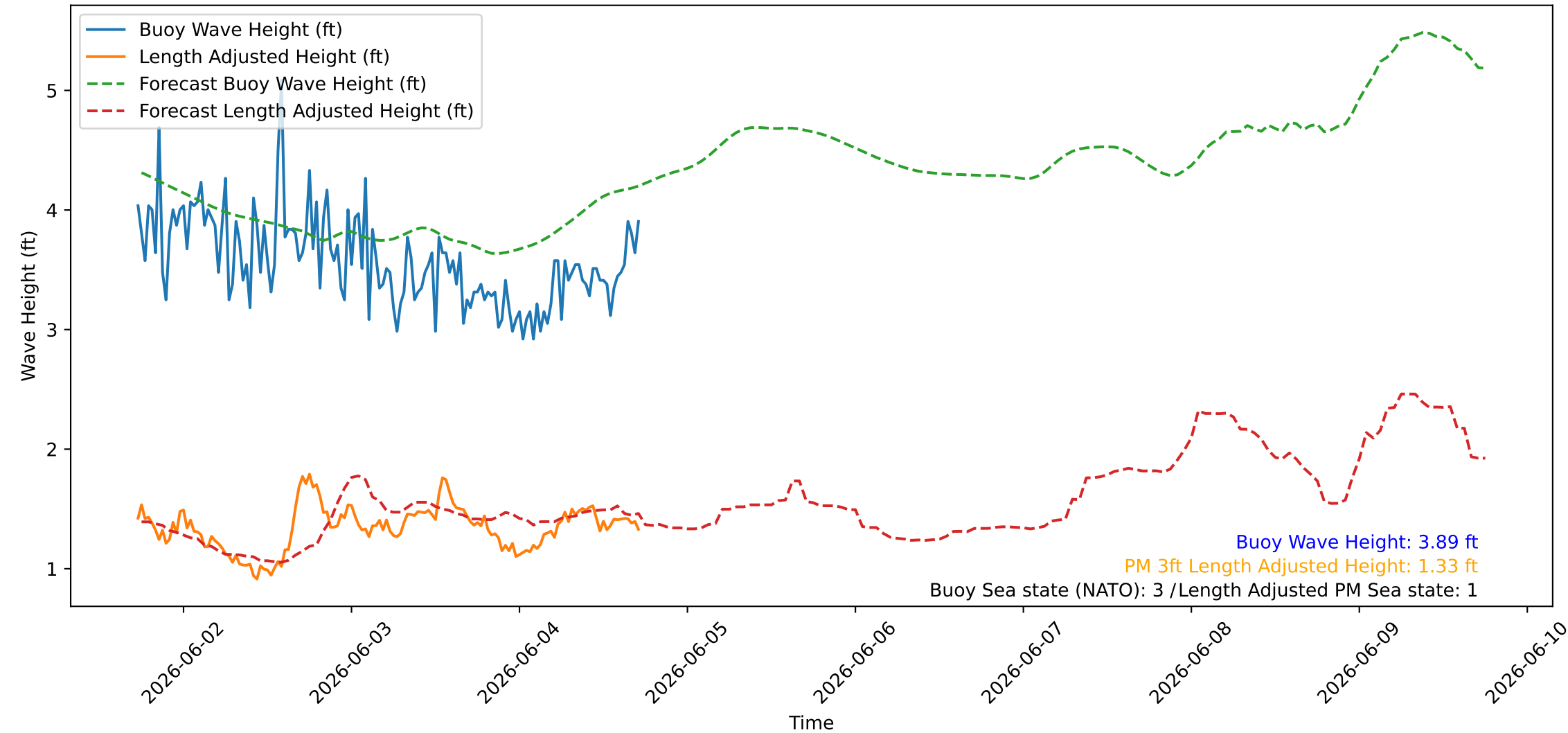
Wave Heights over Time for Oceanside Harbor at 2026-06-04 17:40:26
