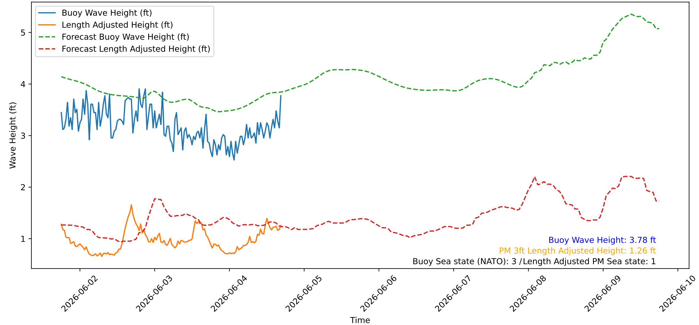
Wave Heights over Time for Red Beach at 2026-06-04 17:40:45
