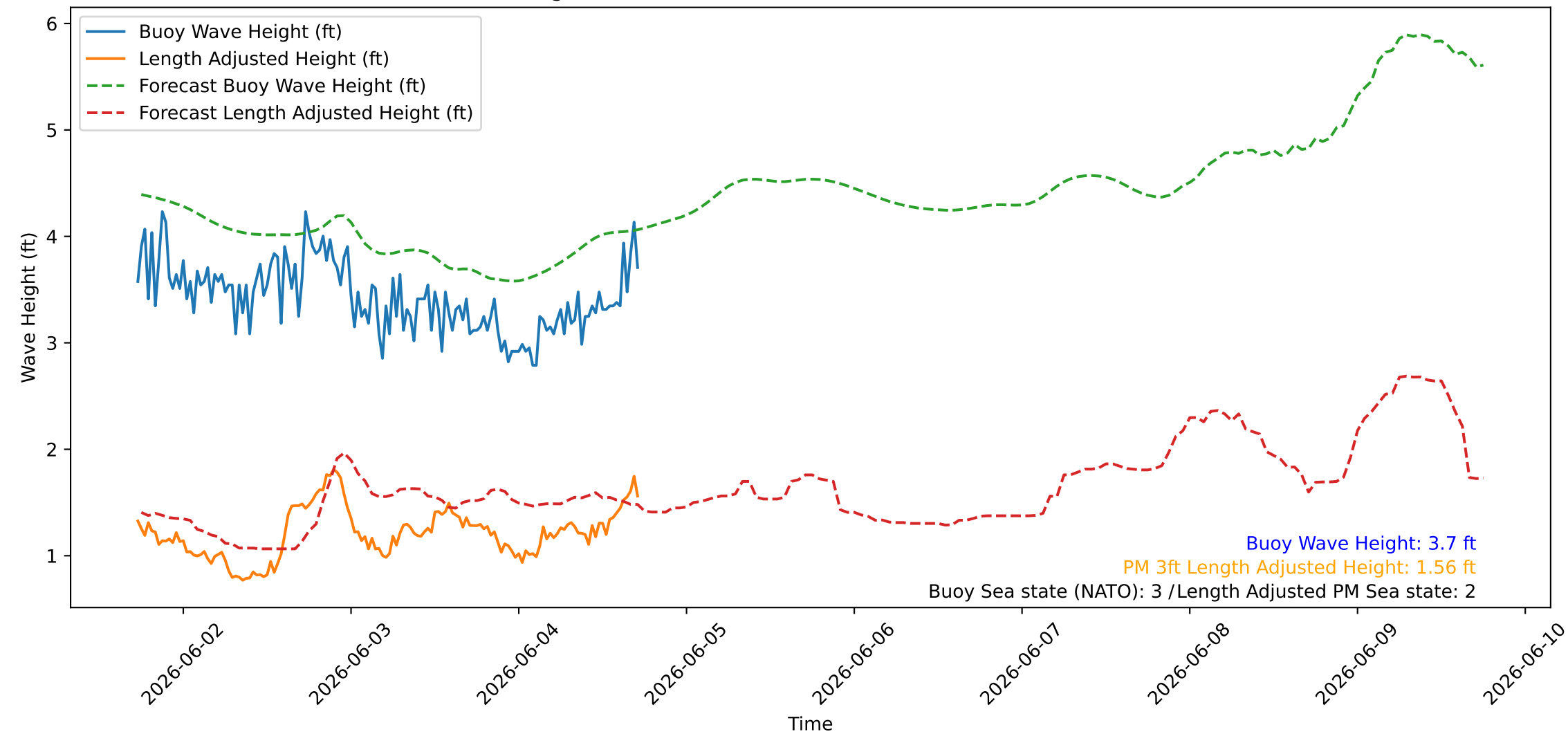
Wave Heights over Time for Green Beach at 2026-06-04 17:41:08
