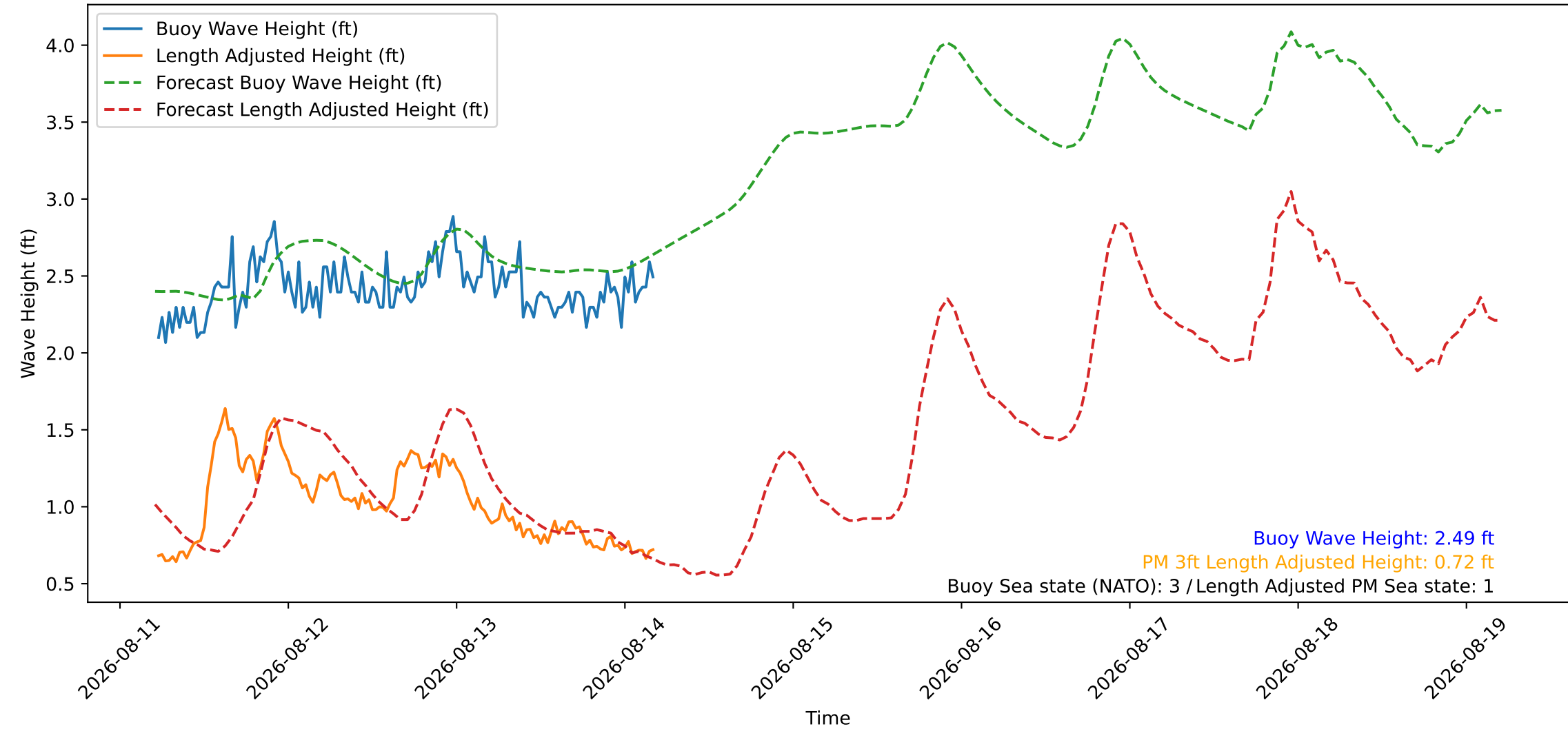
Wave Heights over Time for Red Beach at 2026-08-14 05:00:46
