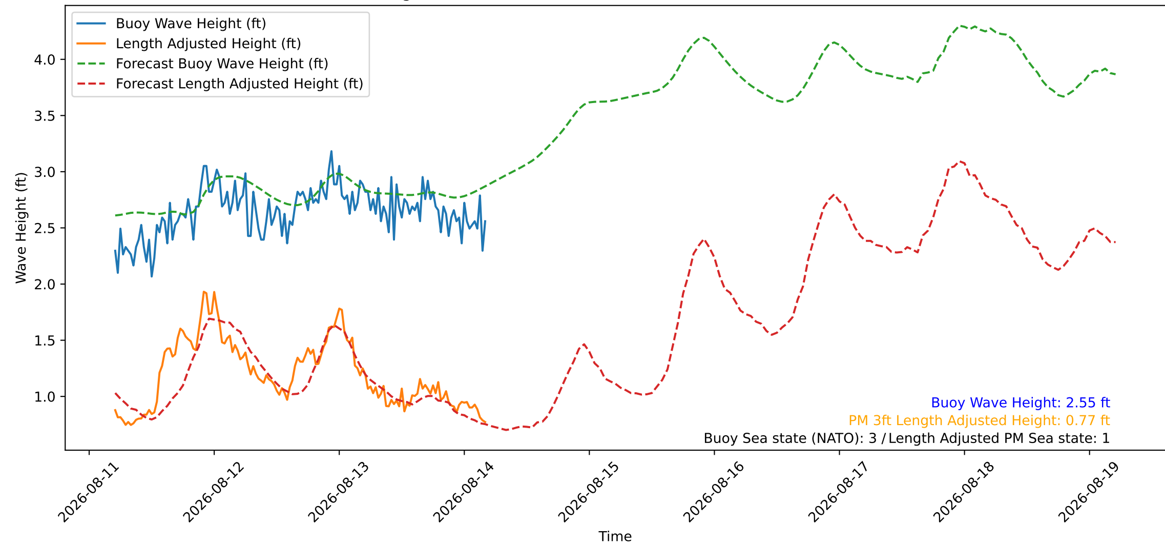
Wave Heights over Time for Oceanside Harbor at 2026-08-14 05:00:27
