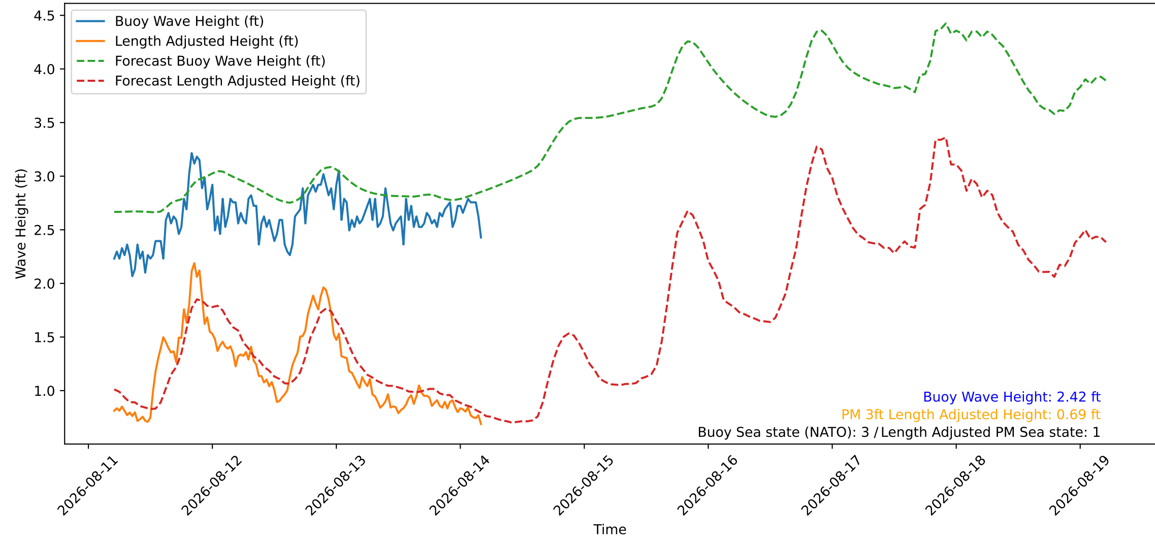
Wave Heights over Time for Green Beach at 2026-08-14 05:01:09
