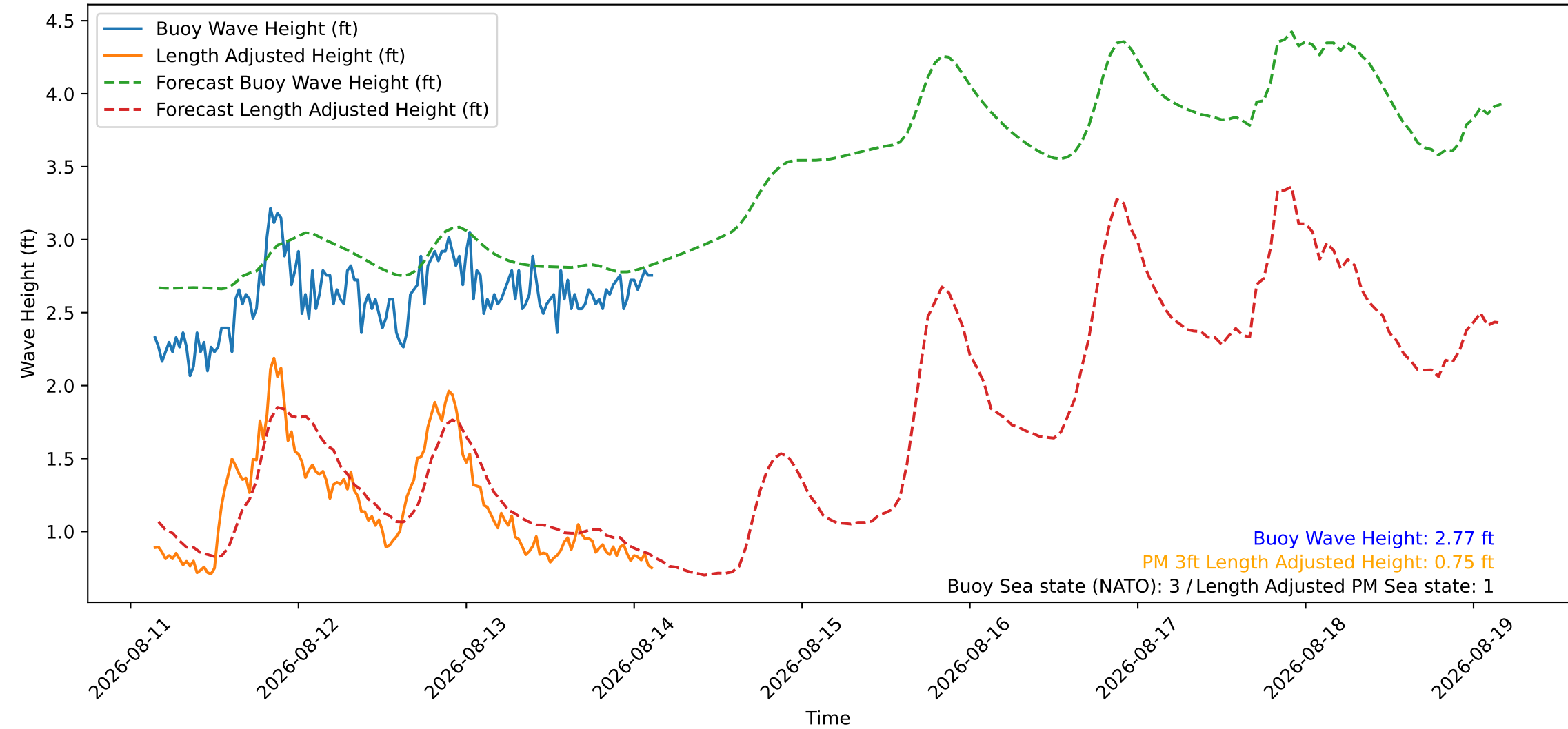
Wave Heights over Time for Green Beach at 2026-08-14 03:31:09
