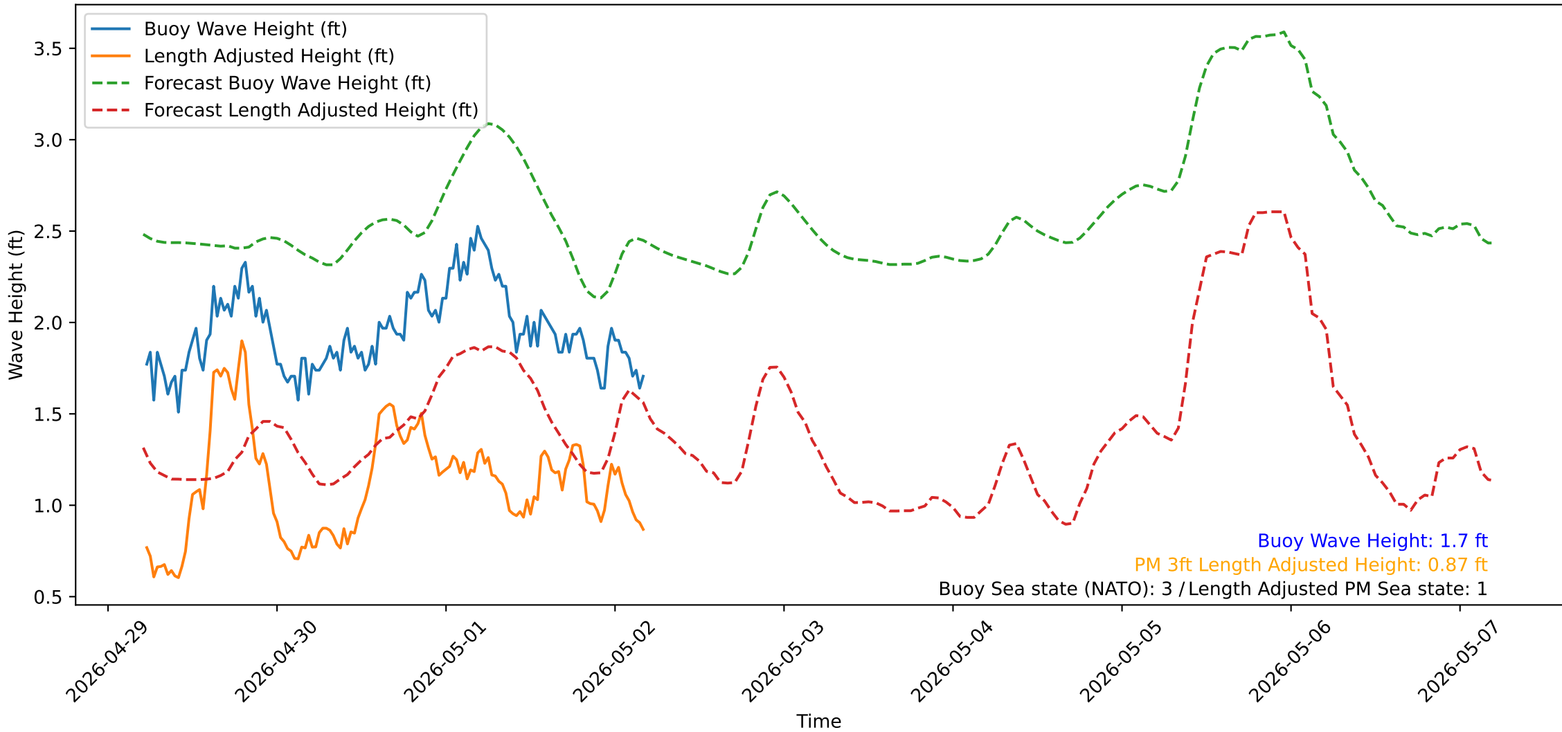
Wave Heights over Time for Red Beach at 2026-05-02 05:00:50
