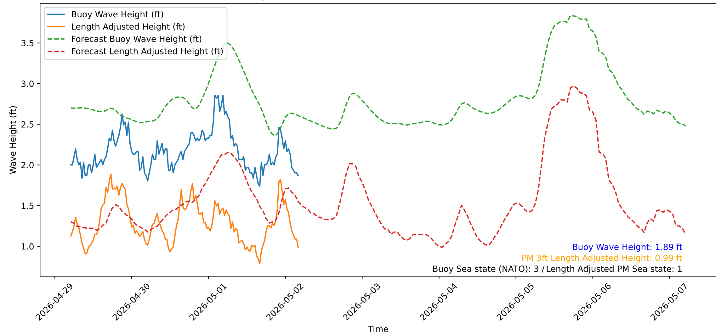
Wave Heights over Time for Green Beach at 2026-05-02 05:01:12
