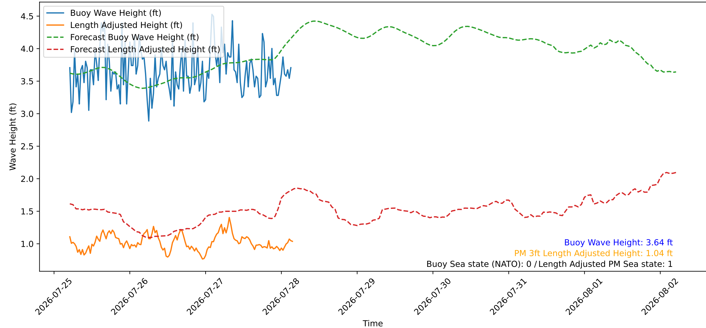
Wave Heights over Time for Red Beach at 2026-07-28 04:30:45
