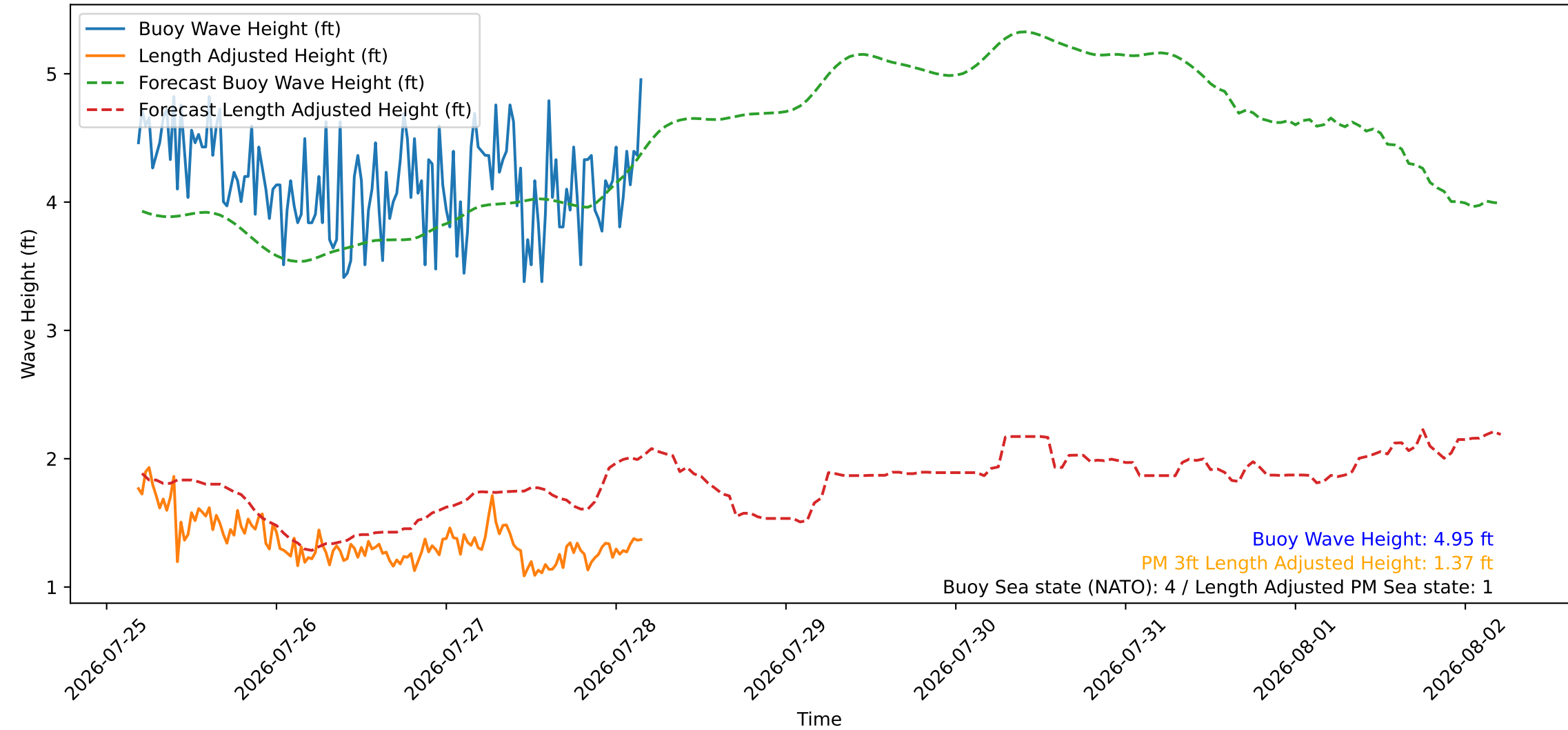
Wave Heights over Time for Green Beach at 2026-07-28 04:31:08
