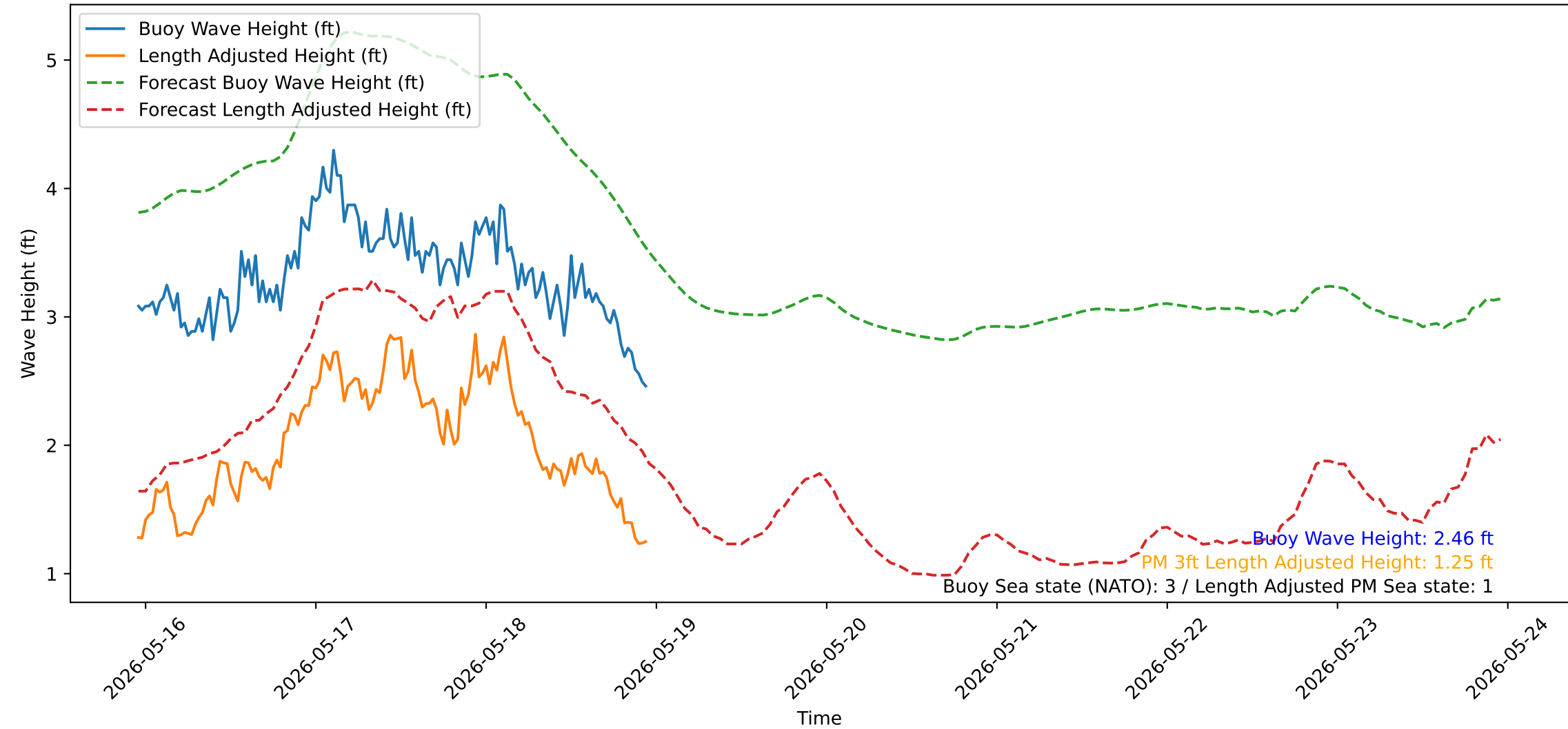
Wave Heights over Time for Oceanside Harbor at 2026-05-18 23:00:32
