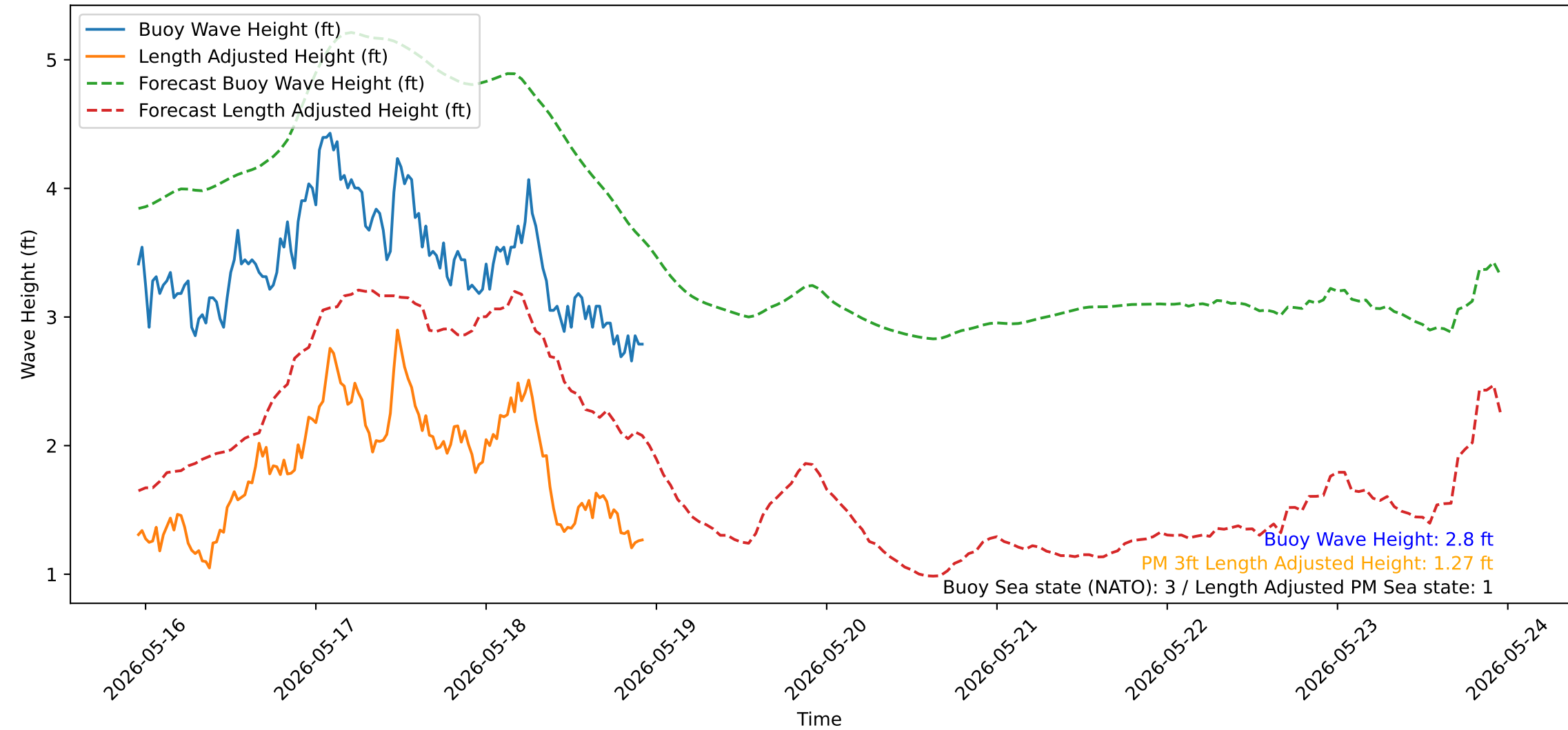
Wave Heights over Time for Green Beach at 2026-05-18 23:01:14
