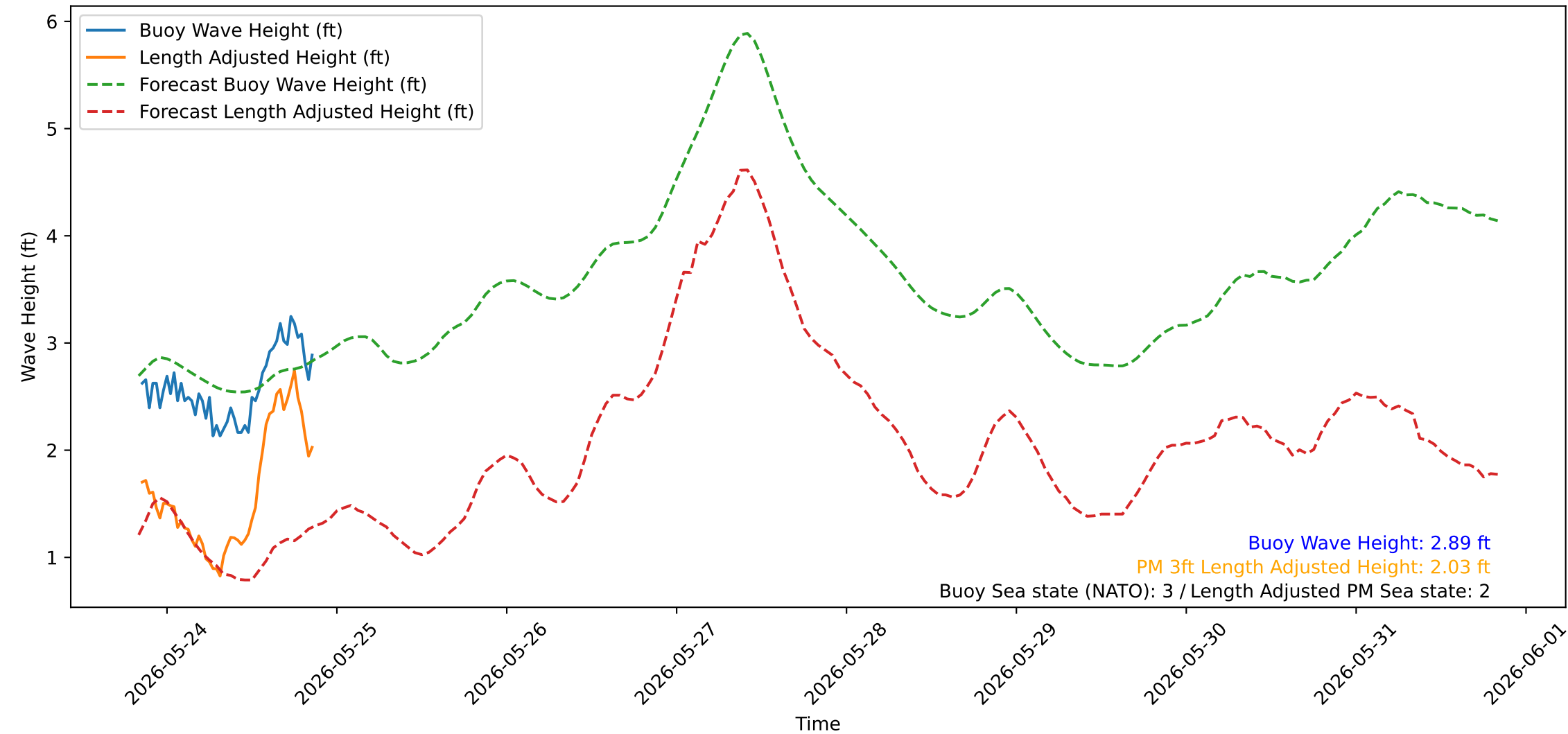
Wave Heights over Time for Oceanside Harbor at 2026-05-26 20:20:27
