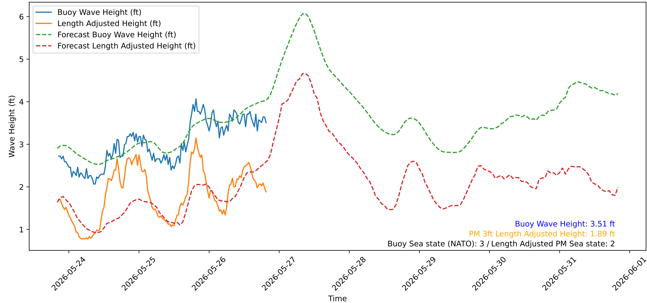
Wave Heights over Time for Green Beach at 2026-05-26 20:21:10
