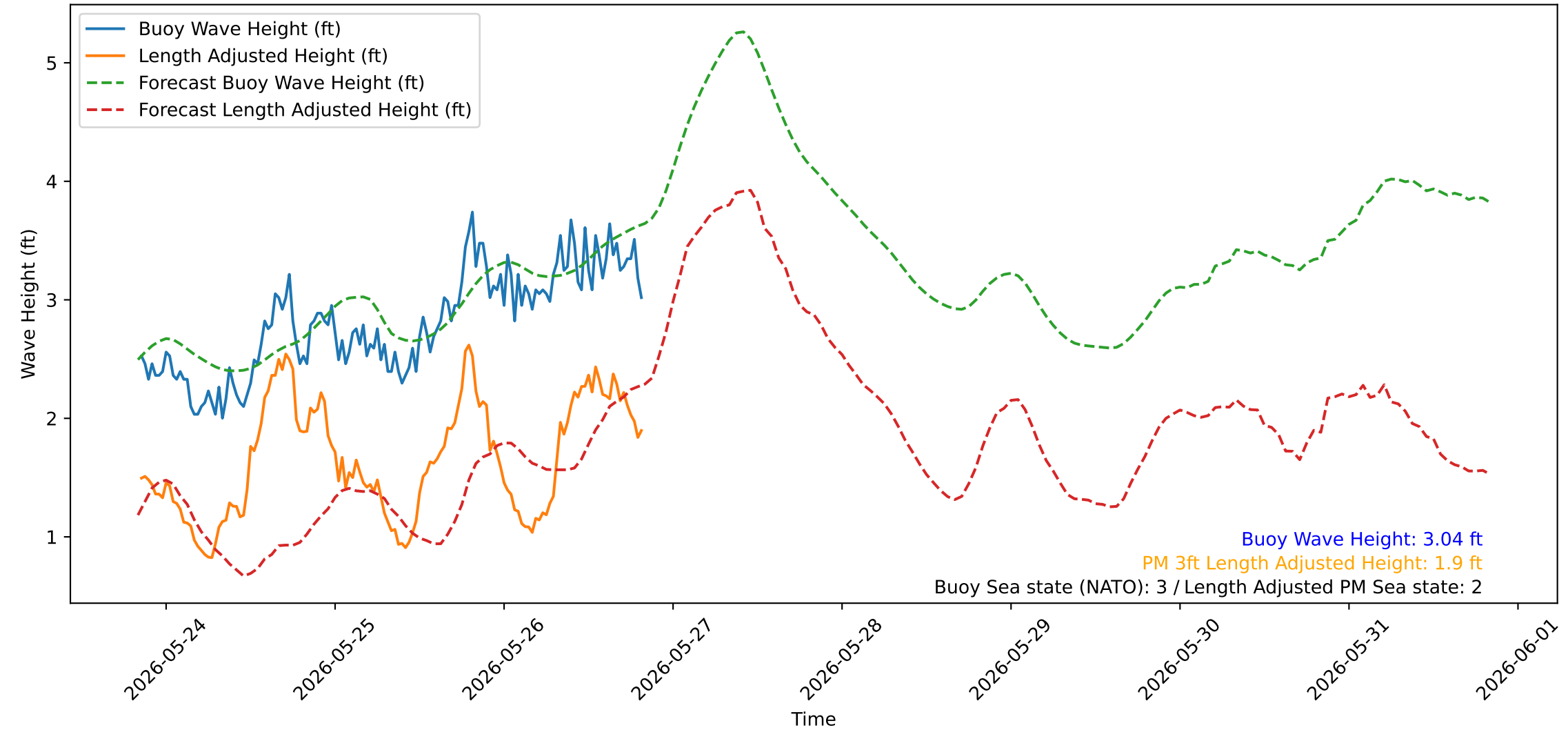
Wave Heights over Time for Red Beach at 2026-05-26 20:20:47
