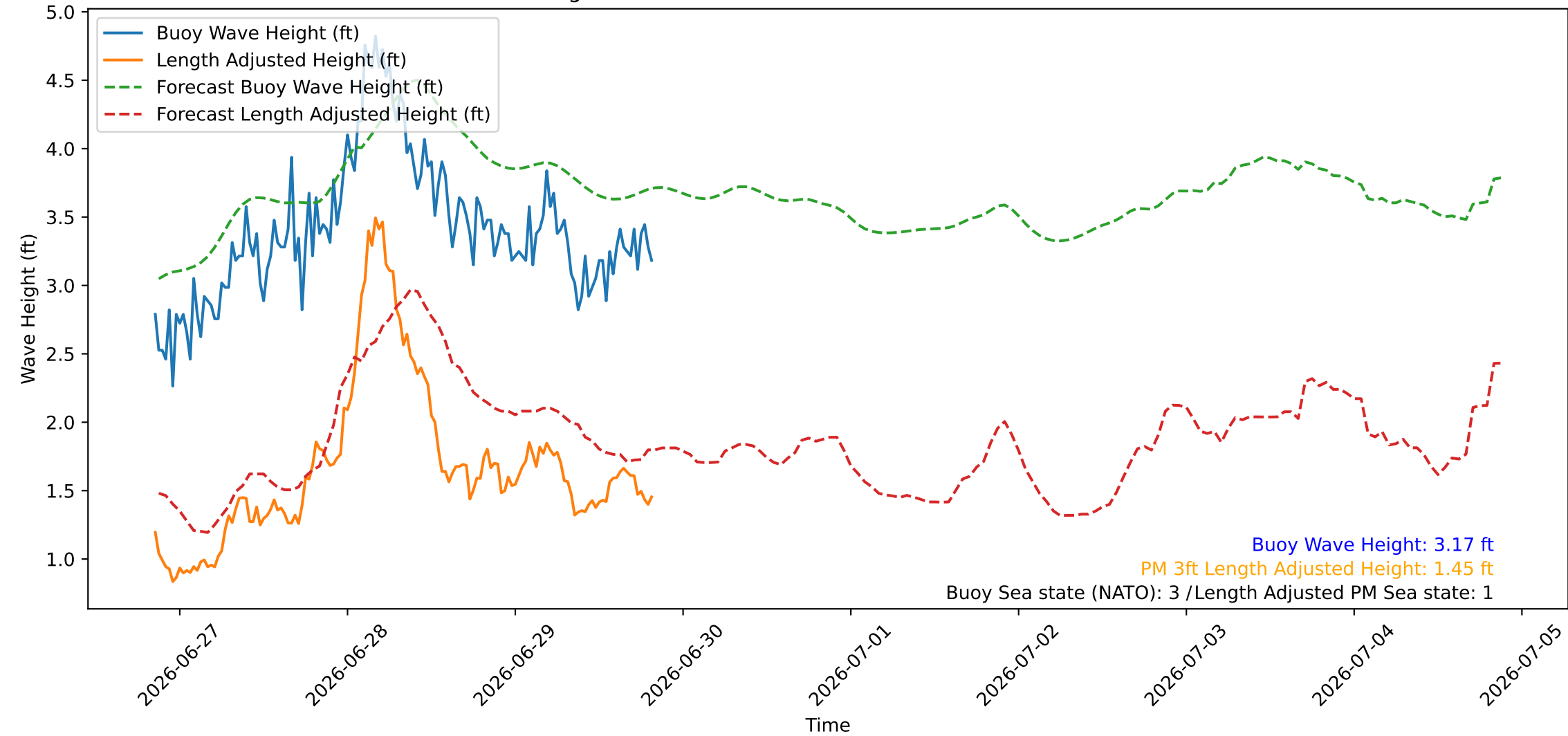
Wave Heights over Time for Green Beach at 2026-06-29 20:31:08
