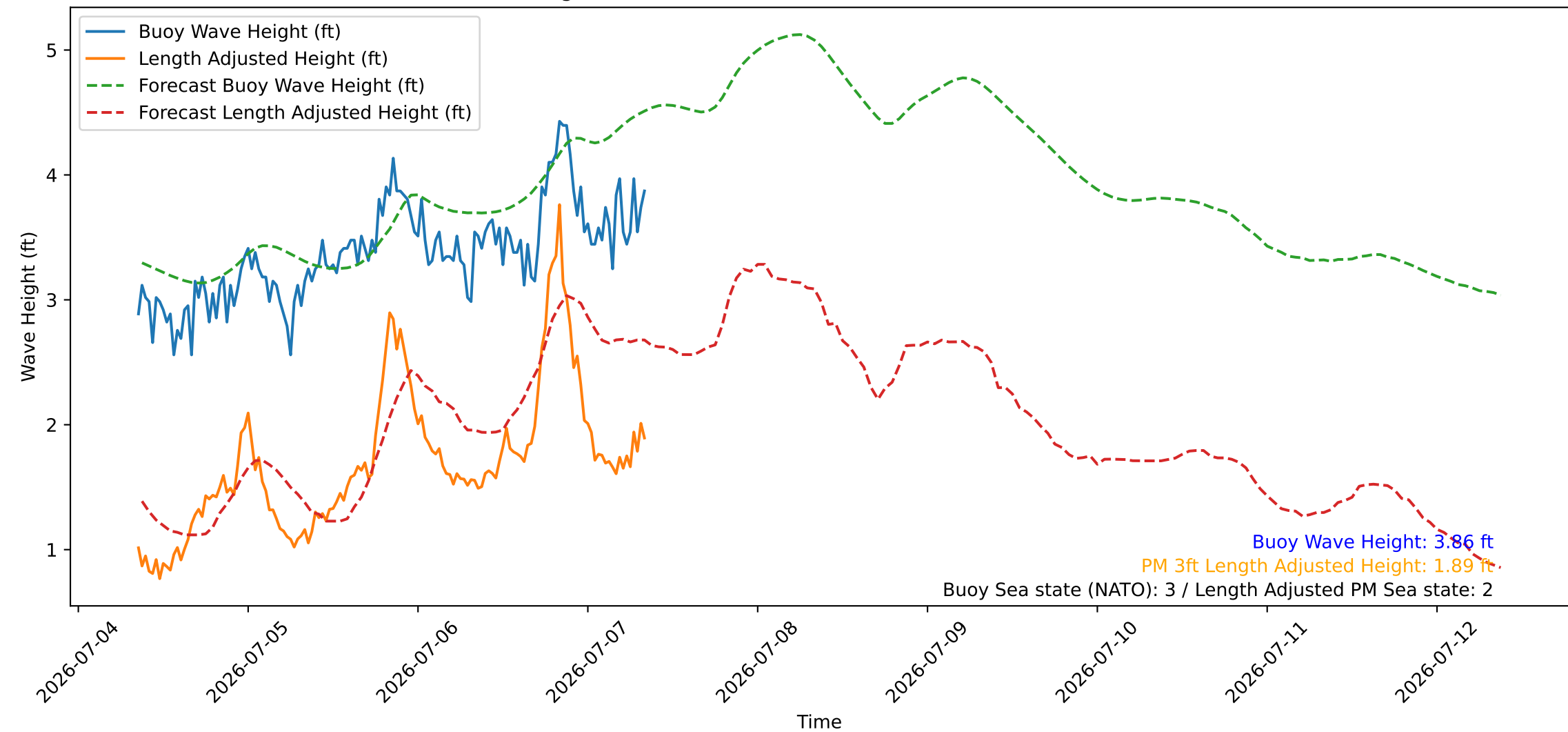
Wave Heights over Time for Green Beach at 2026-07-07 08:41:08
