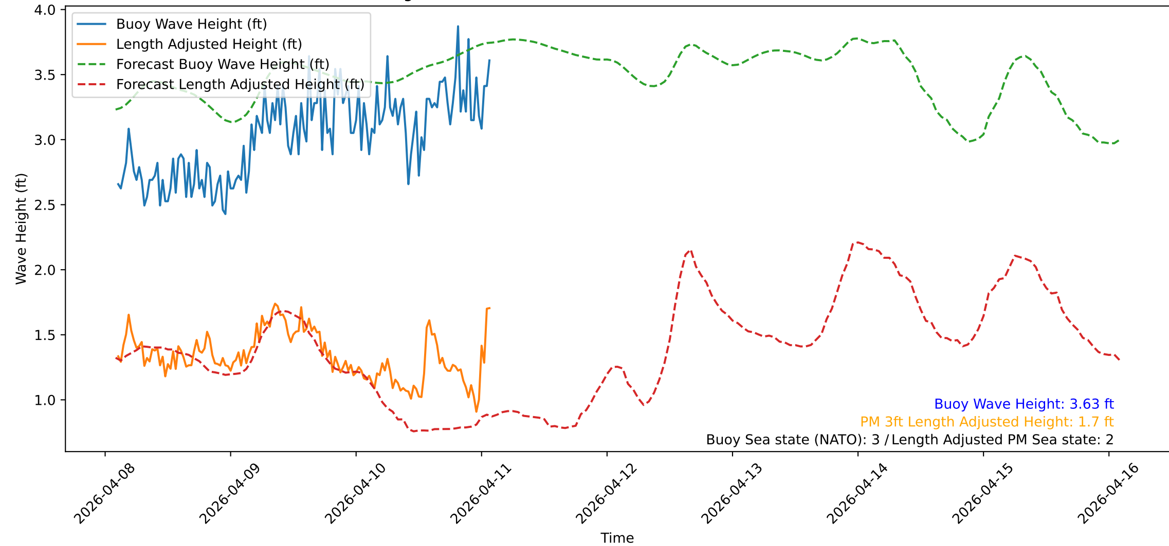
Wave Heights over Time for Oceanside Harbor at 2026-04-11 02:20:31
