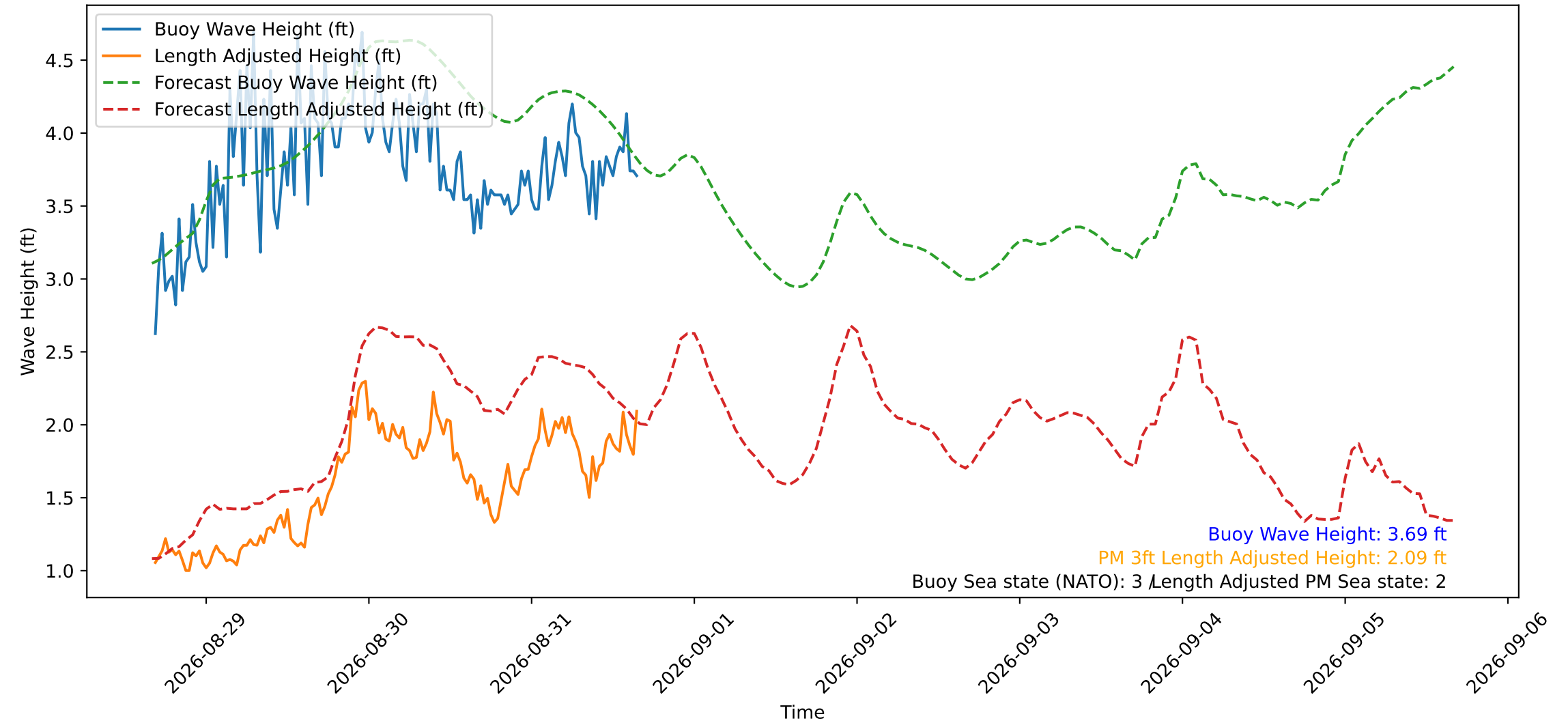
Wave Heights over Time for Red Beach at 2026-08-31 16:10:49
