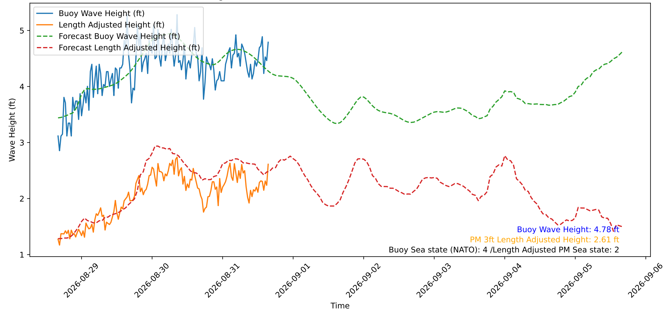
Wave Heights over Time for Oceanside Harbor at 2026-08-31 16:10:29
