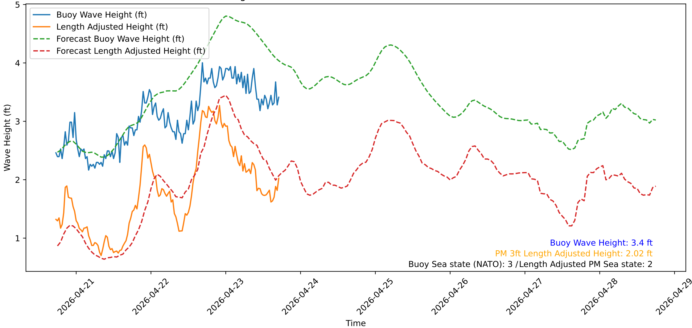
Wave Heights over Time for Green Beach at 2026-04-23 17:41:13
