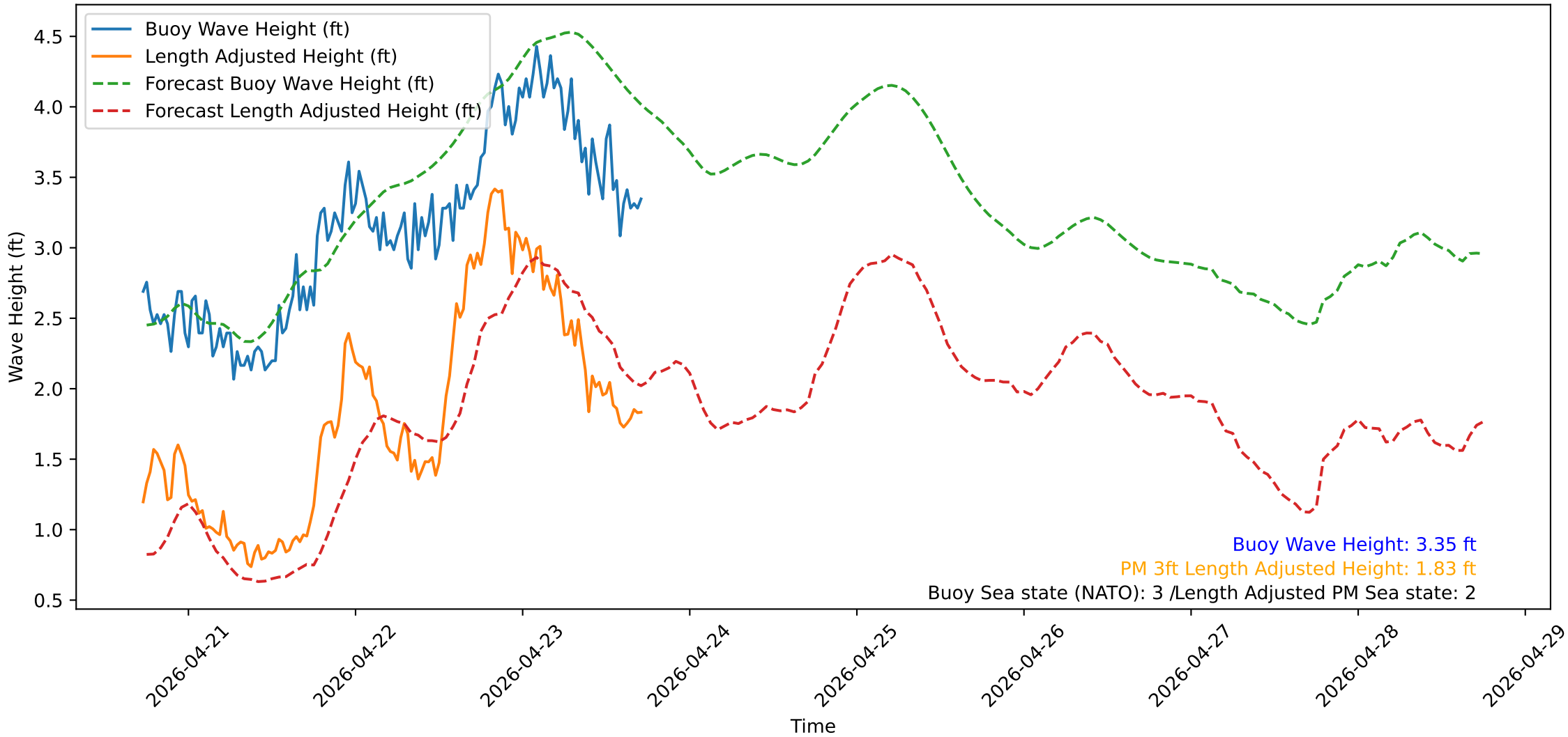
Wave Heights over Time for Oceanside Harbor at 2026-04-23 17:40:31
