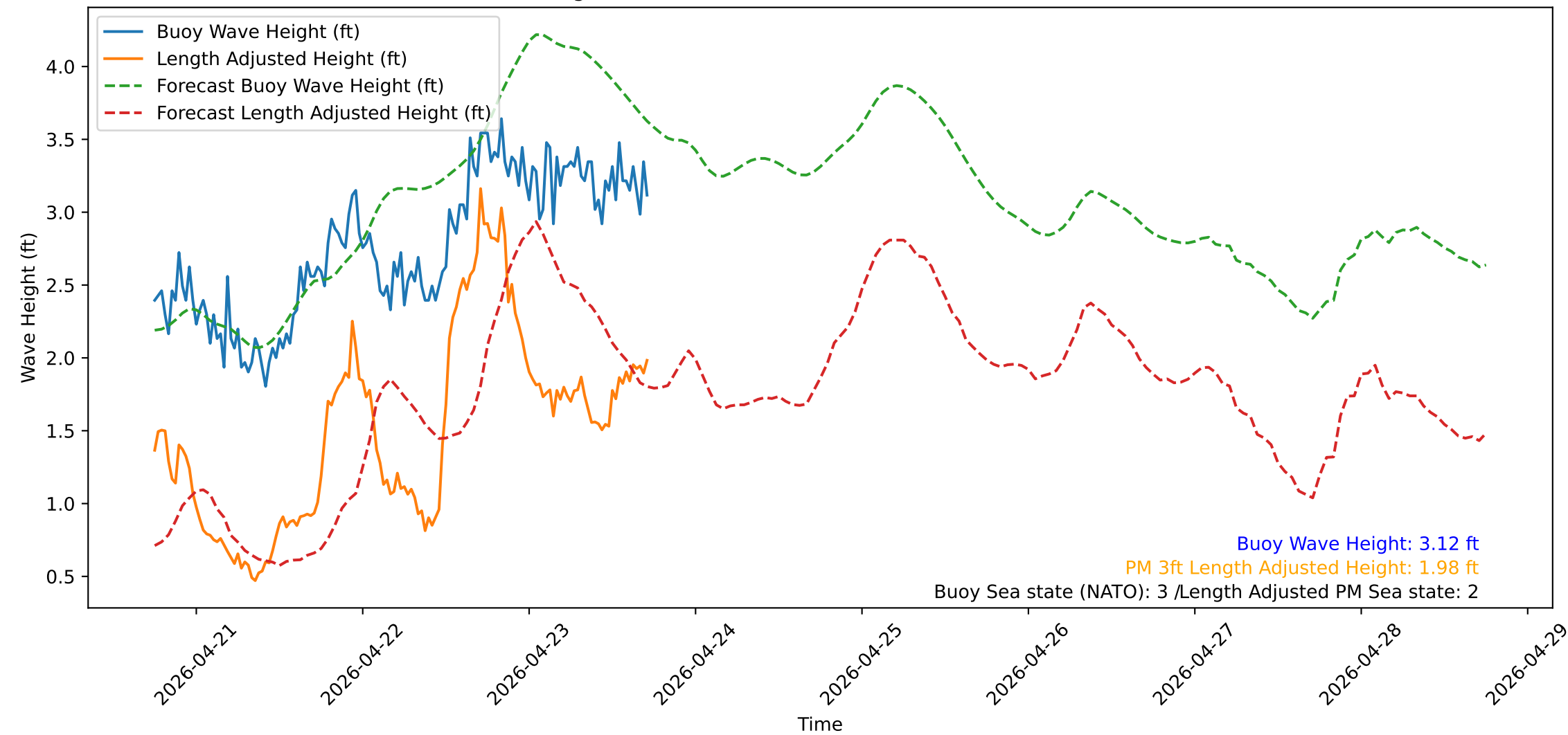
Wave Heights over Time for Red Beach at 2026-04-23 17:40:50
