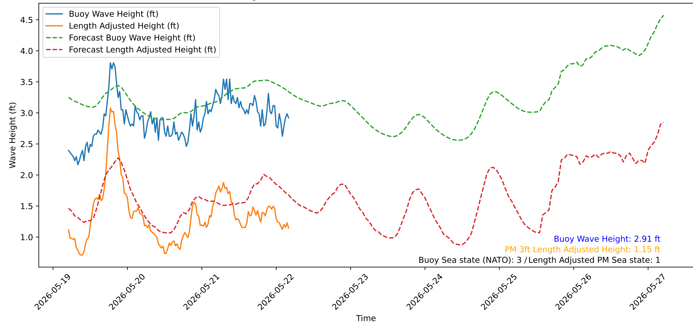
Wave Heights over Time for Green Beach at 2026-05-22 05:01:13
