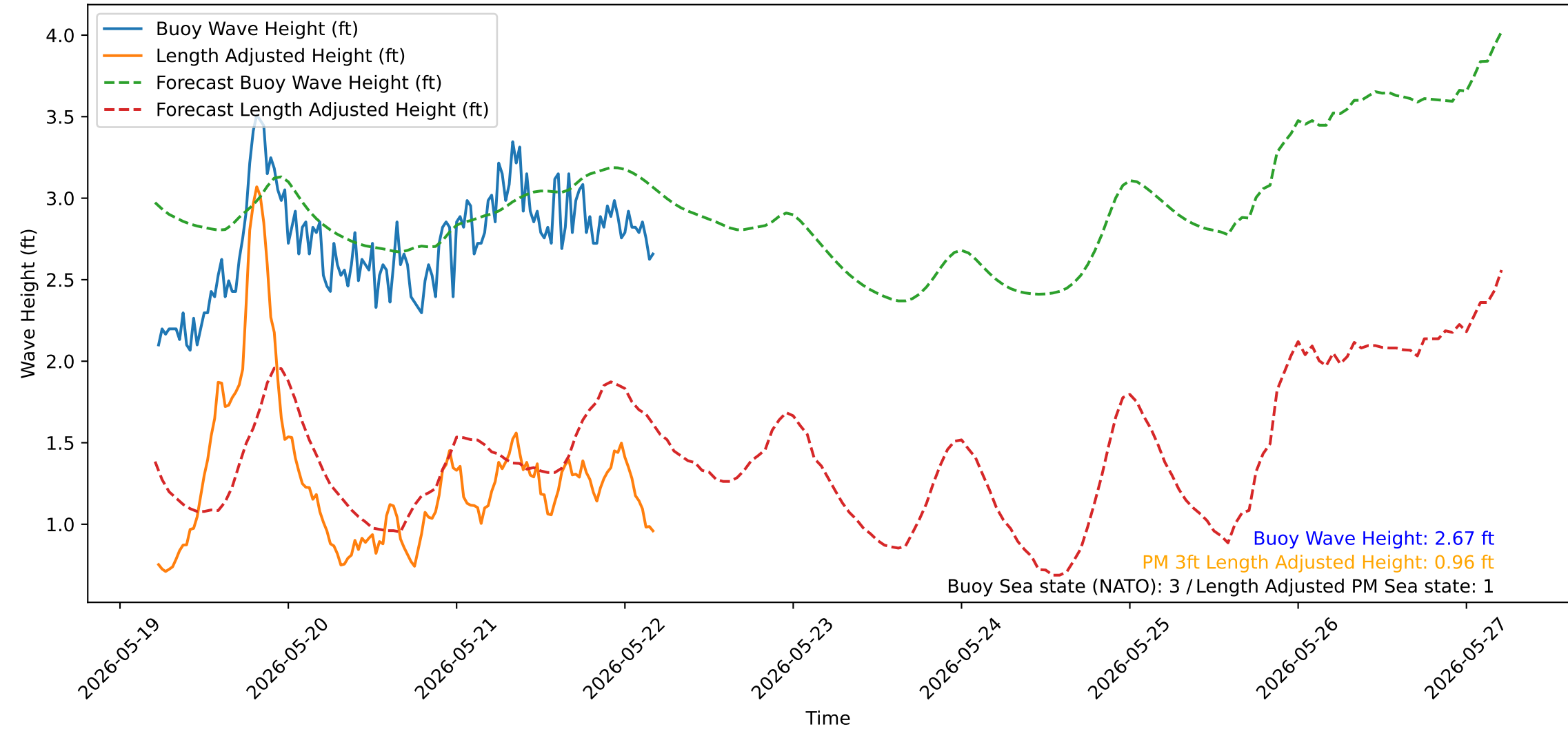
Wave Heights over Time for Red Beach at 2026-05-22 05:00:50
