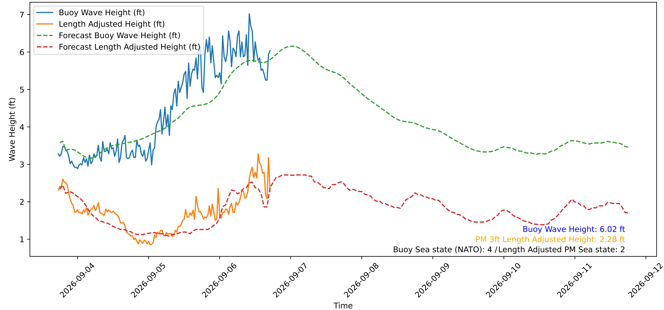
Wave Heights over Time for Oceanside Harbor at 2026-09-06 17:30:29
