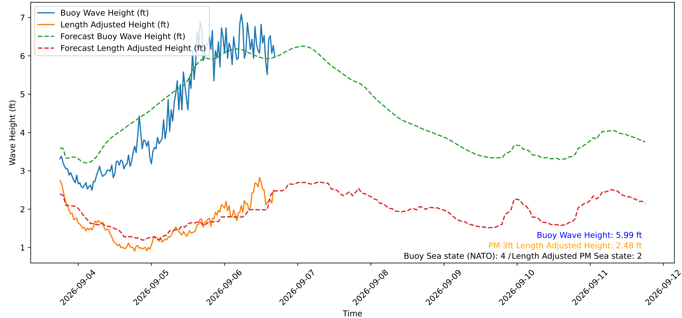
Wave Heights over Time for Green Beach at 2026-09-06 17:31:12
