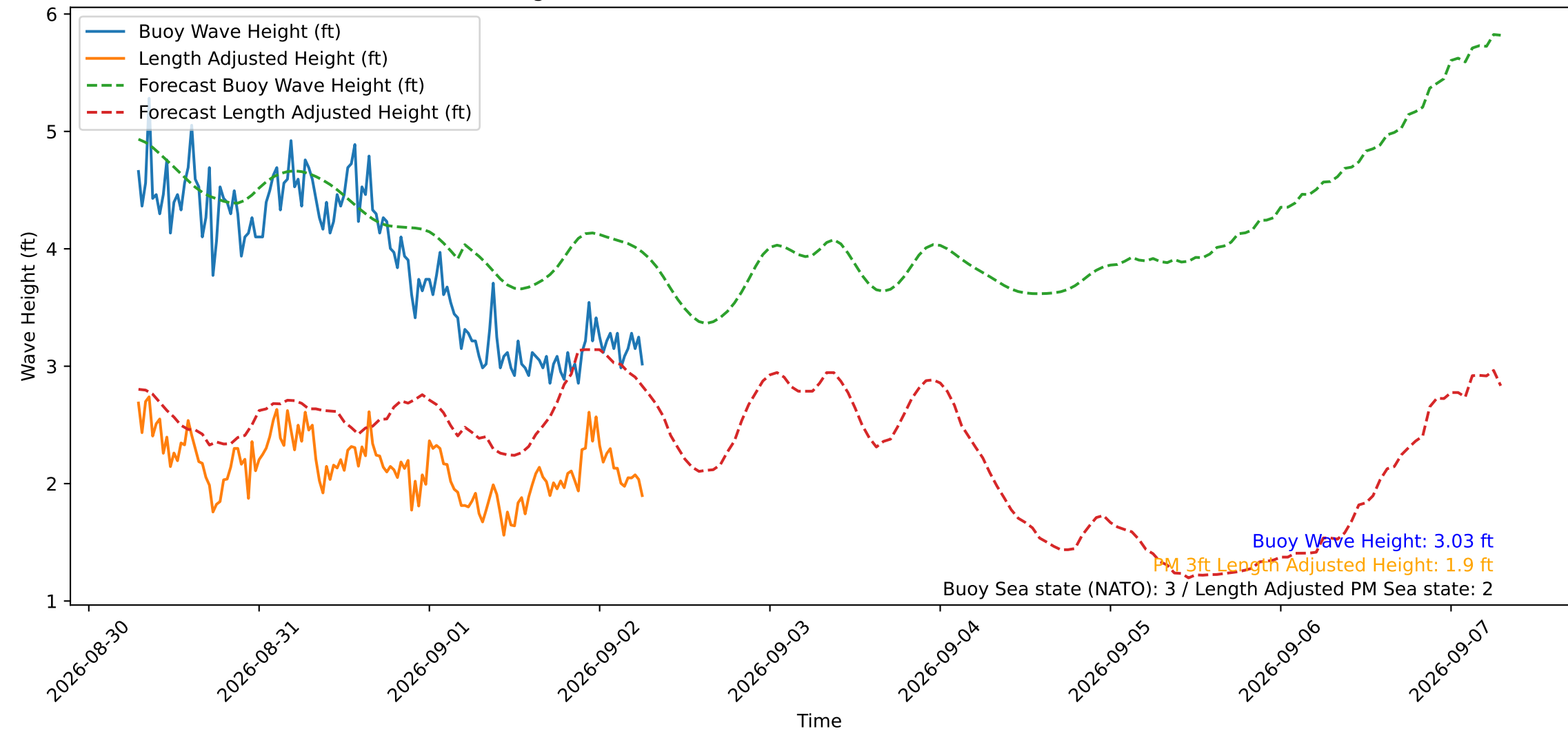
Wave Heights over Time for Oceanside Harbor at 2026-09-02 07:10:29
