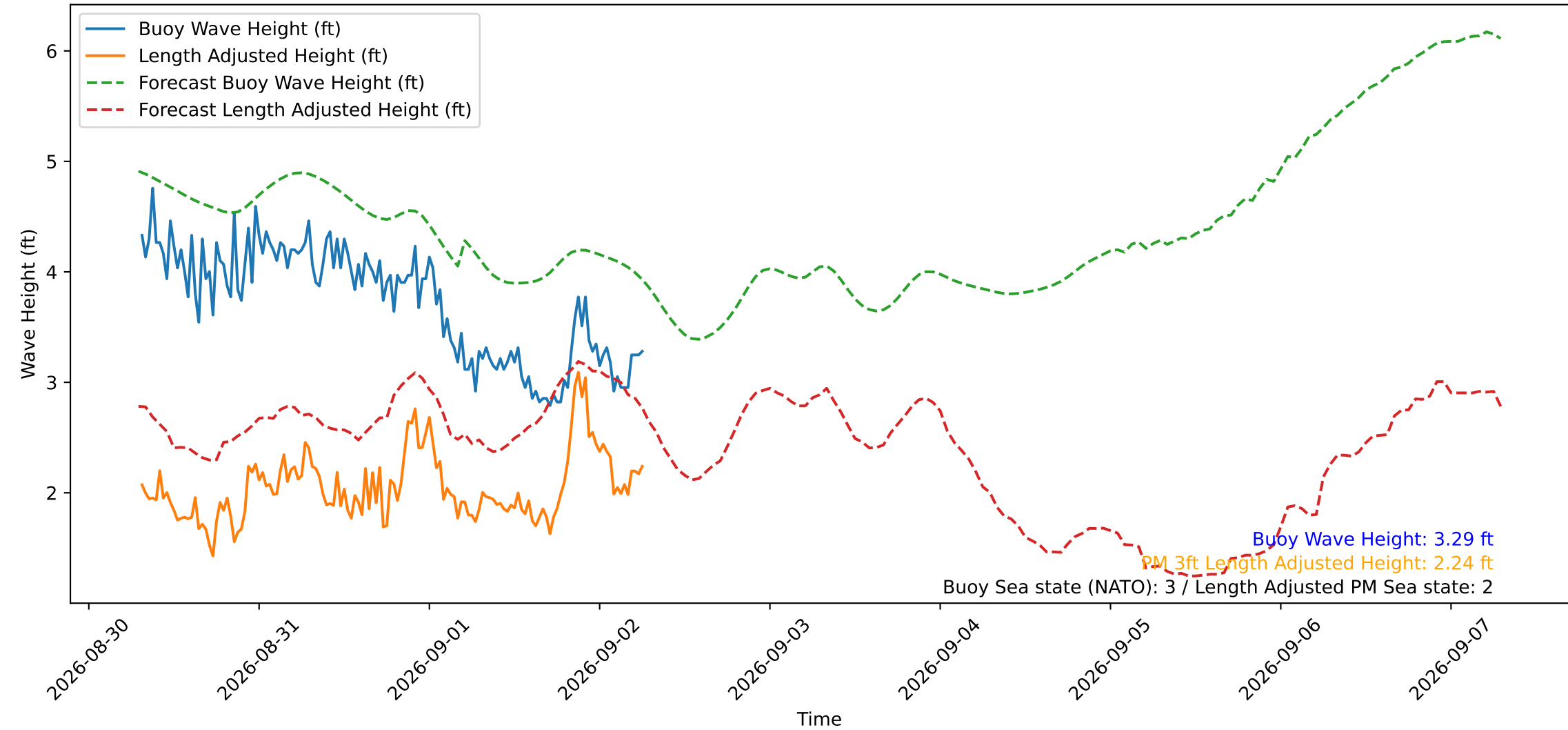
Wave Heights over Time for Green Beach at 2026-09-02 07:11:11
