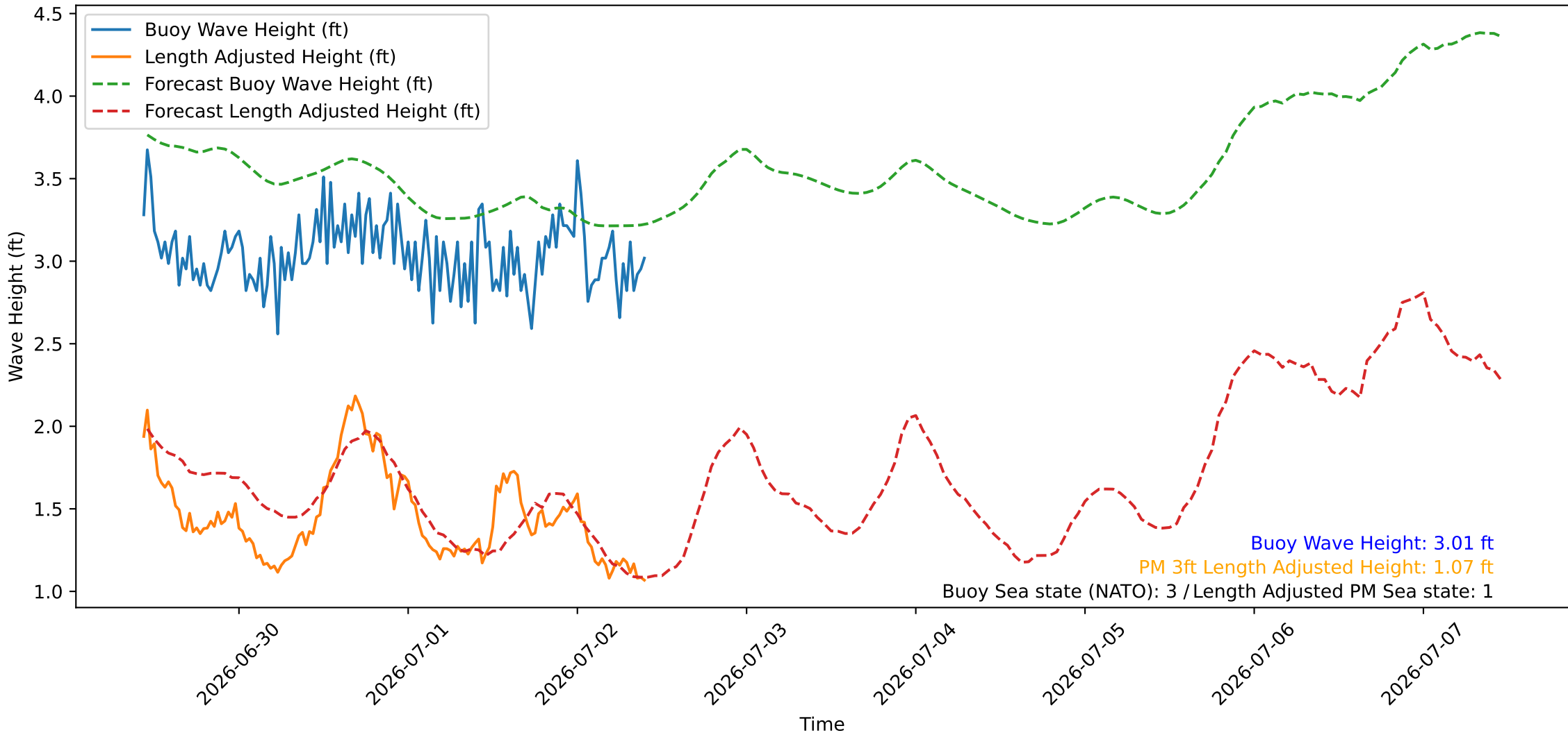
Wave Heights over Time for Oceanside Harbor at 2026-07-02 10:30:27
