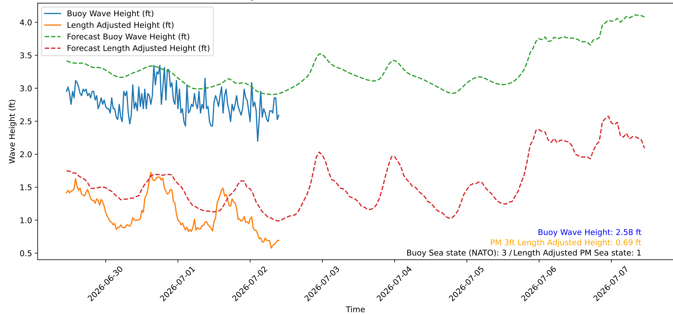
Wave Heights over Time for Red Beach at 2026-07-02 10:30:46
