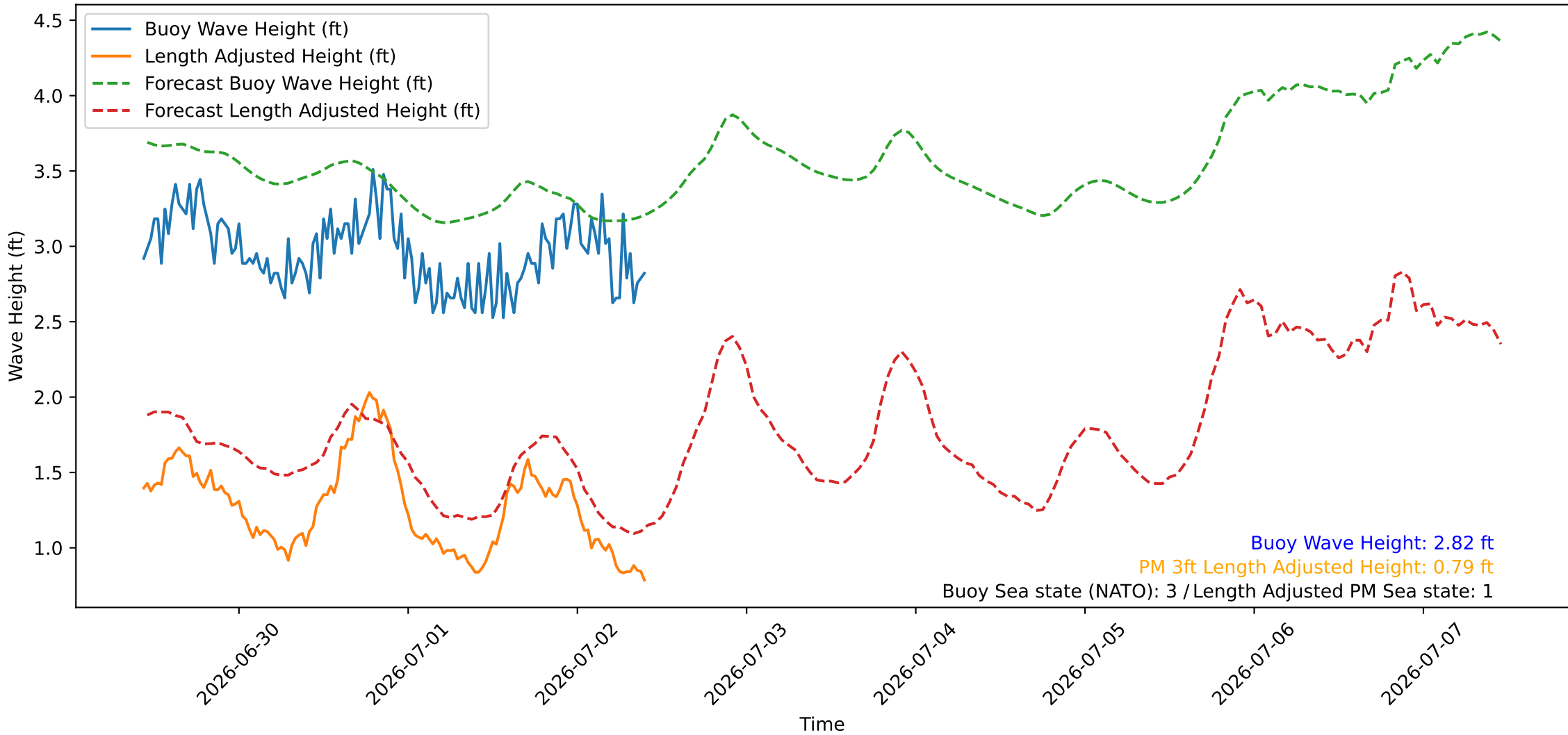
Wave Heights over Time for Green Beach at 2026-07-02 10:31:08
