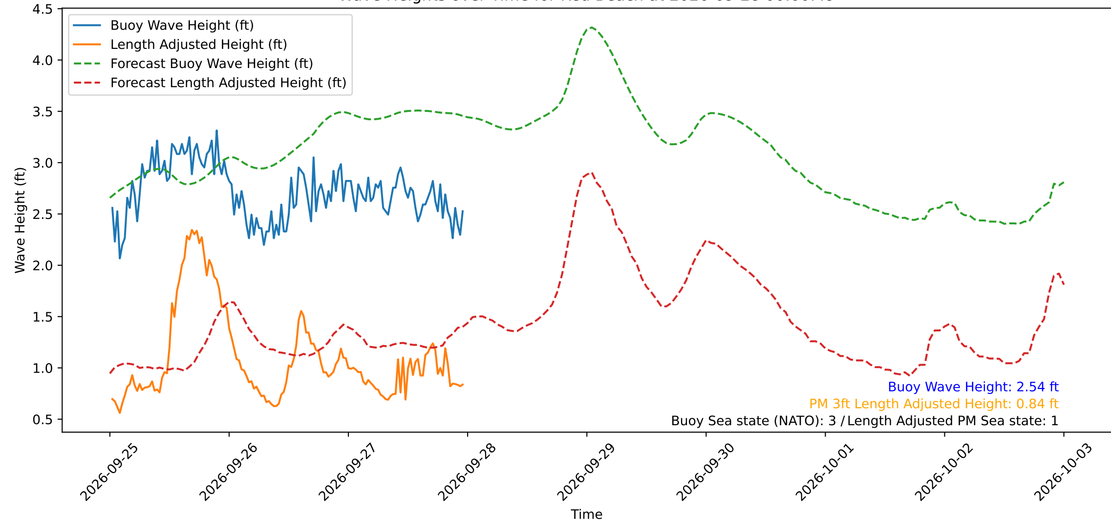
Wave Heights over Time for Red Beach at 2026-09-28 00:00:49
