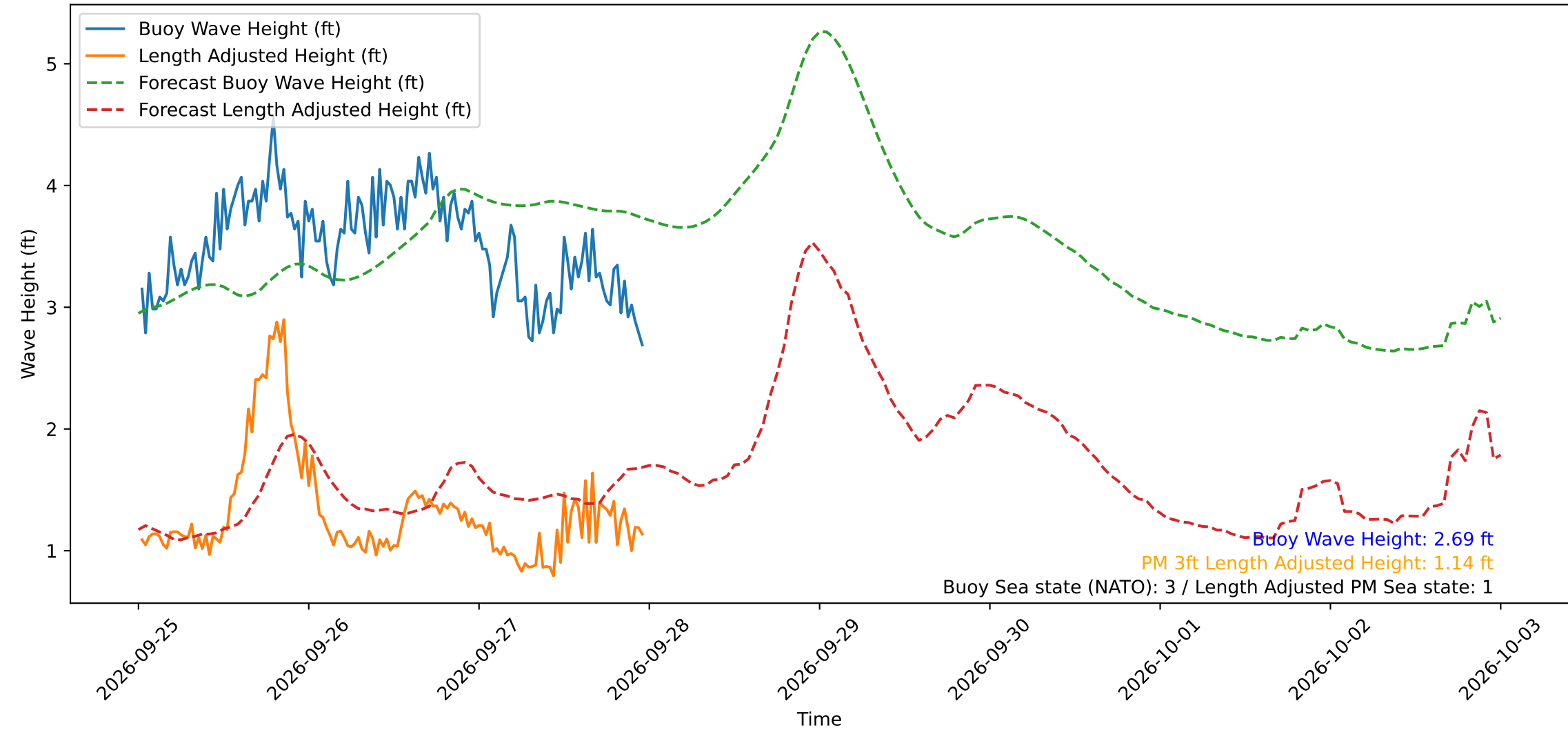
Wave Heights over Time for Green Beach at 2026-09-28 00:01:12
