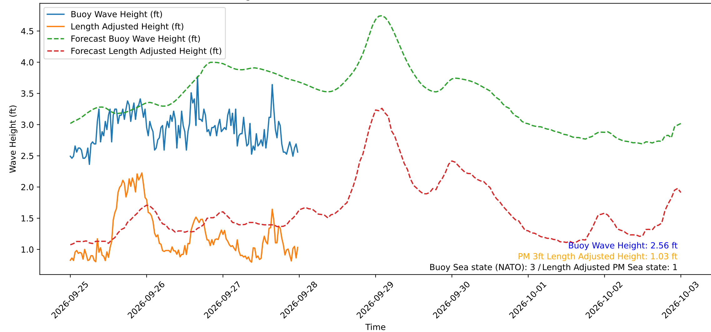
Wave Heights over Time for Oceanside Harbor at 2026-09-28 00:00:30
