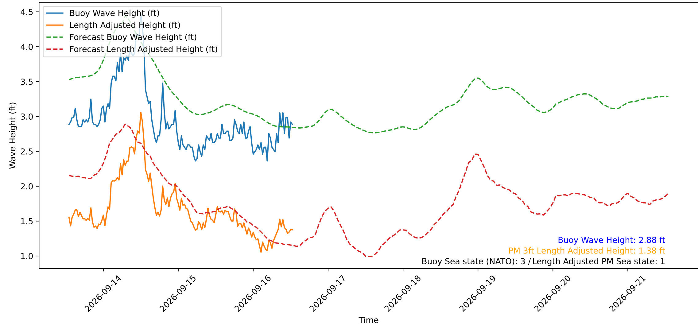
Wave Heights over Time for Oceanside Harbor at 2026-09-16 13:10:30
