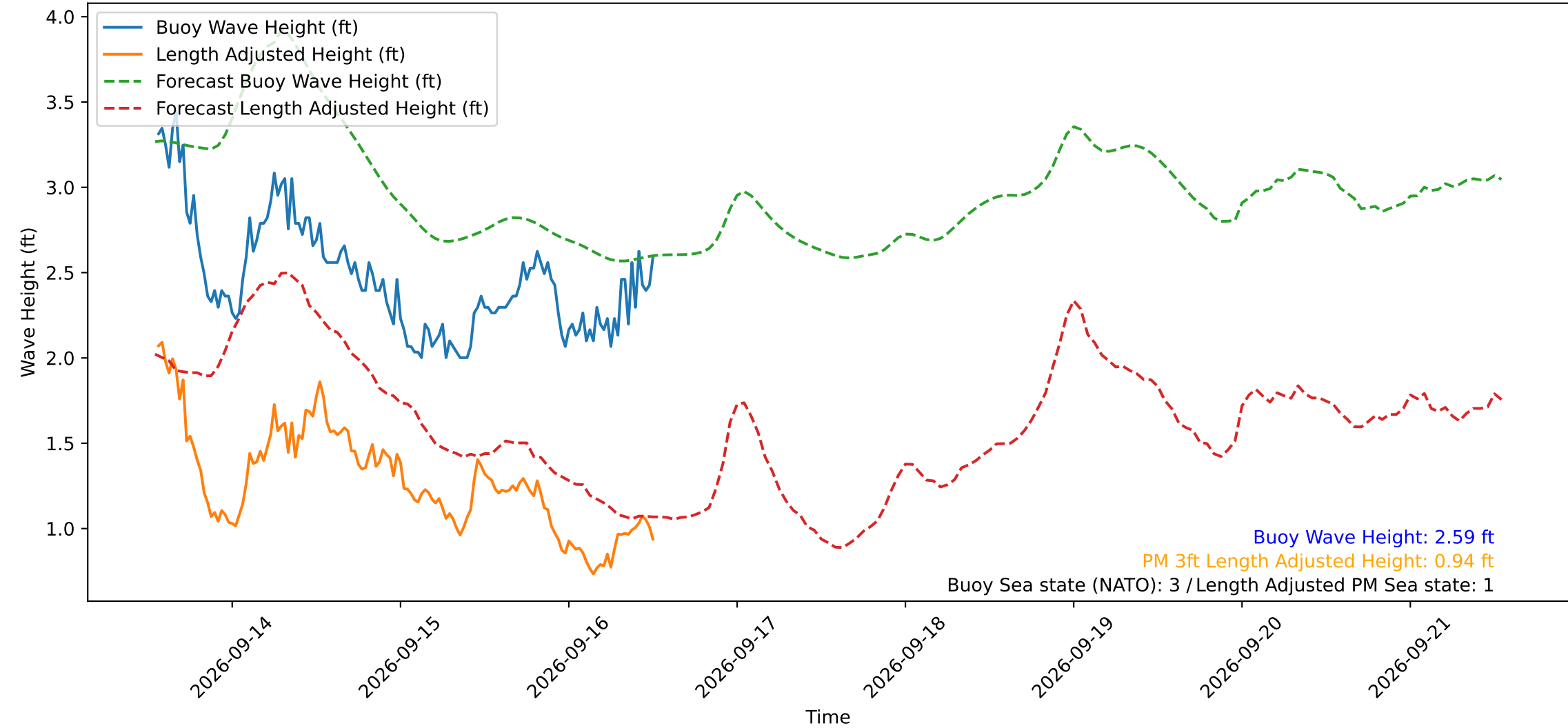
Wave Heights over Time for Red Beach at 2026-09-16 13:10:49
