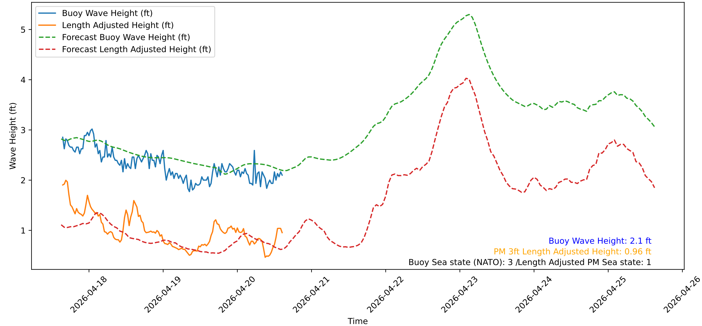
Wave Heights over Time for Red Beach at 2026-04-20 15:20:52
