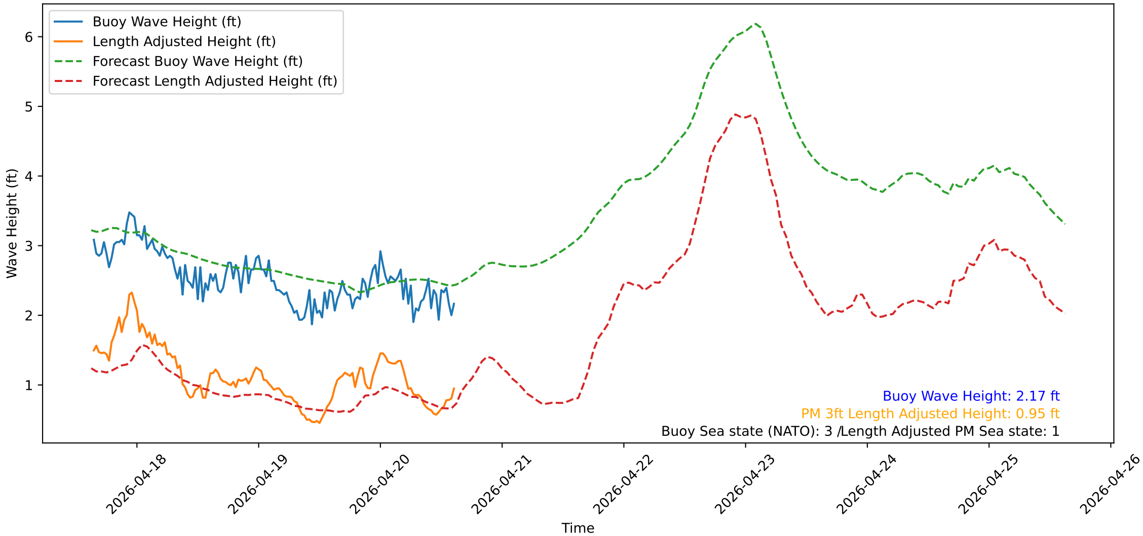
Wave Heights over Time for Green Beach at 2026-04-20 15:21:14
