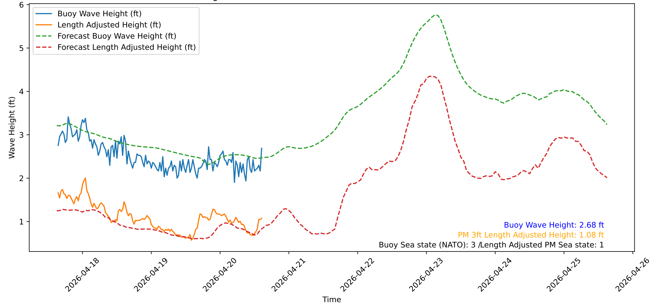
Wave Heights over Time for Oceanside Harbor at 2026-04-20 15:20:32
