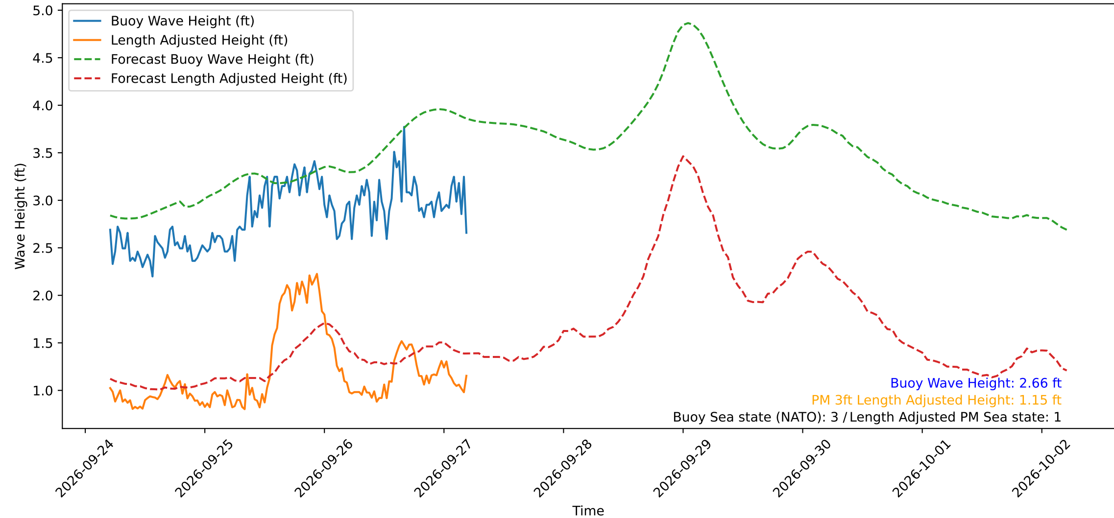
Wave Heights over Time for Oceanside Harbor at 2026-09-27 05:10:29
