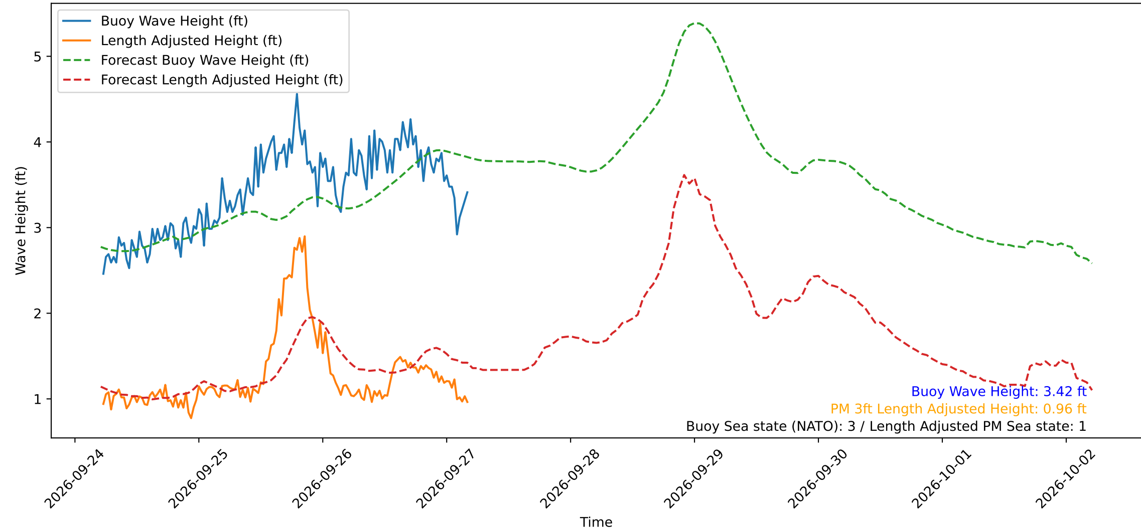
Wave Heights over Time for Green Beach at 2026-09-27 05:11:12
