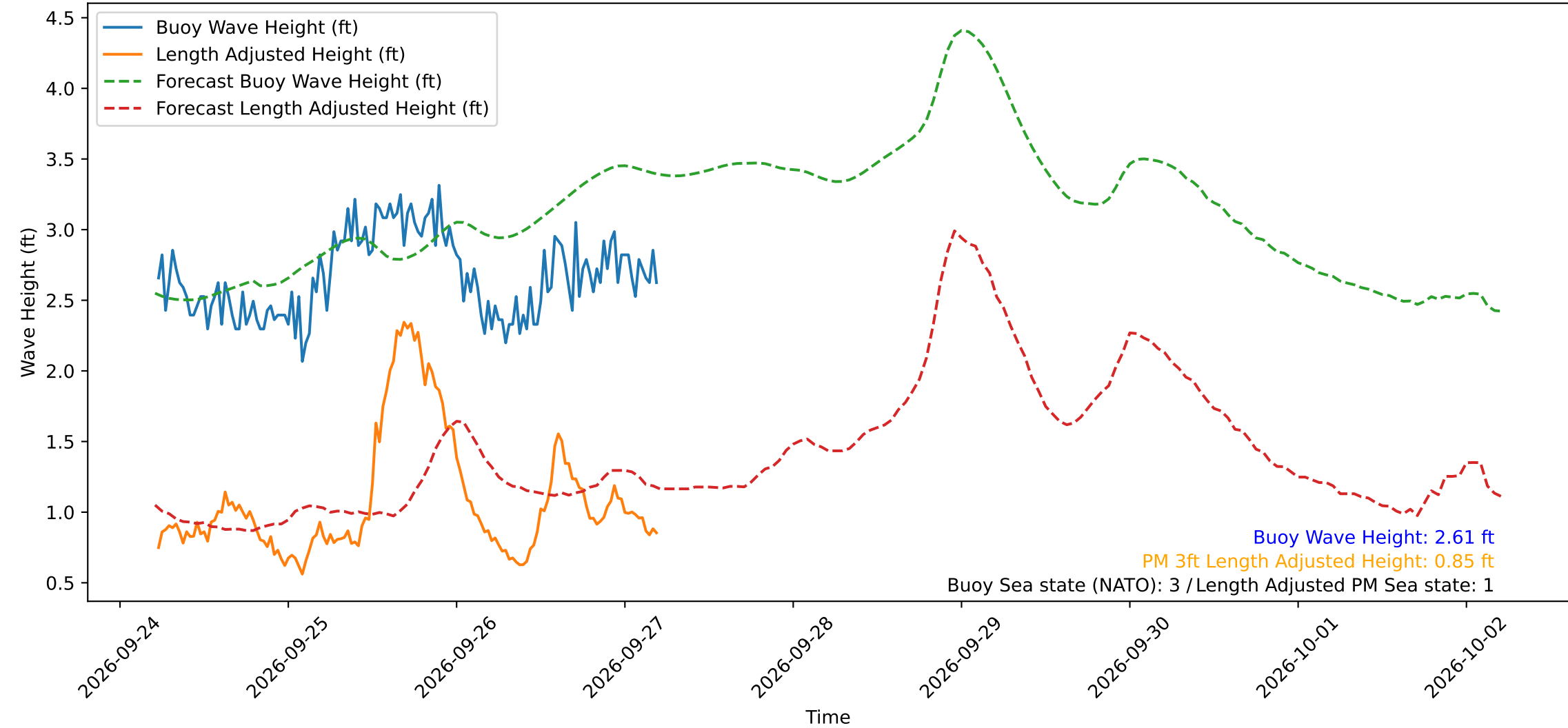
Wave Heights over Time for Red Beach at 2026-09-27 05:10:49
