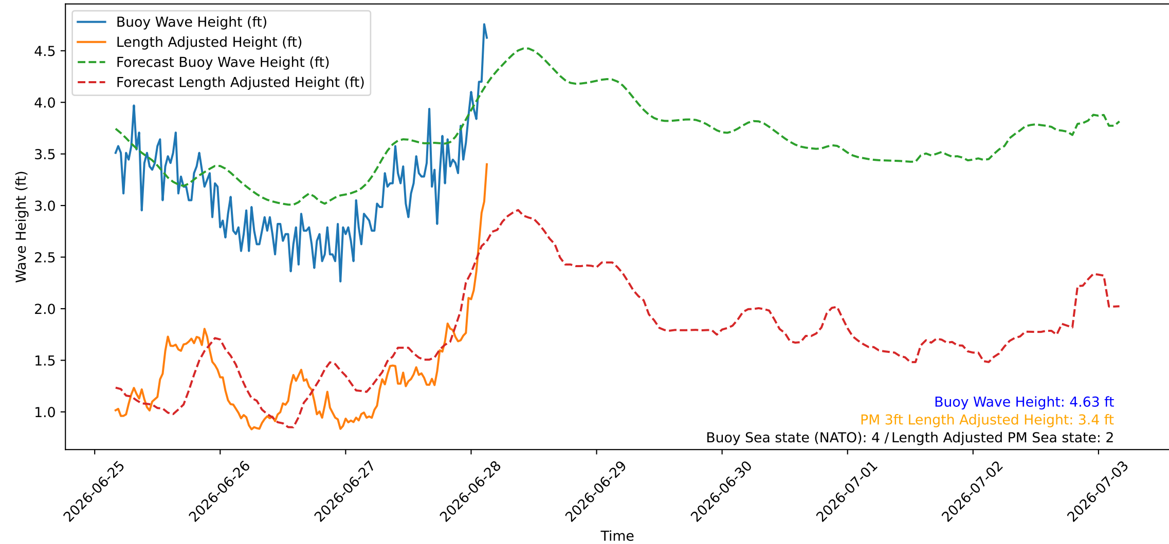
Wave Heights over Time for Green Beach at 2026-06-28 03:51:09
