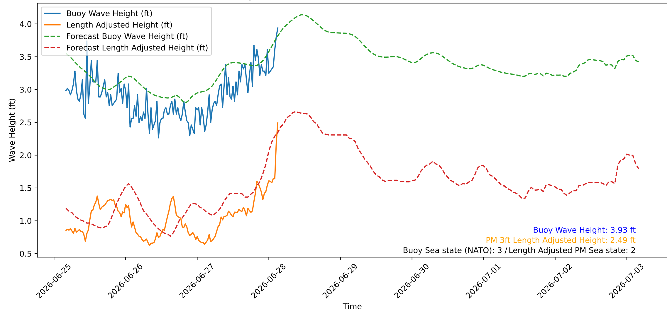
Wave Heights over Time for Red Beach at 2026-06-28 03:50:46
