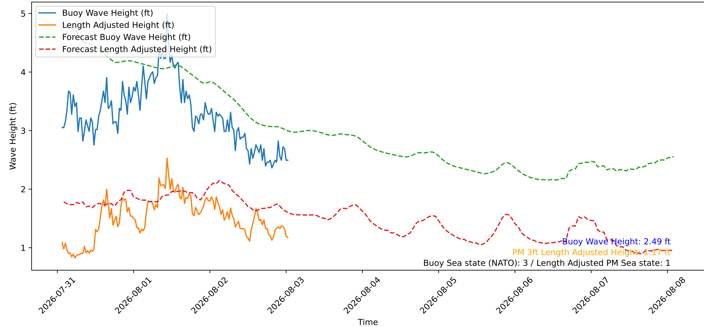
Wave Heights over Time for Green Beach at 2026-08-03 01:31:08
