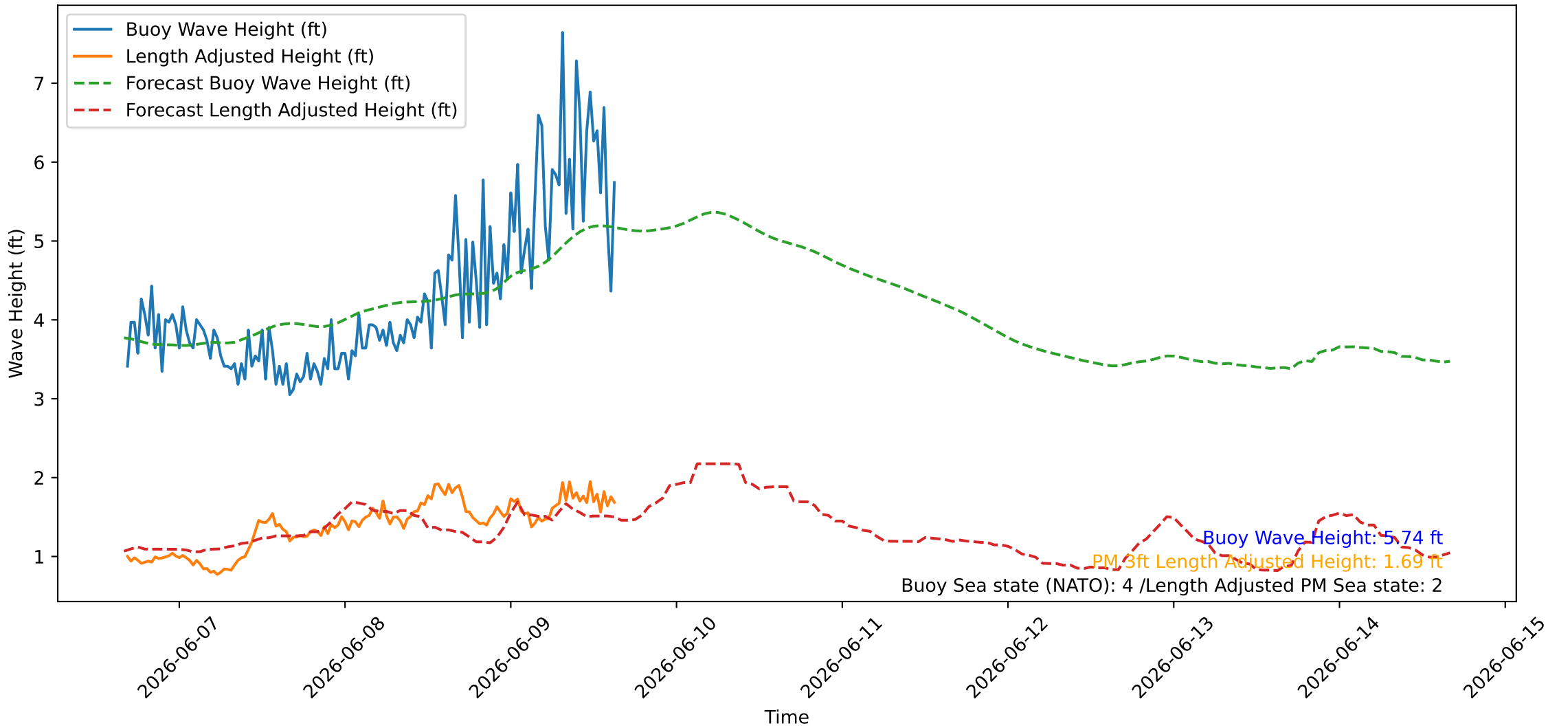
Wave Heights over Time for Red Beach at 2026-06-09 16:00:45
