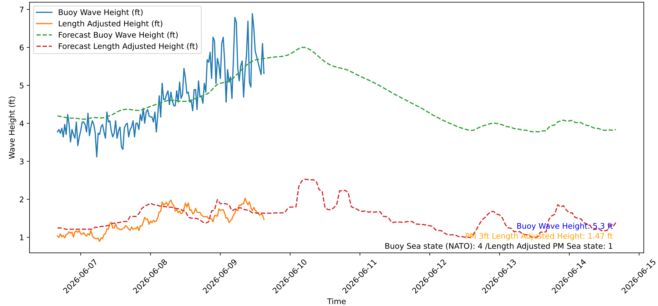
Wave Heights over Time for Green Beach at 2026-06-09 16:01:08
