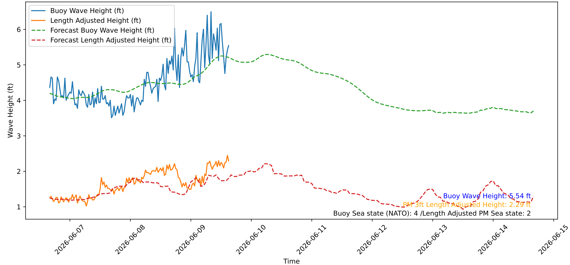
Wave Heights over Time for Oceanside Harbor at 2026-06-09 16:00:26
