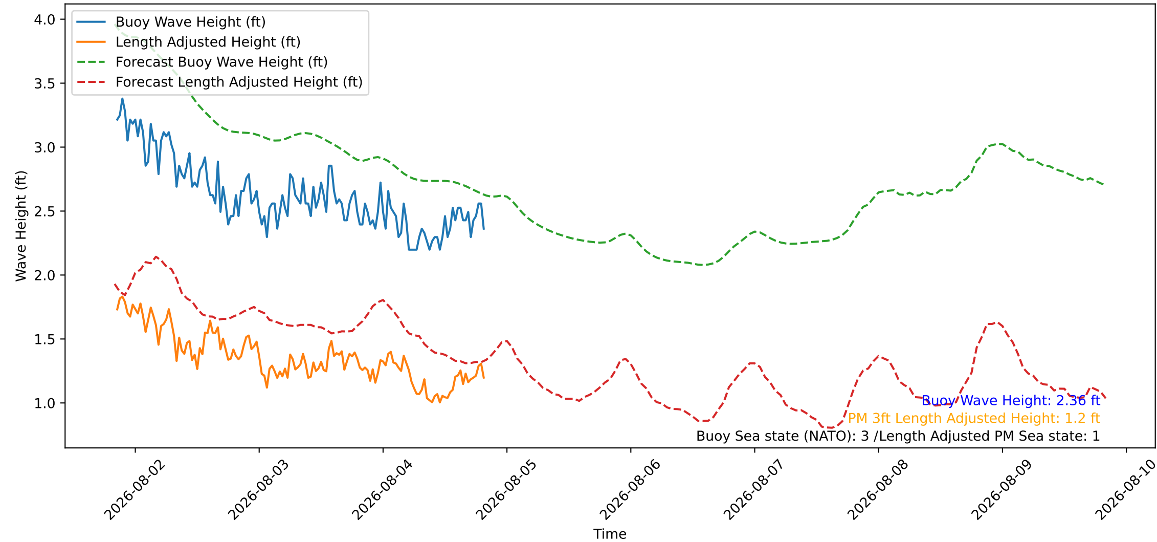
Wave Heights over Time for Oceanside Harbor at 2026-08-04 20:20:26
