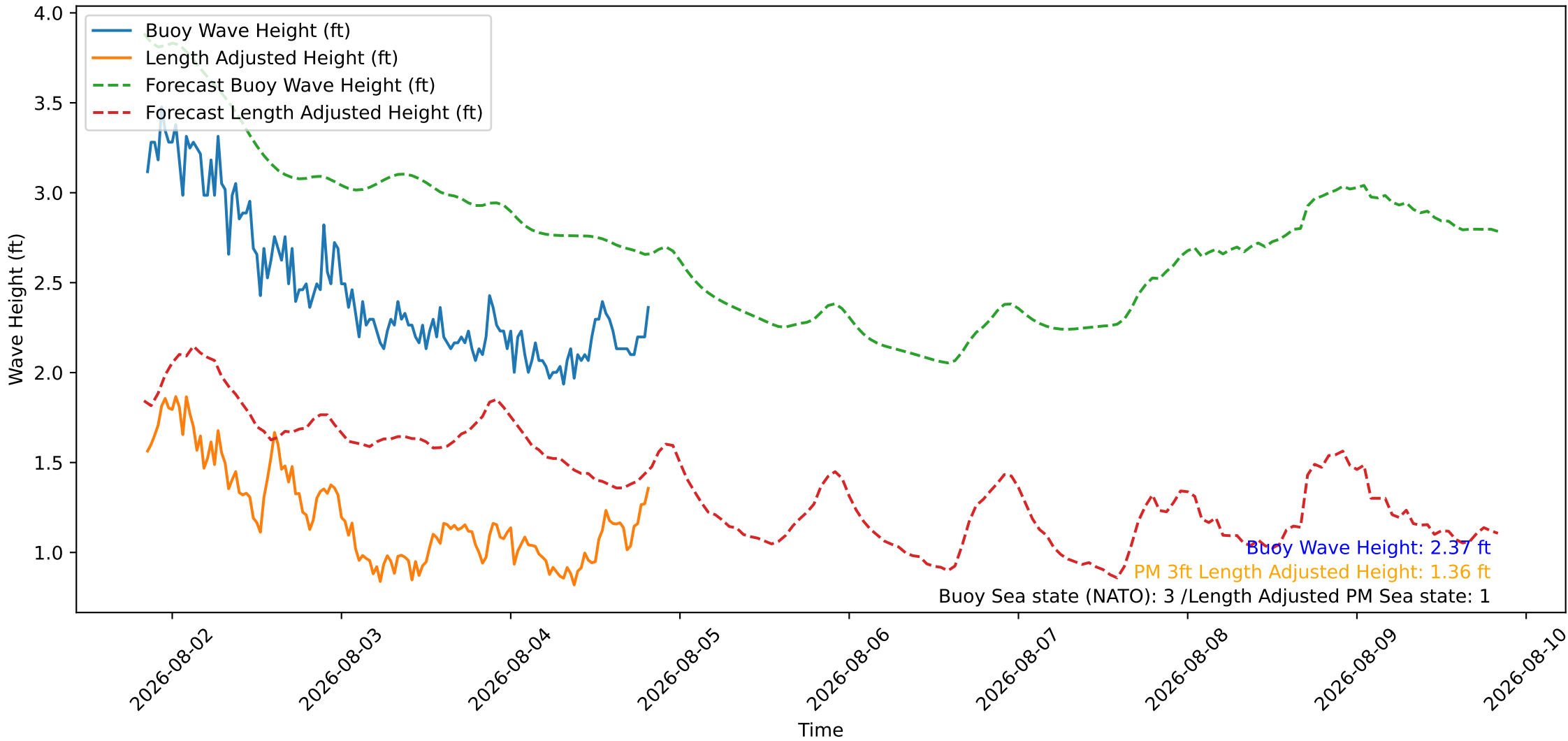
Wave Heights over Time for Green Beach at 2026-08-04 20:21:10
