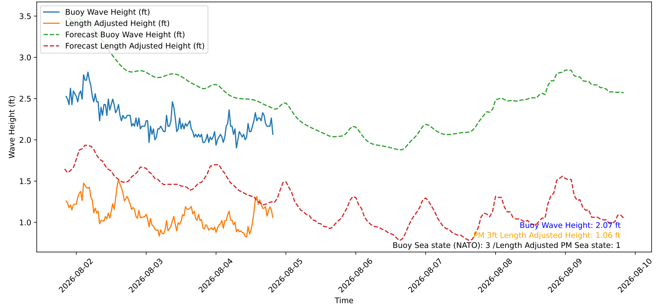
Wave Heights over Time for Red Beach at 2026-08-04 20:20:47
