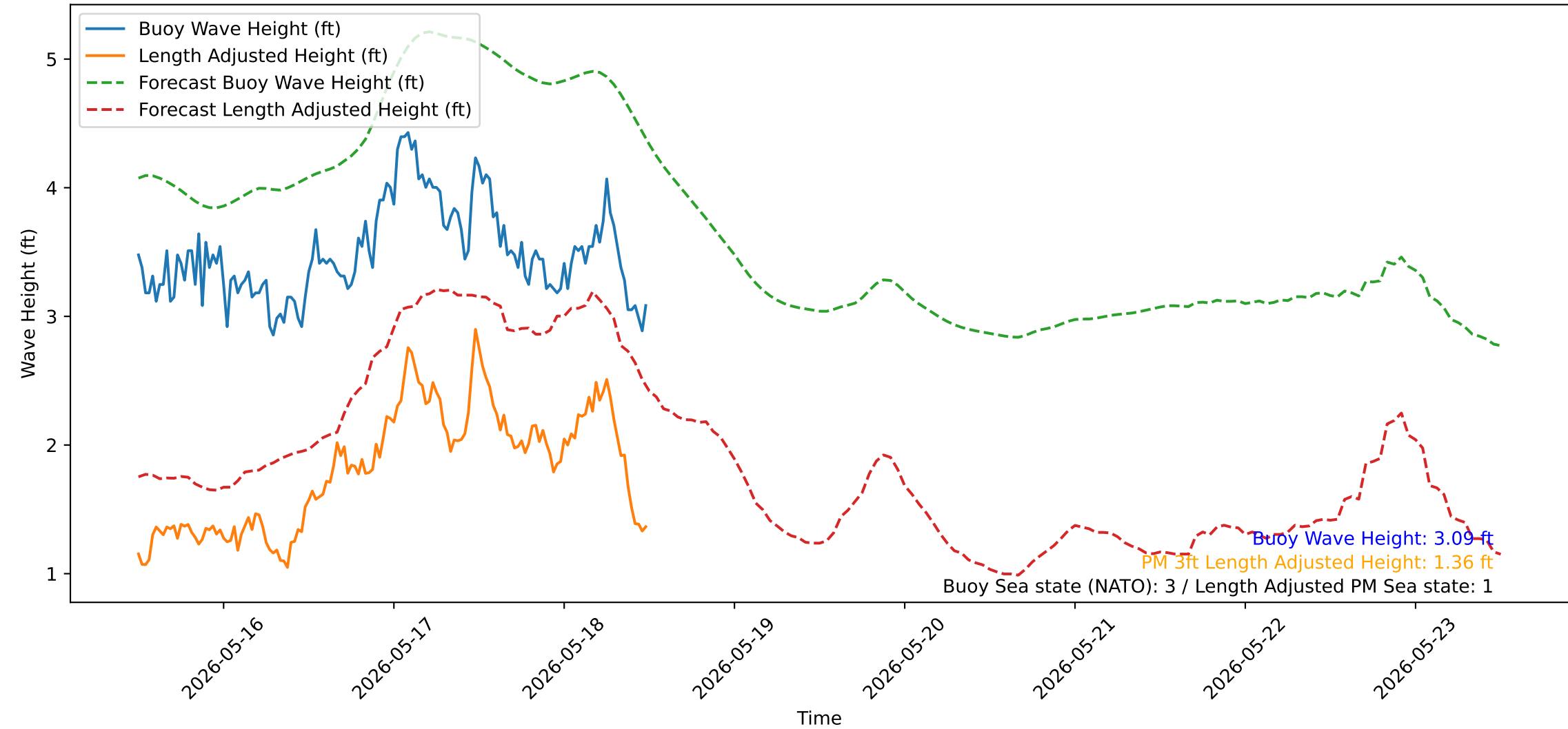
Wave Heights over Time for Green Beach at 2026-05-18 12:11:13
