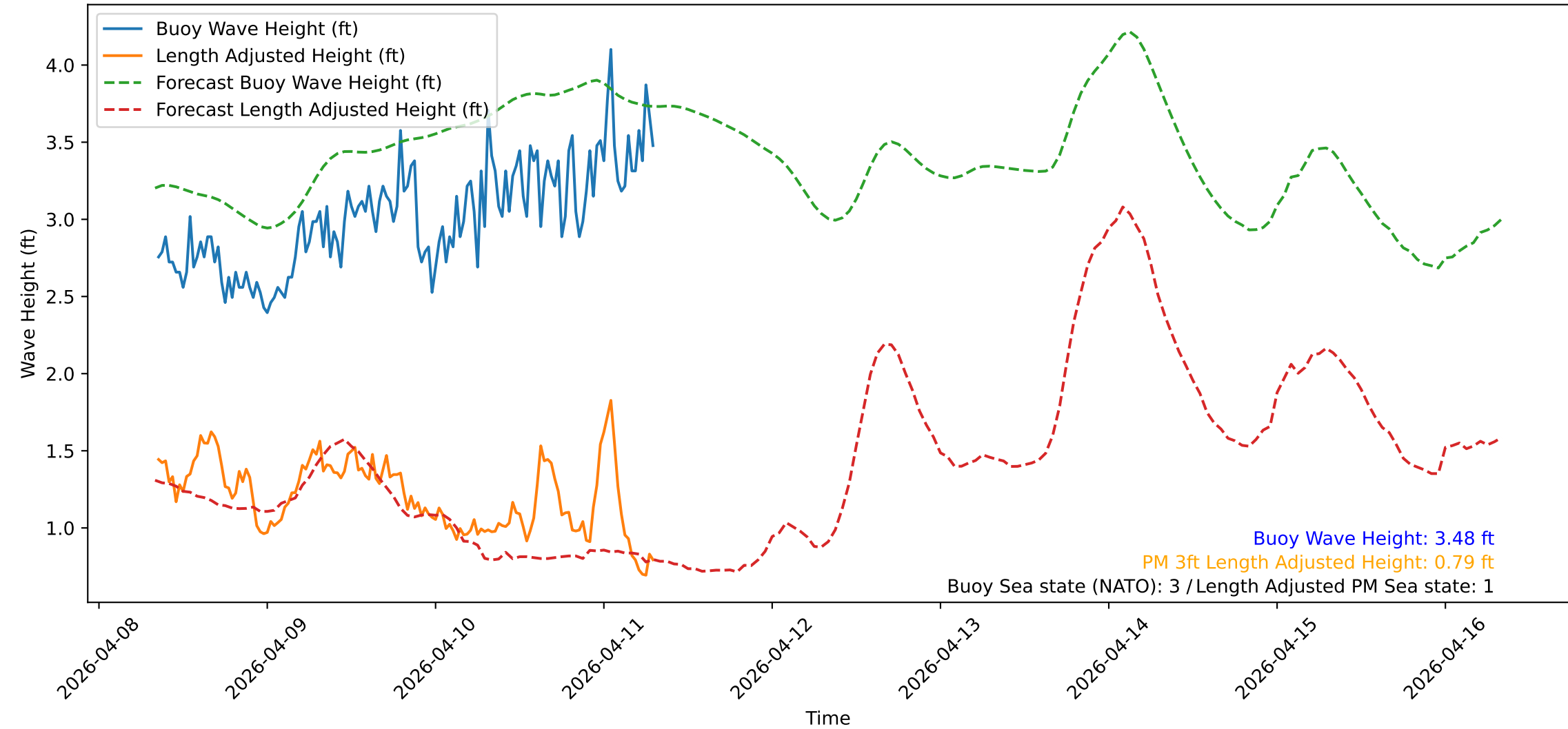
Wave Heights over Time for Red Beach at 2026-04-11 08:10:50
