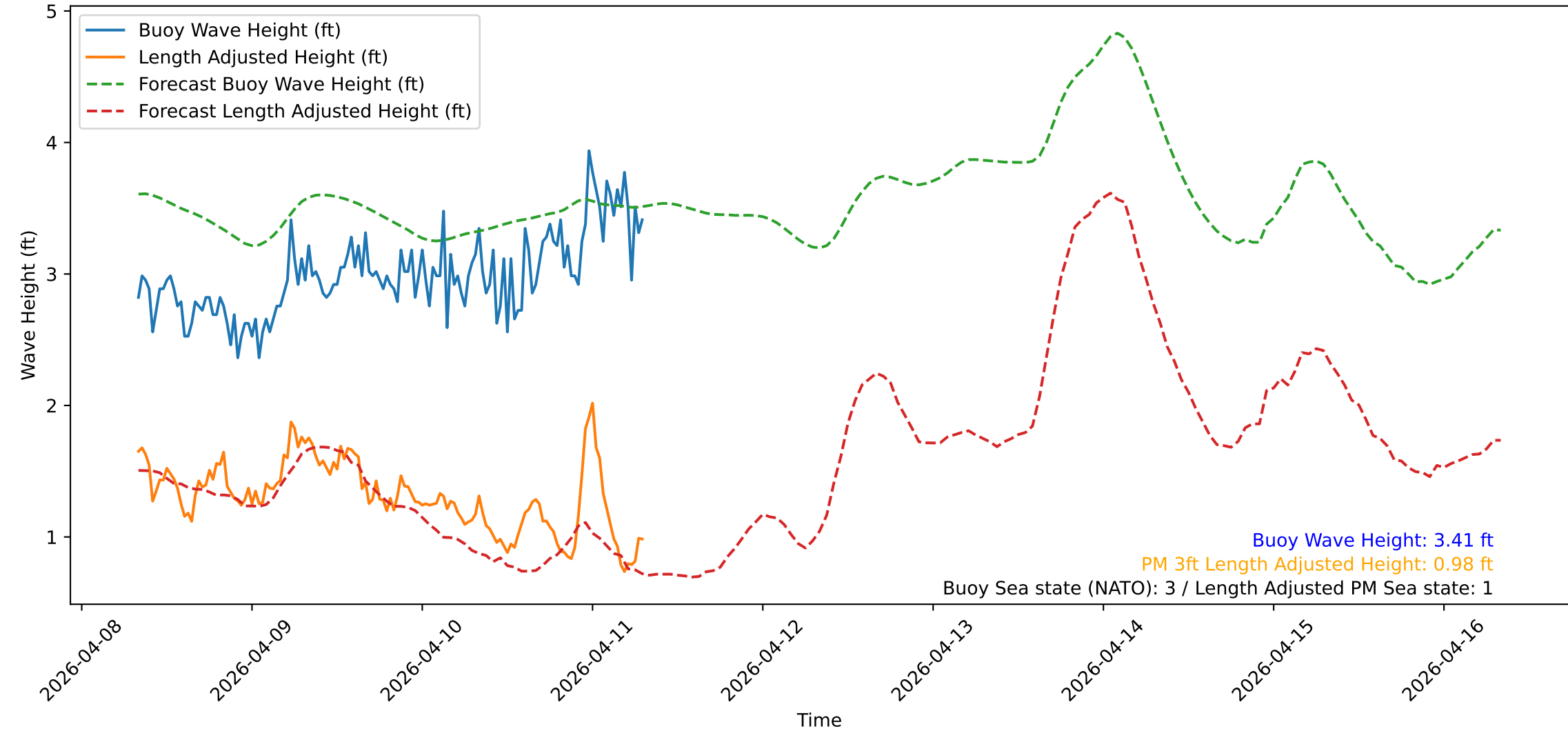
Wave Heights over Time for Green Beach at 2026-04-11 08:11:13
