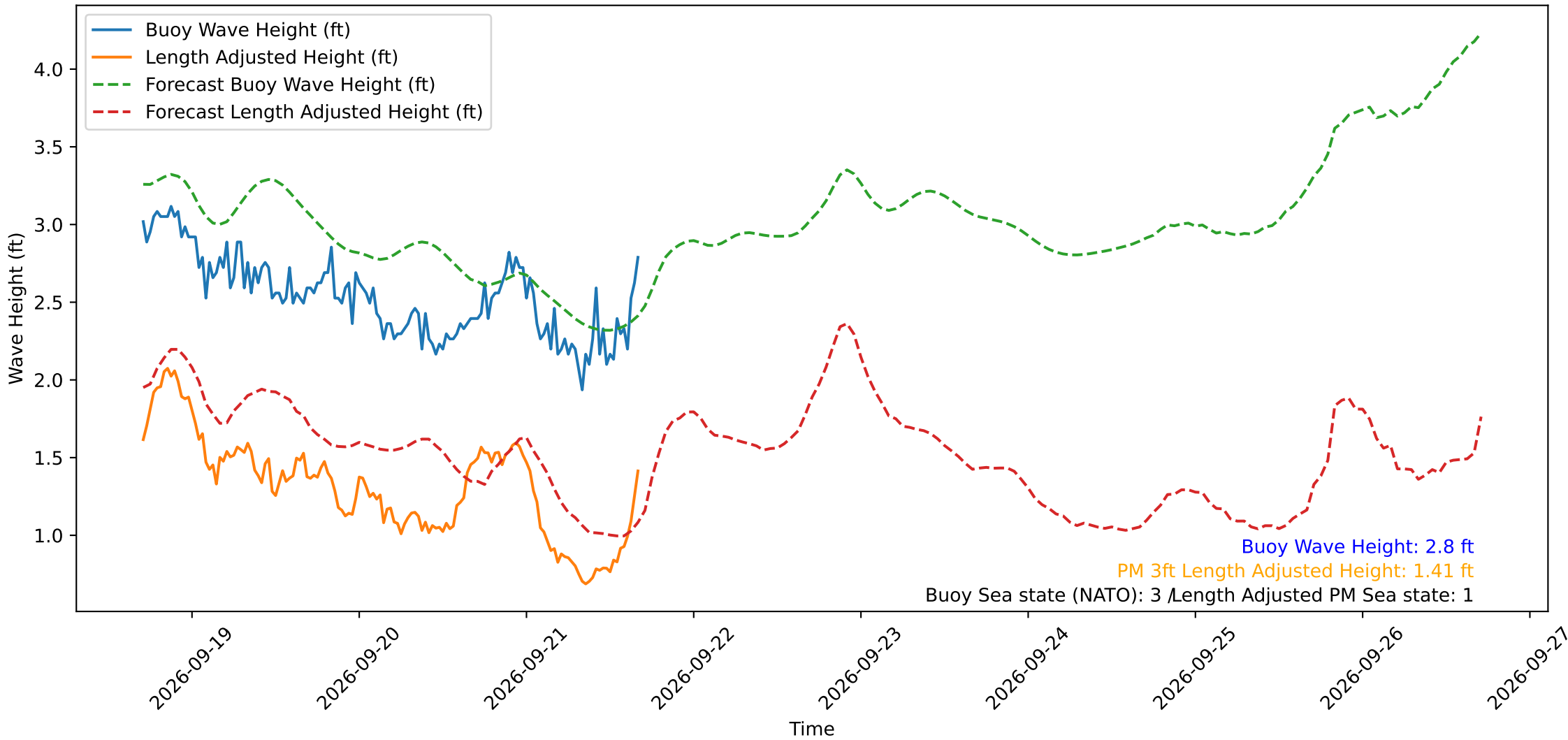
Wave Heights over Time for Green Beach at 2026-09-21 16:41:11
