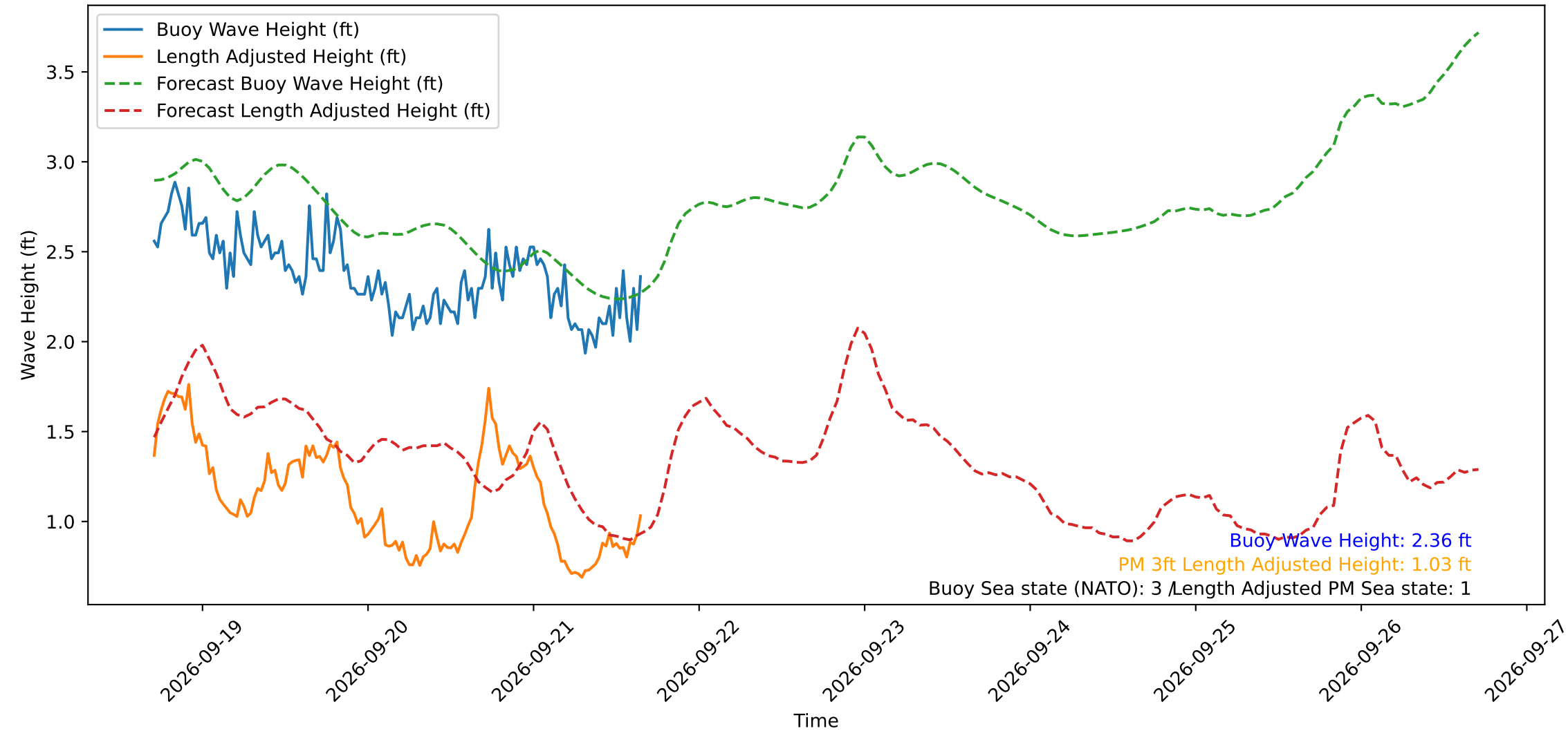
Wave Heights over Time for Red Beach at 2026-09-21 16:40:48
