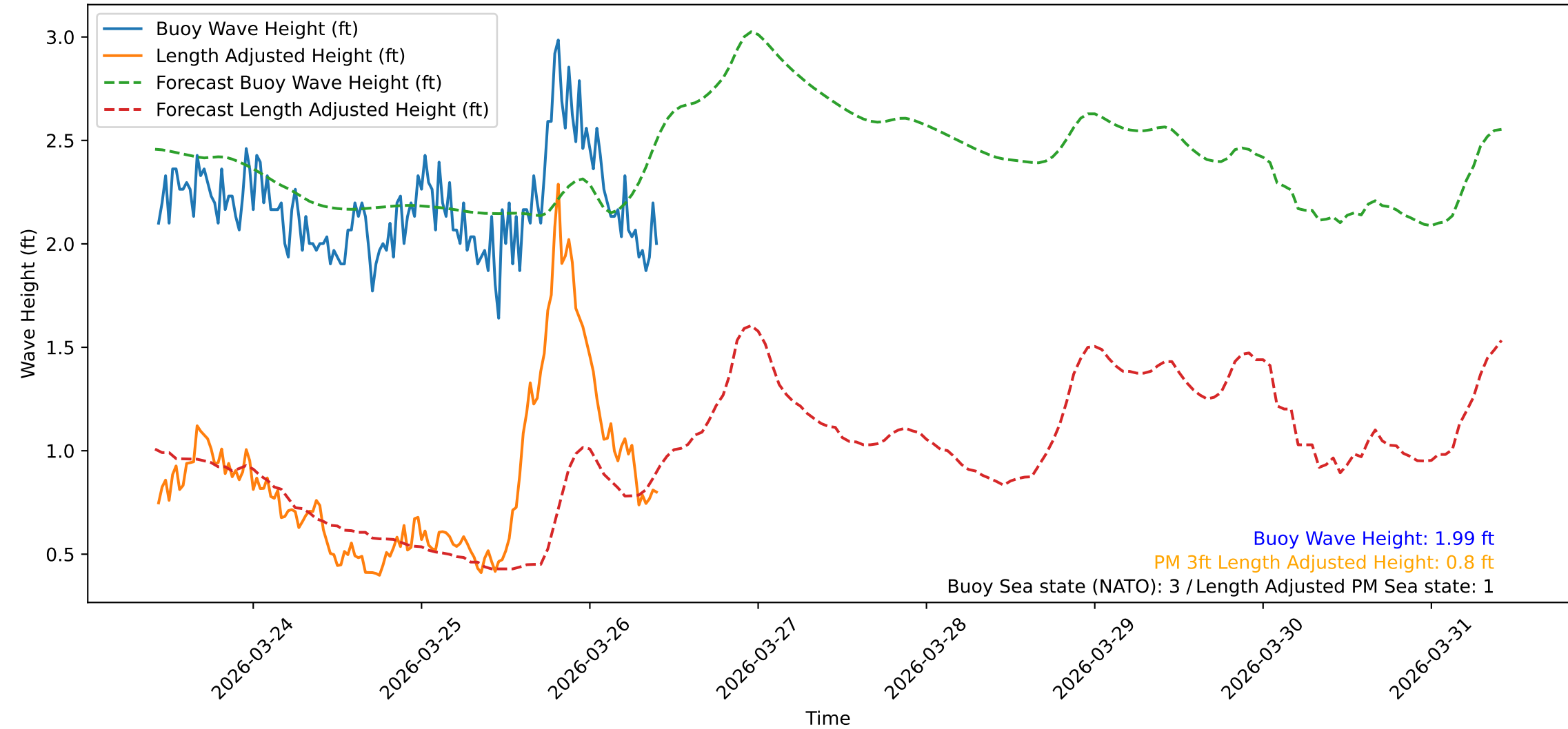
Wave Heights over Time for Green Beach at 2026-03-26 10:21:09
