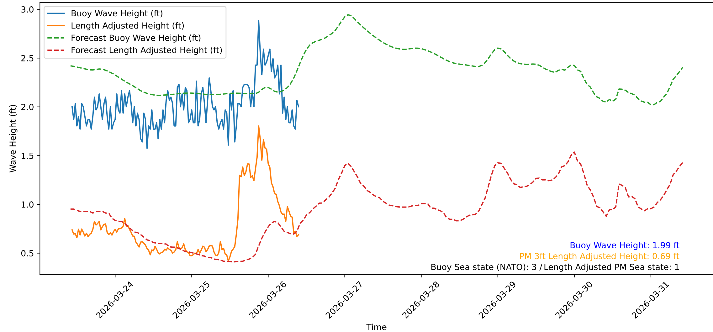
Wave Heights over Time for Oceanside Harbor at 2026-03-26 10:20:31
