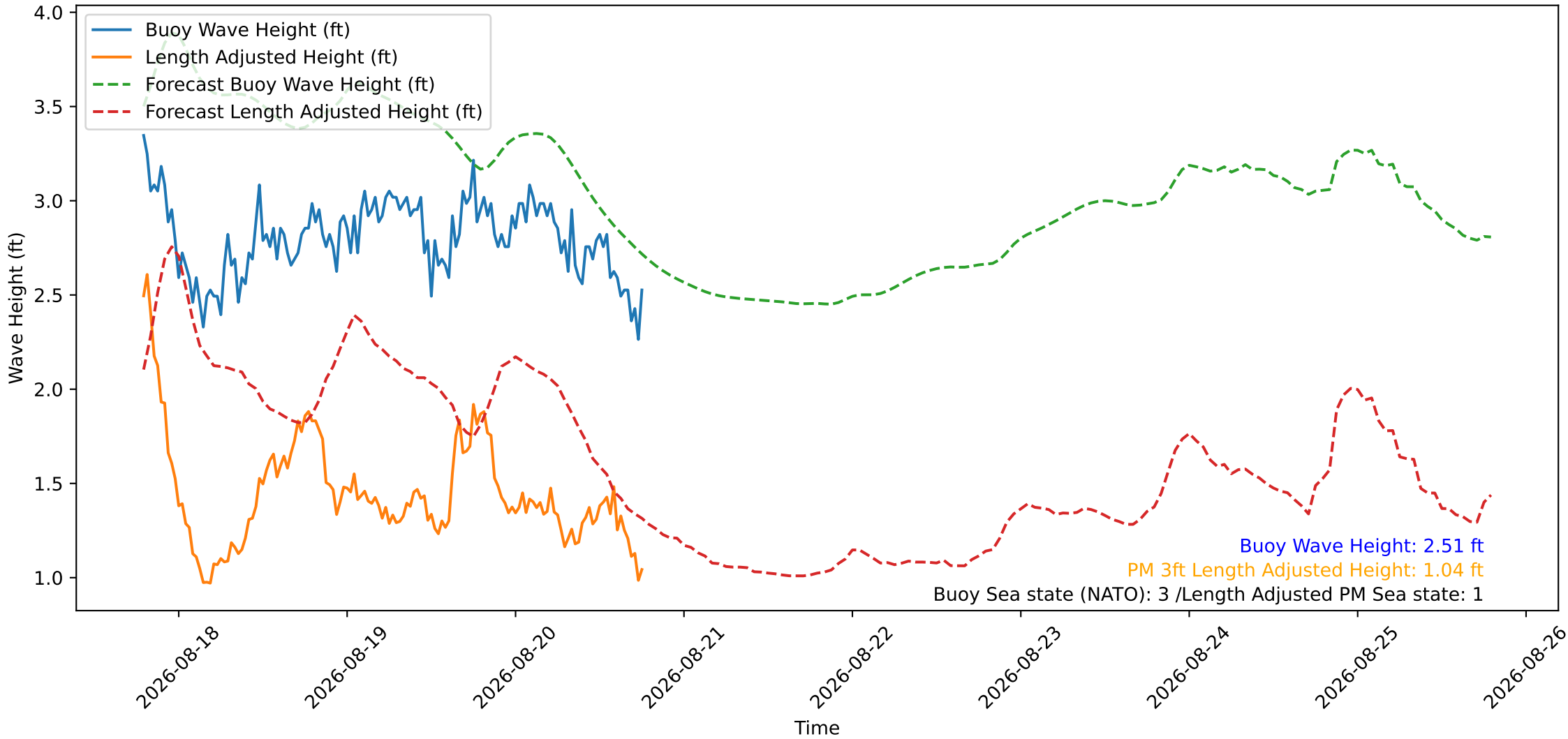
Wave Heights over Time for Red Beach at 2026-08-20 18:50:47
