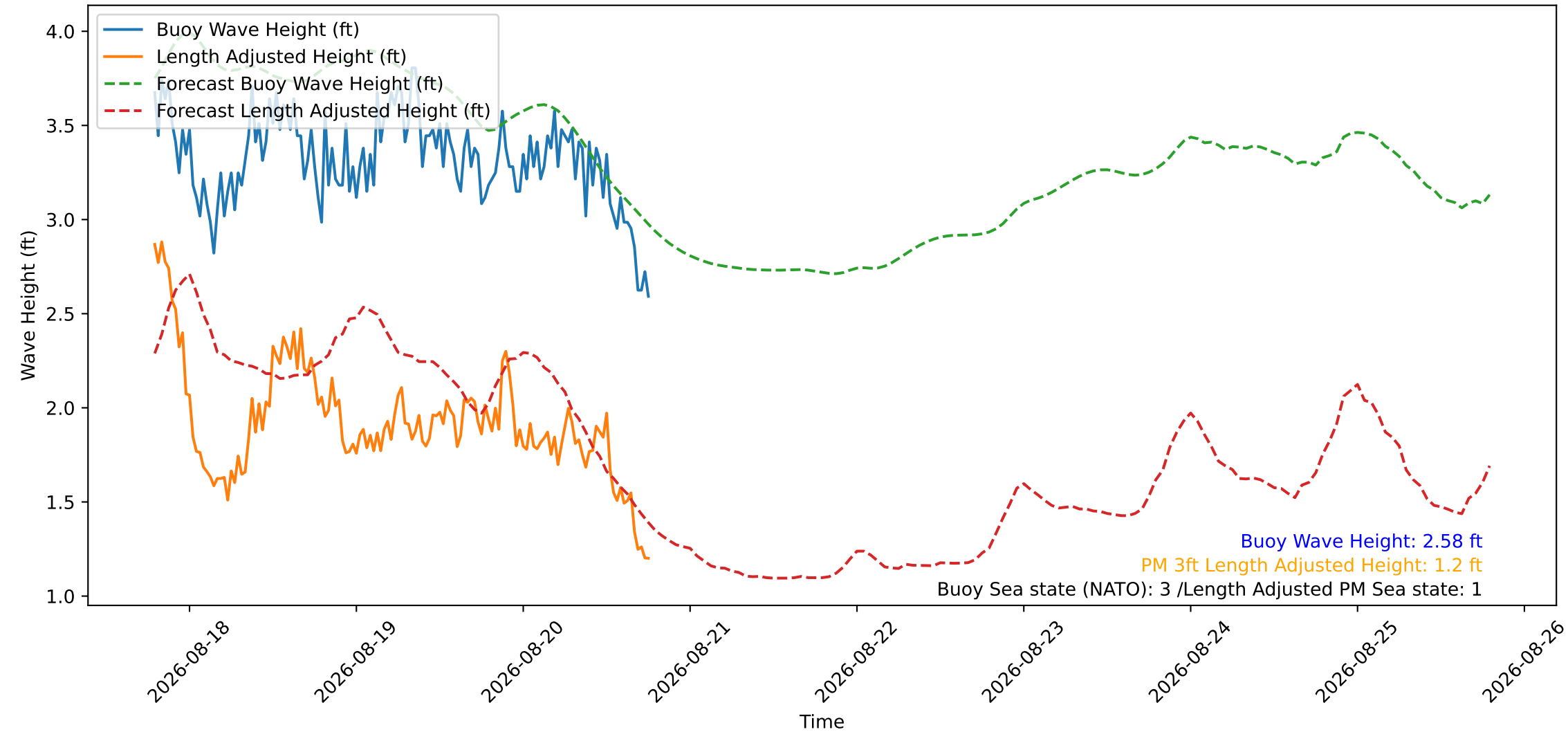
Wave Heights over Time for Oceanside Harbor at 2026-08-20 18:50:26
