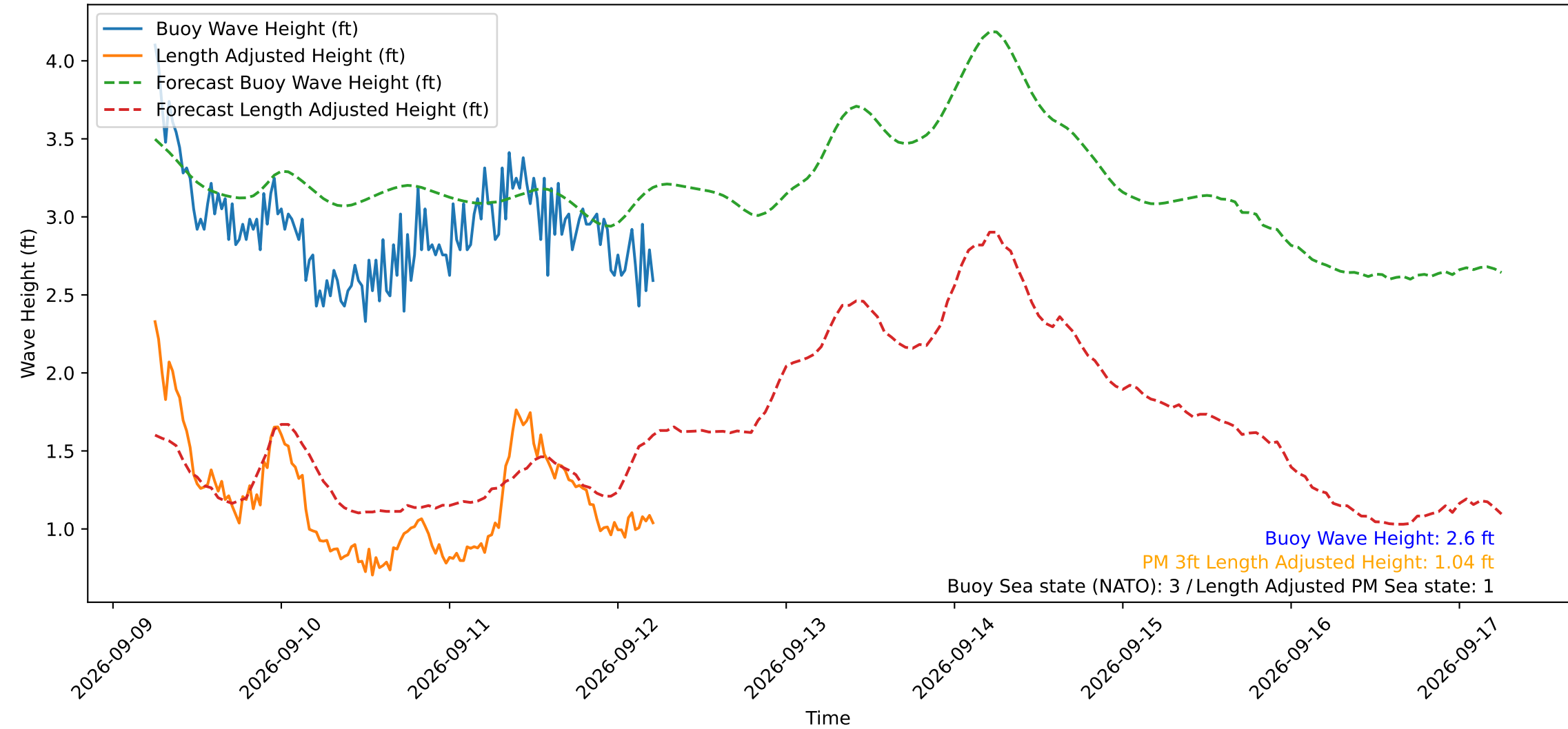
Wave Heights over Time for Red Beach at 2026-09-12 05:50:49
