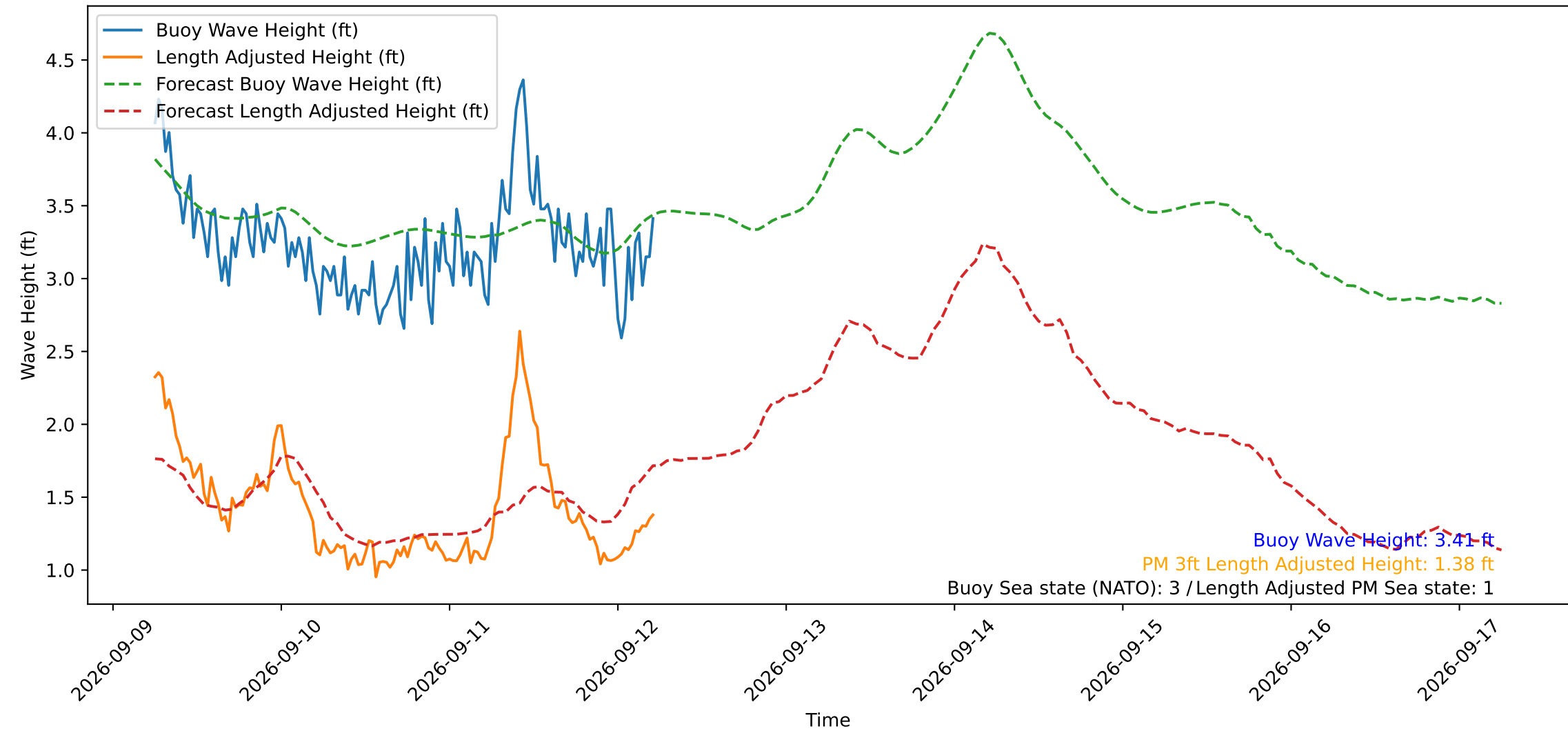
Wave Heights over Time for Oceanside Harbor at 2026-09-12 05:50:29
