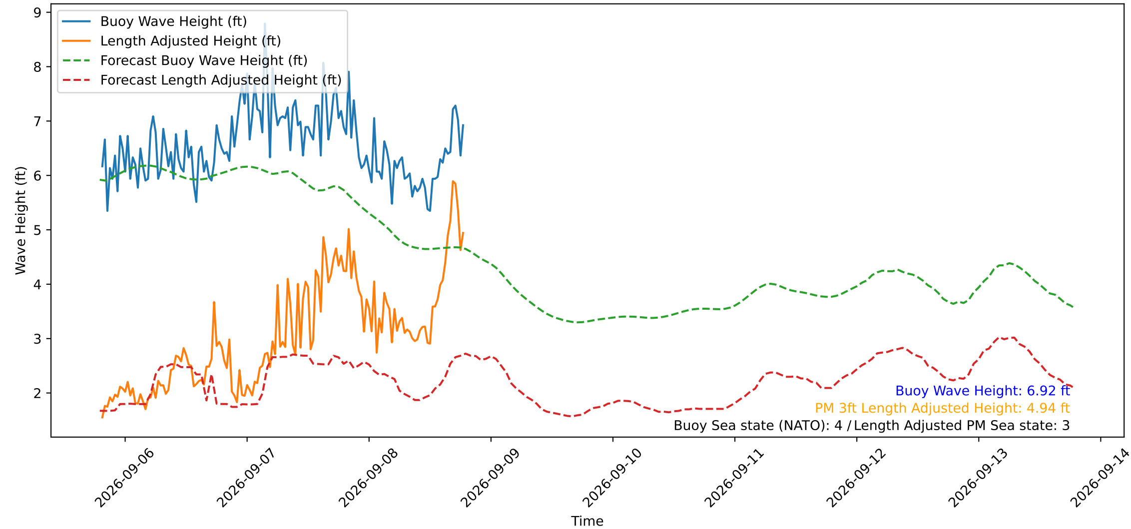
Wave Heights over Time for Green Beach at 2026-09-08 19:11:12
