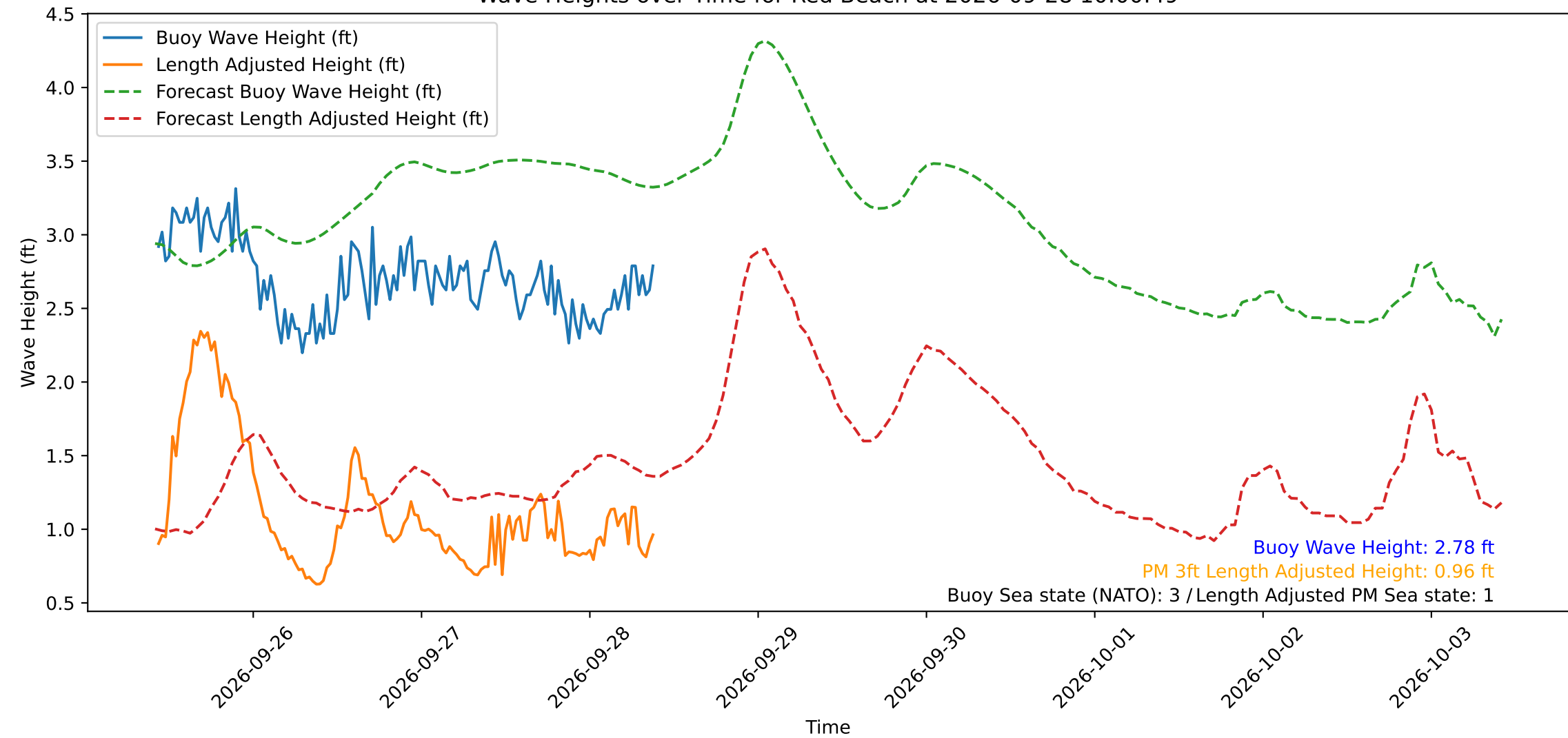
Wave Heights over Time for Red Beach at 2026-09-28 10:00:49
