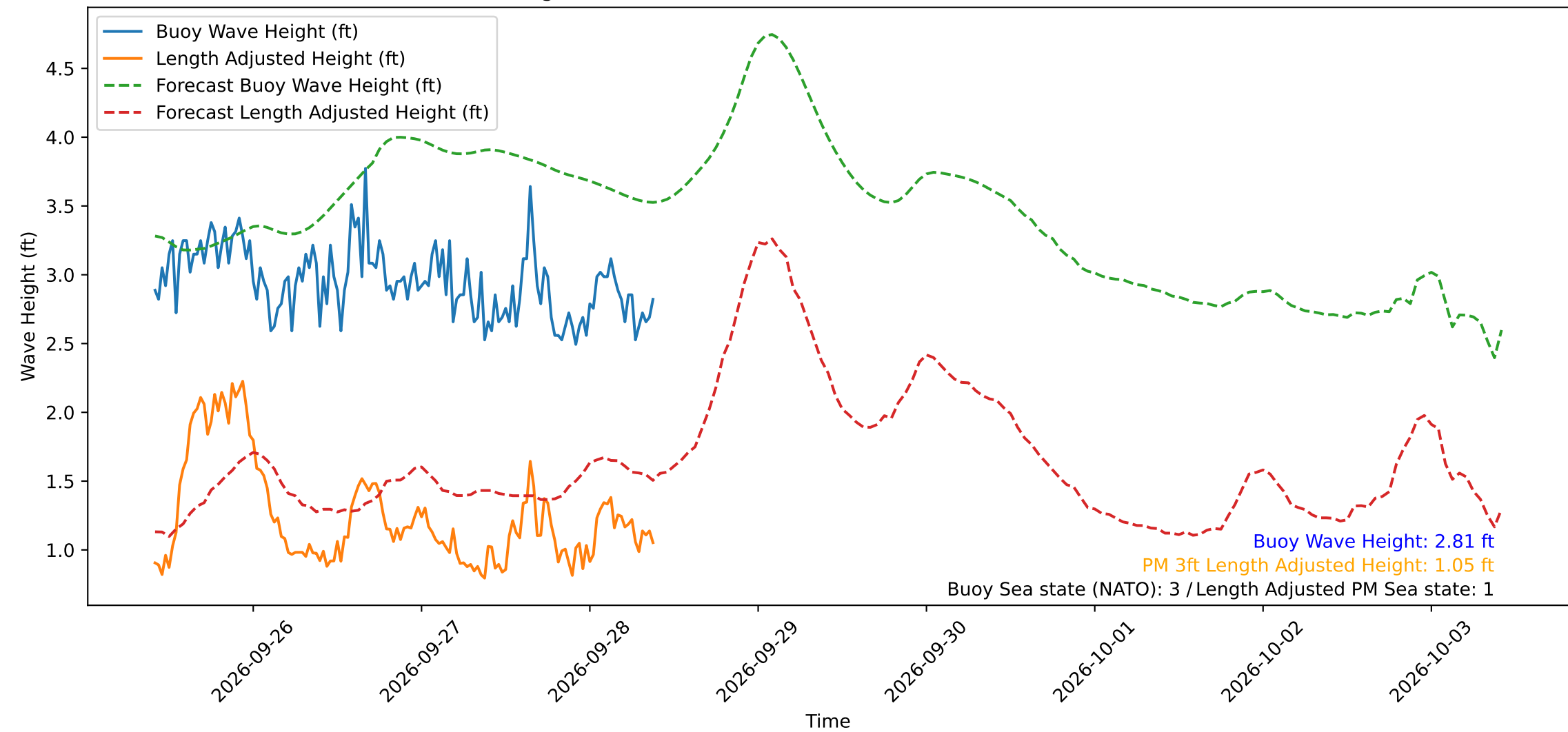
Wave Heights over Time for Oceanside Harbor at 2026-09-28 10:00:29
