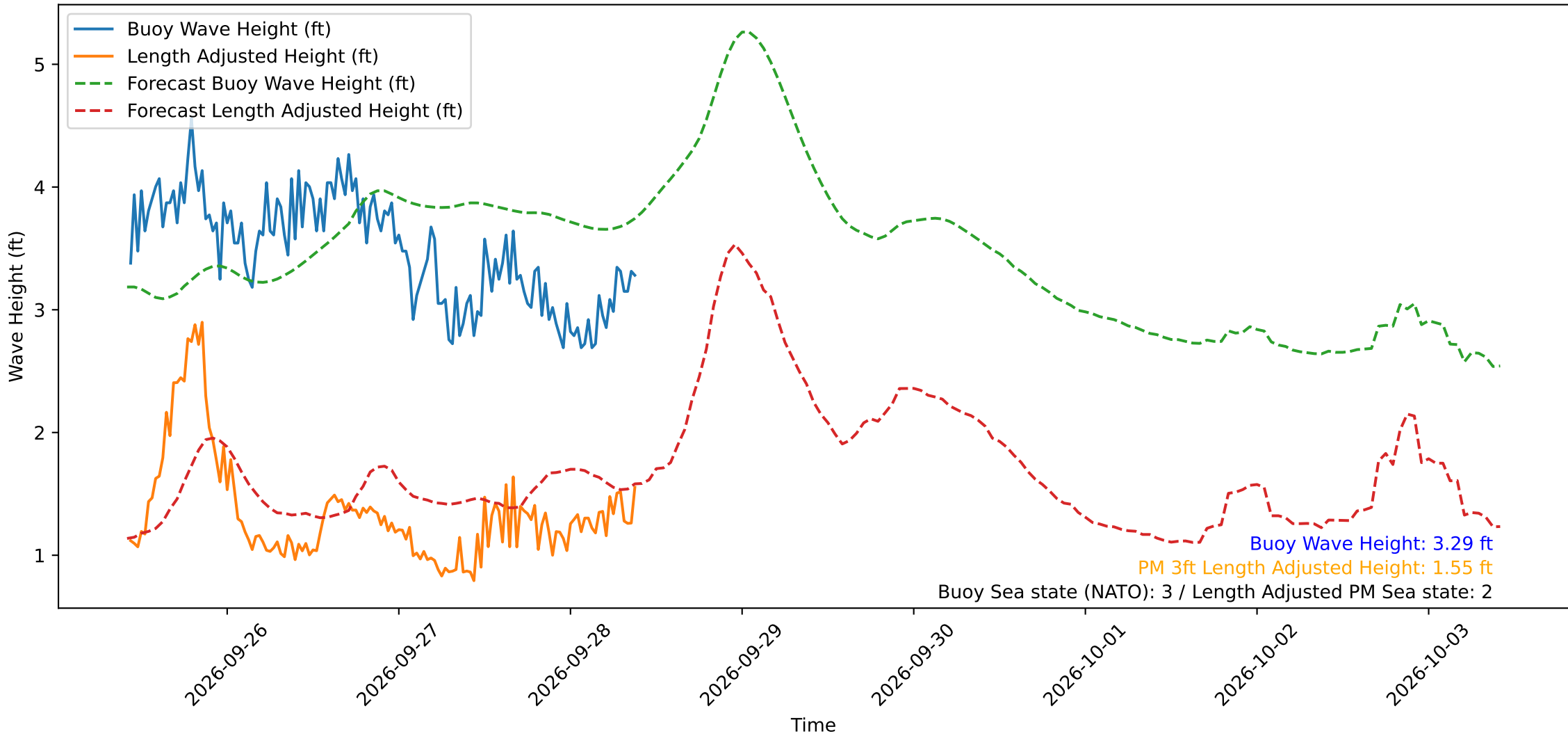
Wave Heights over Time for Green Beach at 2026-09-28 10:01:11
