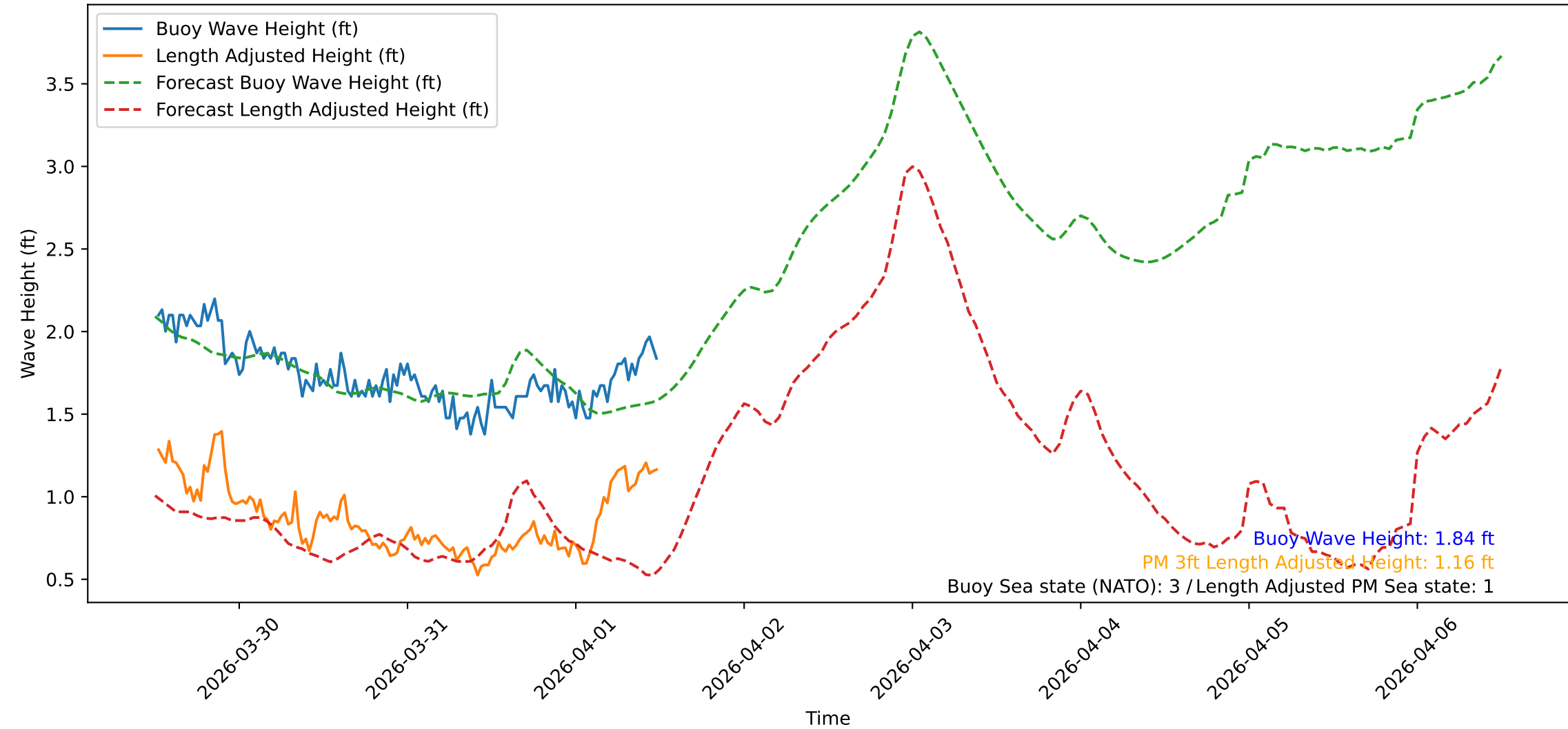
Wave Heights over Time for Red Beach at 2026-04-01 12:20:48
