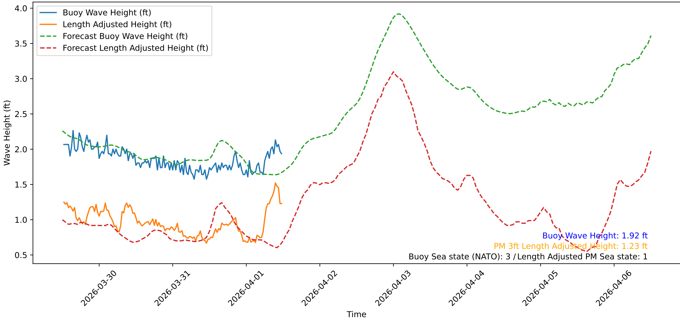
Wave Heights over Time for Oceanside Harbor at 2026-04-01 12:20:31
