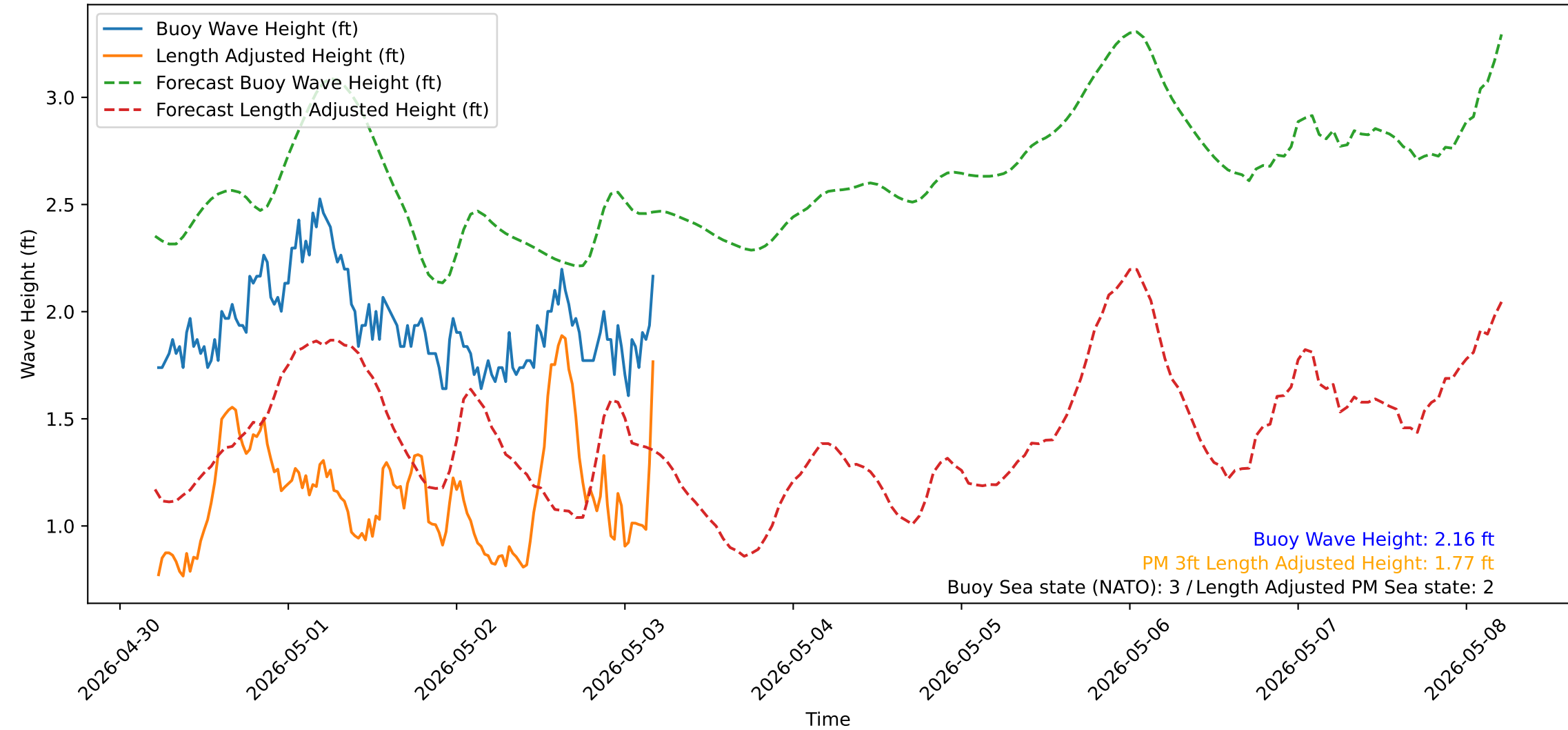
Wave Heights over Time for Red Beach at 2026-05-03 05:00:50
