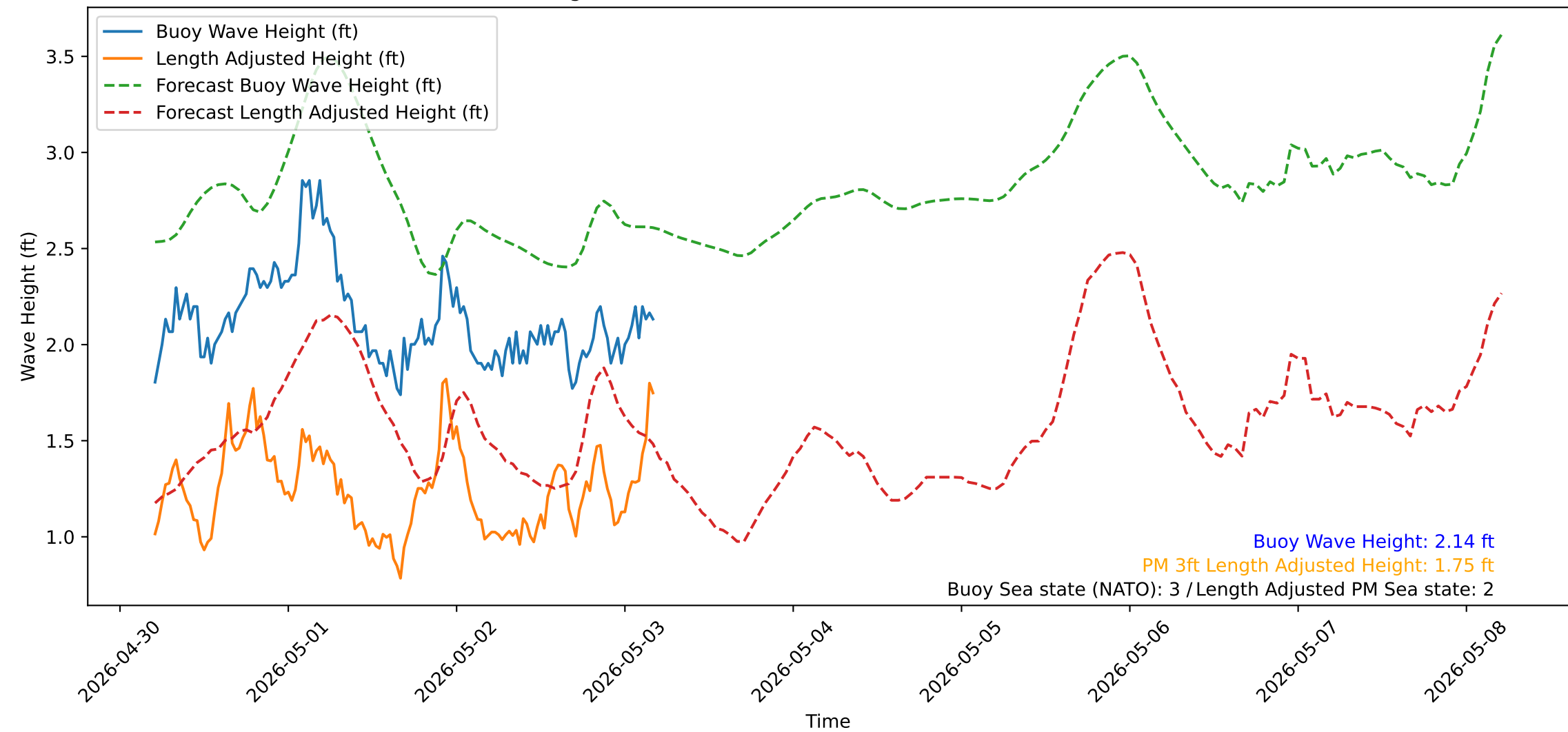
Wave Heights over Time for Green Beach at 2026-05-03 05:01:12
