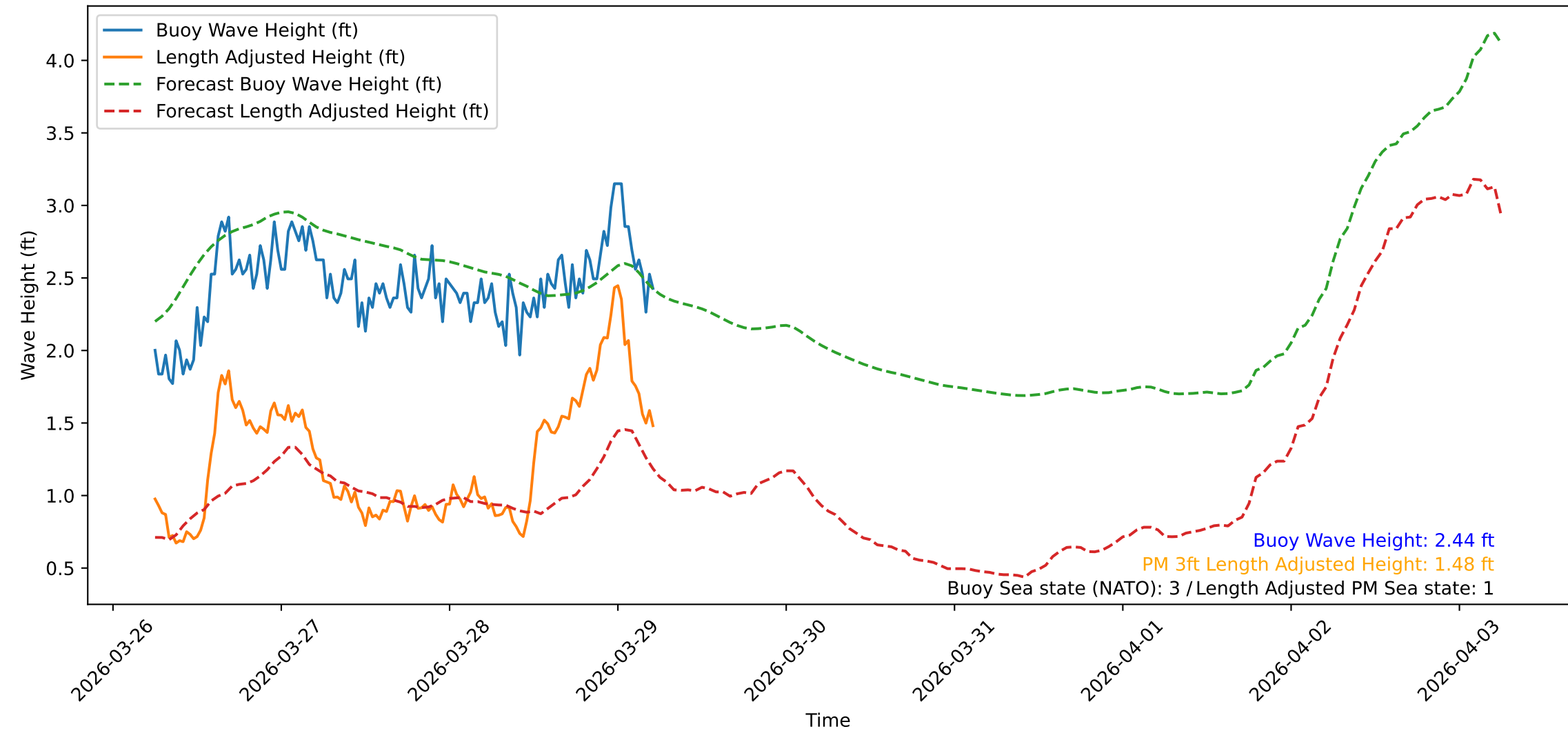
Wave Heights over Time for Oceanside Harbor at 2026-03-29 05:50:31
