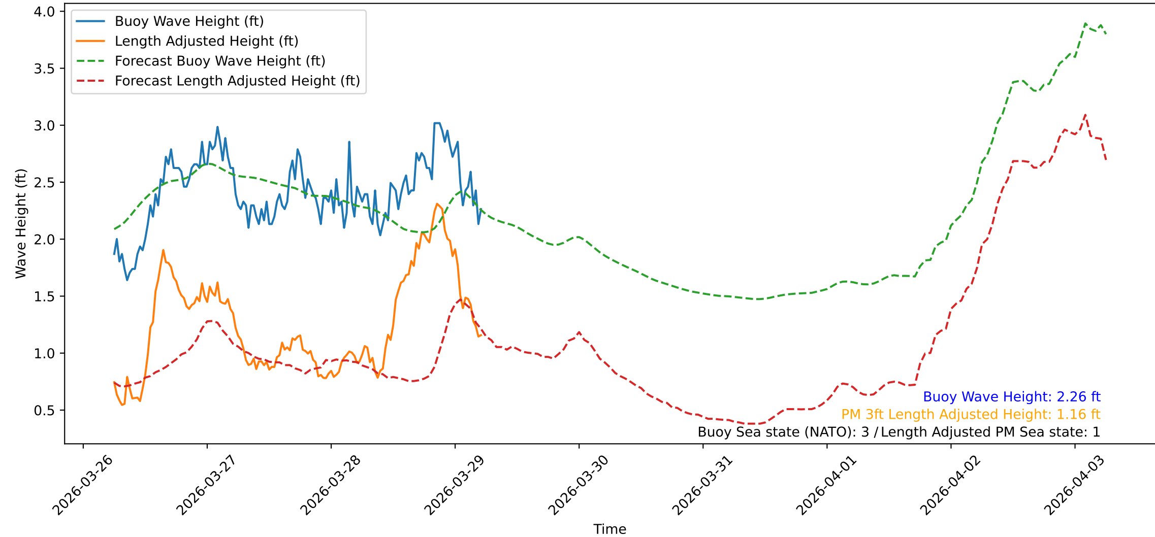
Wave Heights over Time for Red Beach at 2026-03-29 05:50:47
