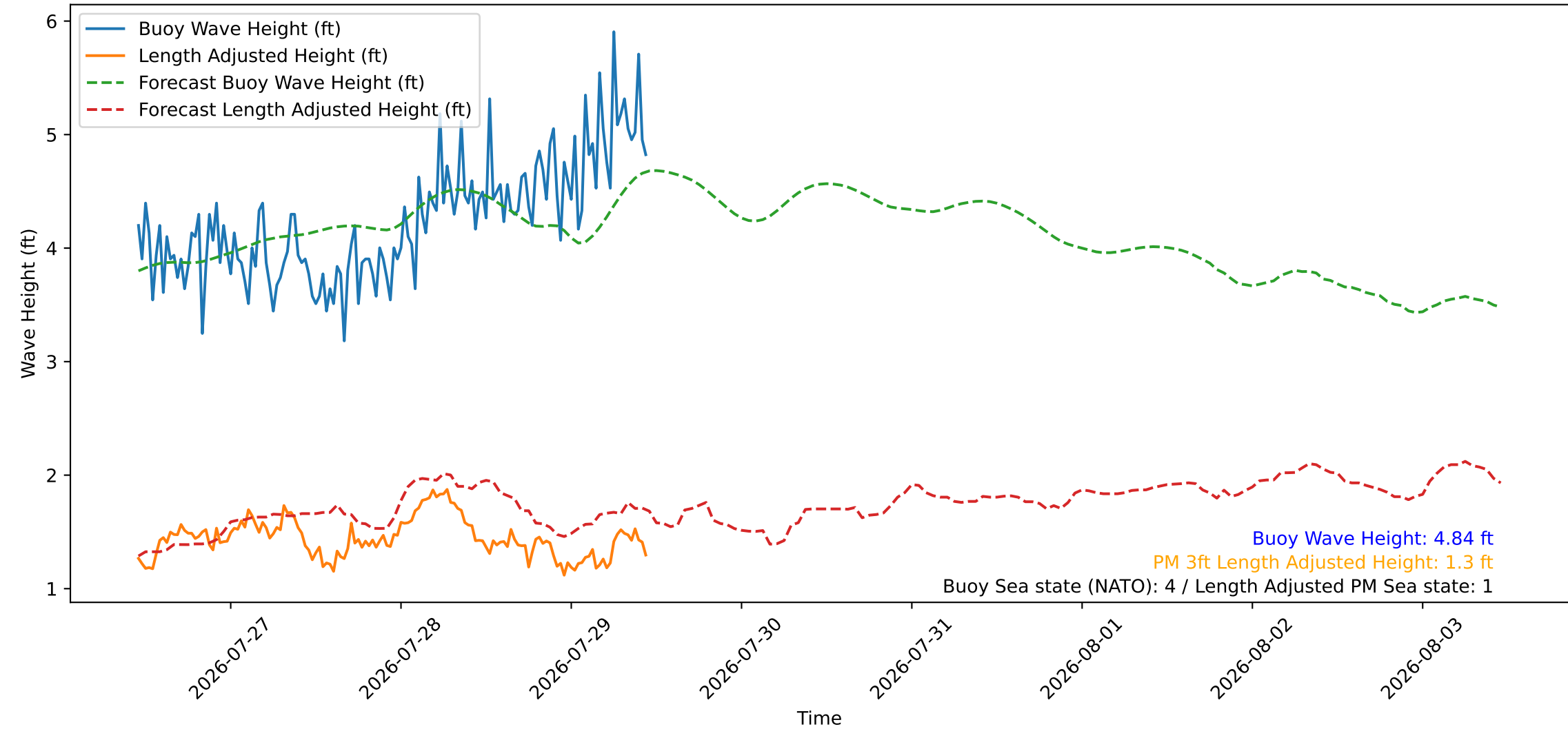
Wave Heights over Time for Oceanside Harbor at 2026-07-29 11:10:26
