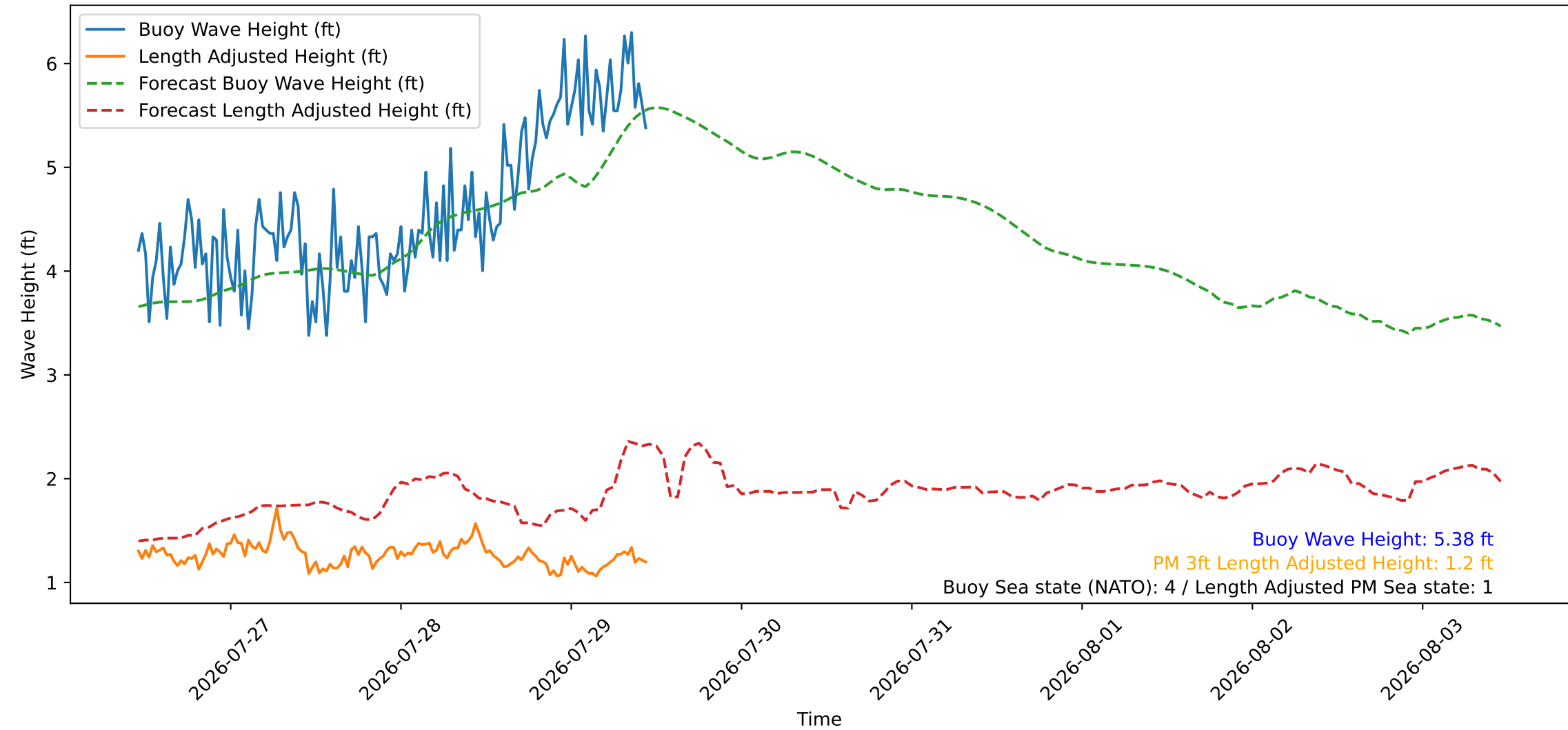
Wave Heights over Time for Green Beach at 2026-07-29 11:11:08
