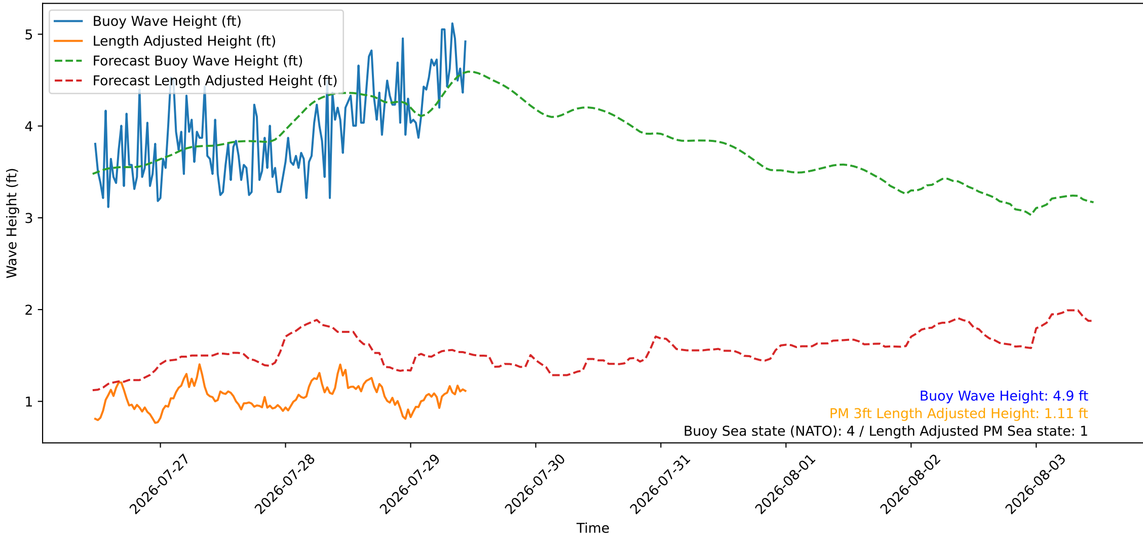
Wave Heights over Time for Red Beach at 2026-07-29 11:10:45
